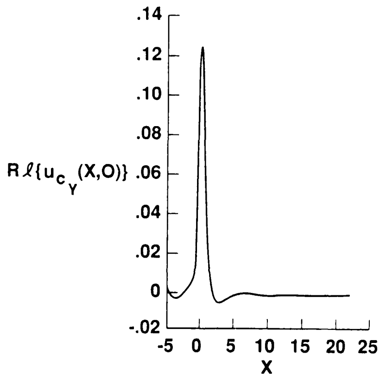
Figure 12b. Disturbance wall shear for the combined receptivity problem ( u_c ) for S_0 = 3.0 , V_w = -0.10 .
