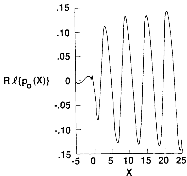
Figure 6a. Disturbance pressure for S_o = 2.5 , V_w = -0.25 .
