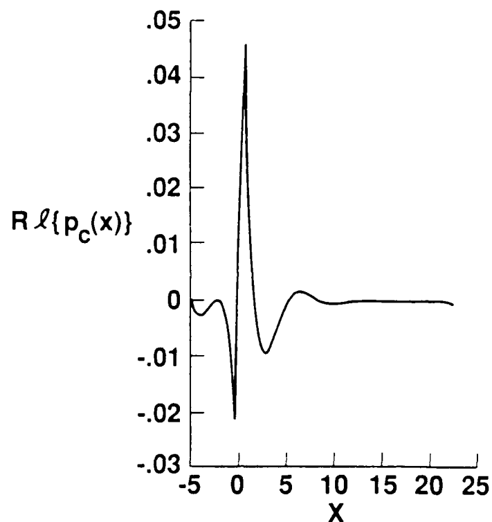
Figure 12a. Disturbance pressure for the combined receptivity problem ( u_c ) for S_0 = 3.0 , V_w = -0.10 .
