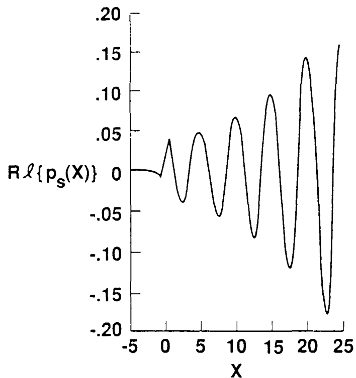
Figure 11a. Disturbance pressure for the suction receptivity problem ( u_s ) for S_0 = 3.0 , V_w = -0.10 .
