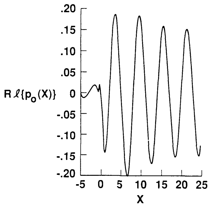
Figure 7a. Disturbance pressure for S_o = 2.5 , V_w = -0.50 .
