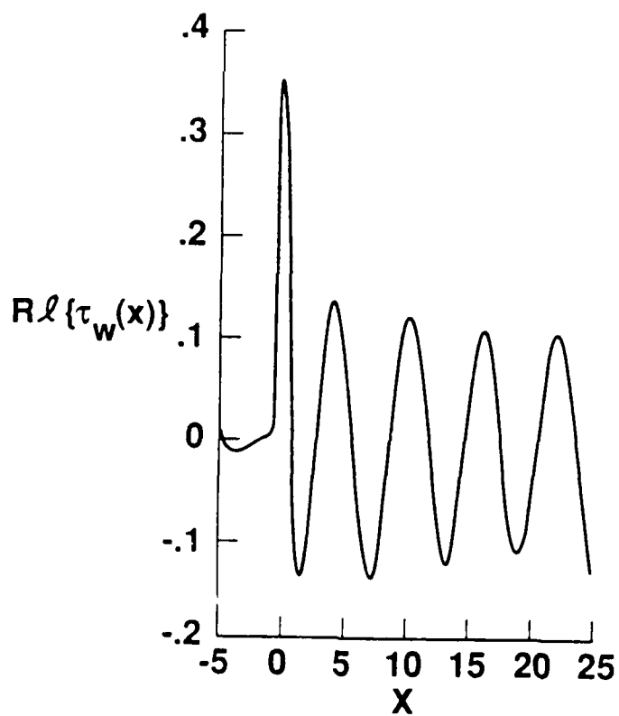
Figure 7b. Disturbance wall shear for S_o = 2.5 , V_w = -0.50 .
