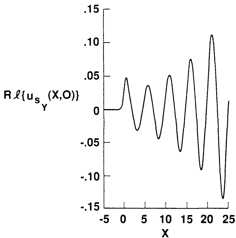
Figure 11b. Disturbance wall shear for the suction receptivity problem ( u_s ) for S_0 = 3.0 , V_w = -0.10 .
