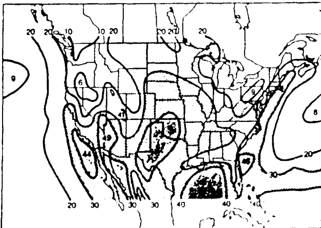
PROBABILITY OF CLEAR SKY IN WINTER
