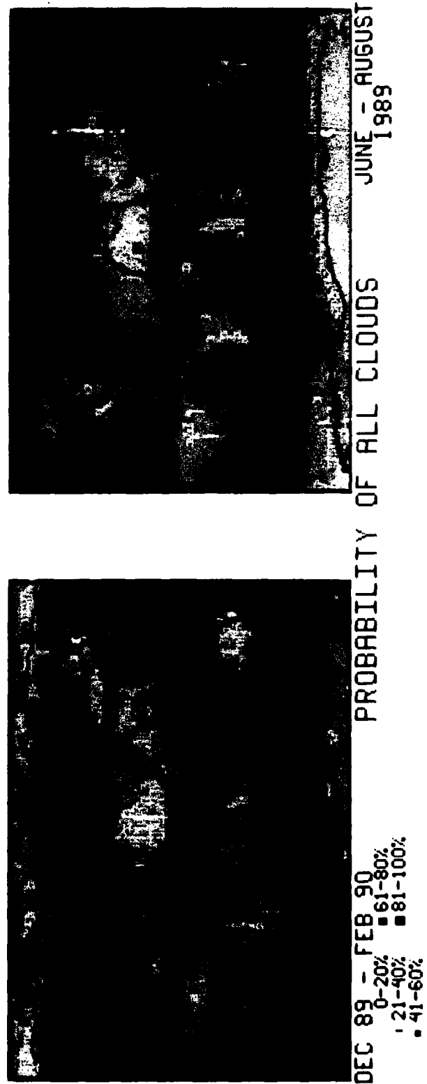
Figure 10: The probability of transmissive cirrus (upper panels) and all cloud forms including cirrus (lower panels) from NOAA/HIRS data.
