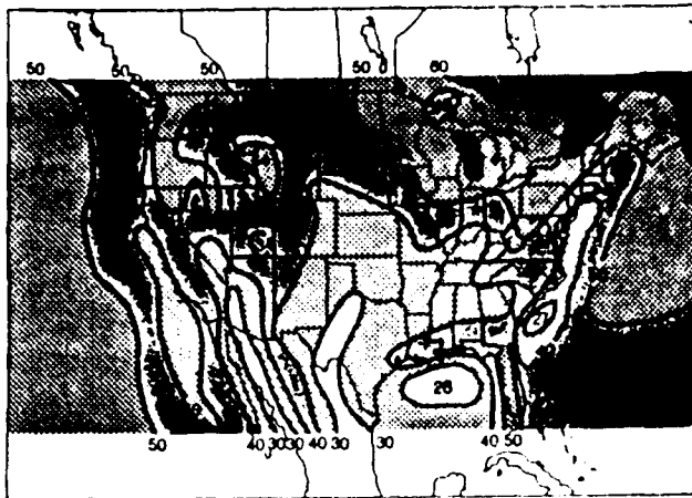
PROBABILITY OF OPAQUE CLOUD IN WINTER
