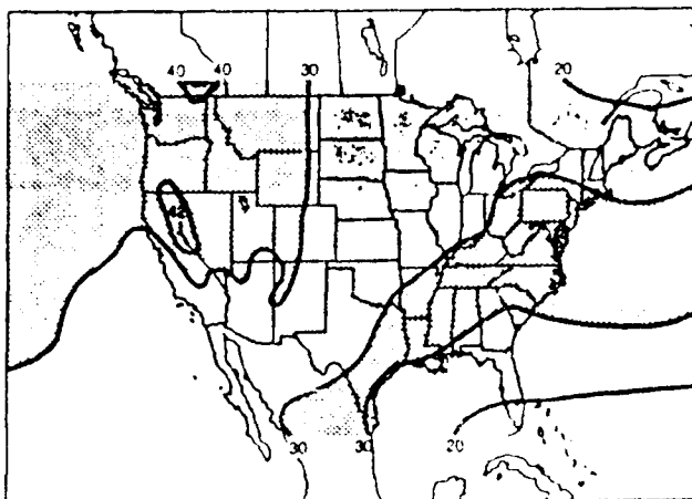
PROBABILITY OF CIRRUS IN WINTER
