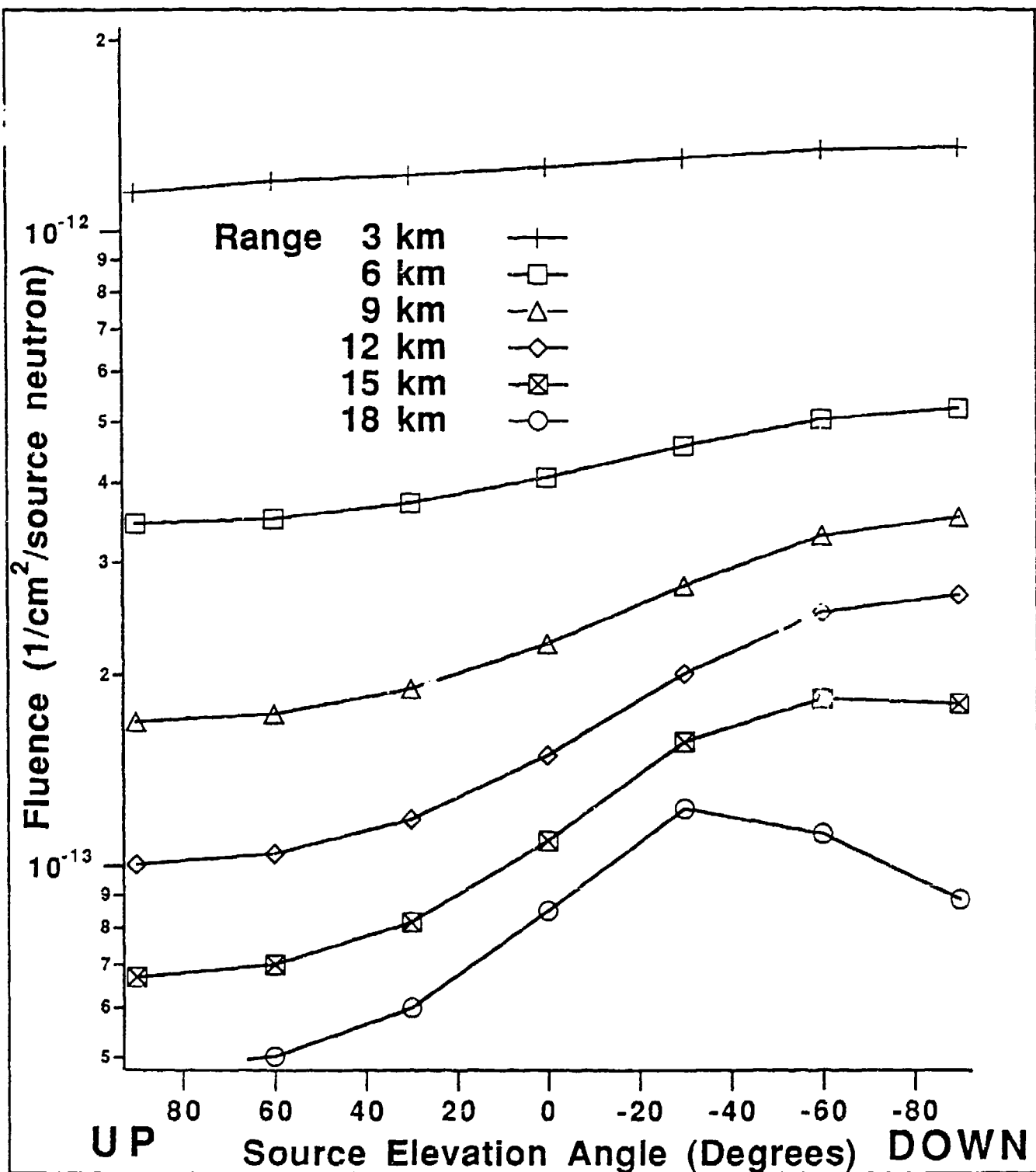
FIGURE 10 Neutron fluence calculated by SMAUG
