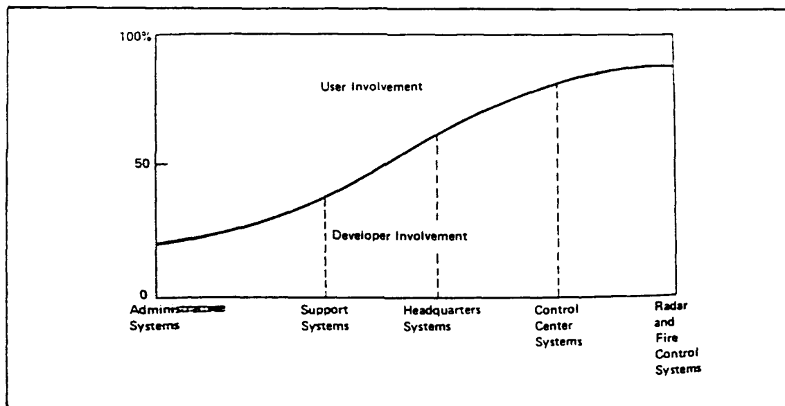
Figure 6.1 User-Developer Involvement
