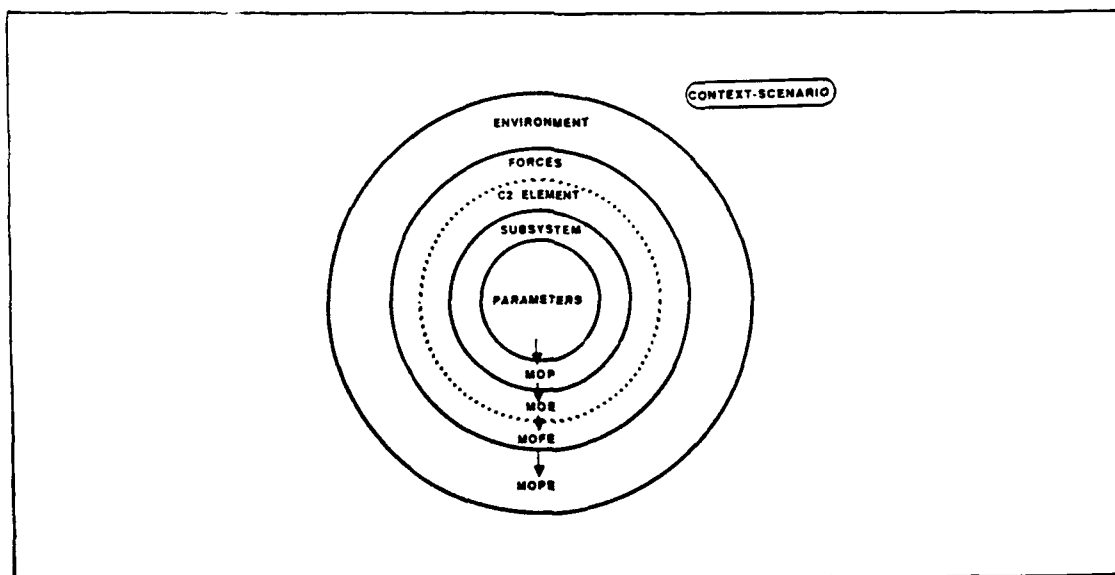
Figure 4.12 System Boundary
