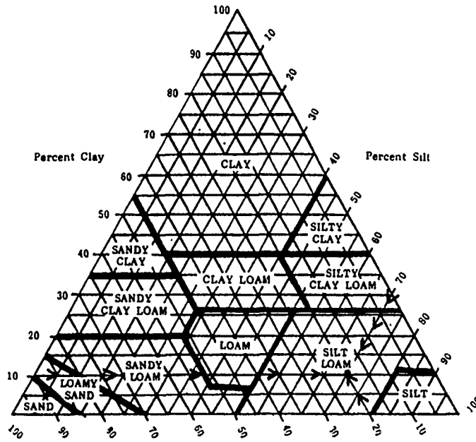
Figure E1. USDA soil textural classification.
