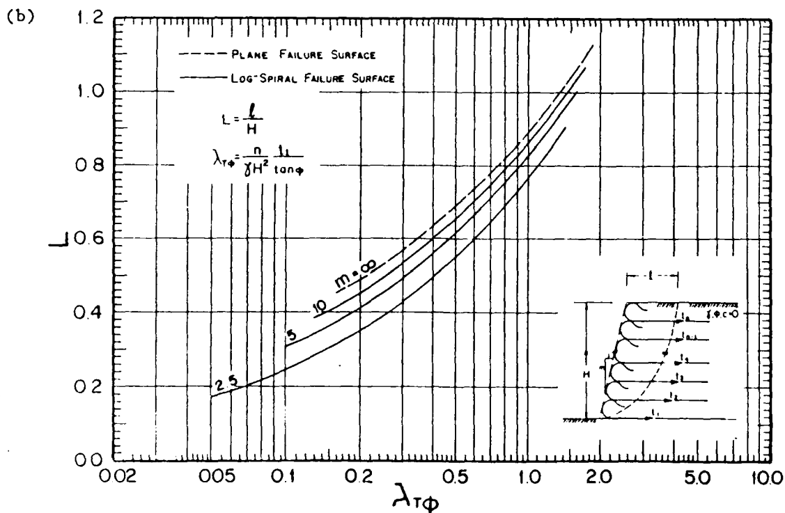
Figure 6. Design Chart.
