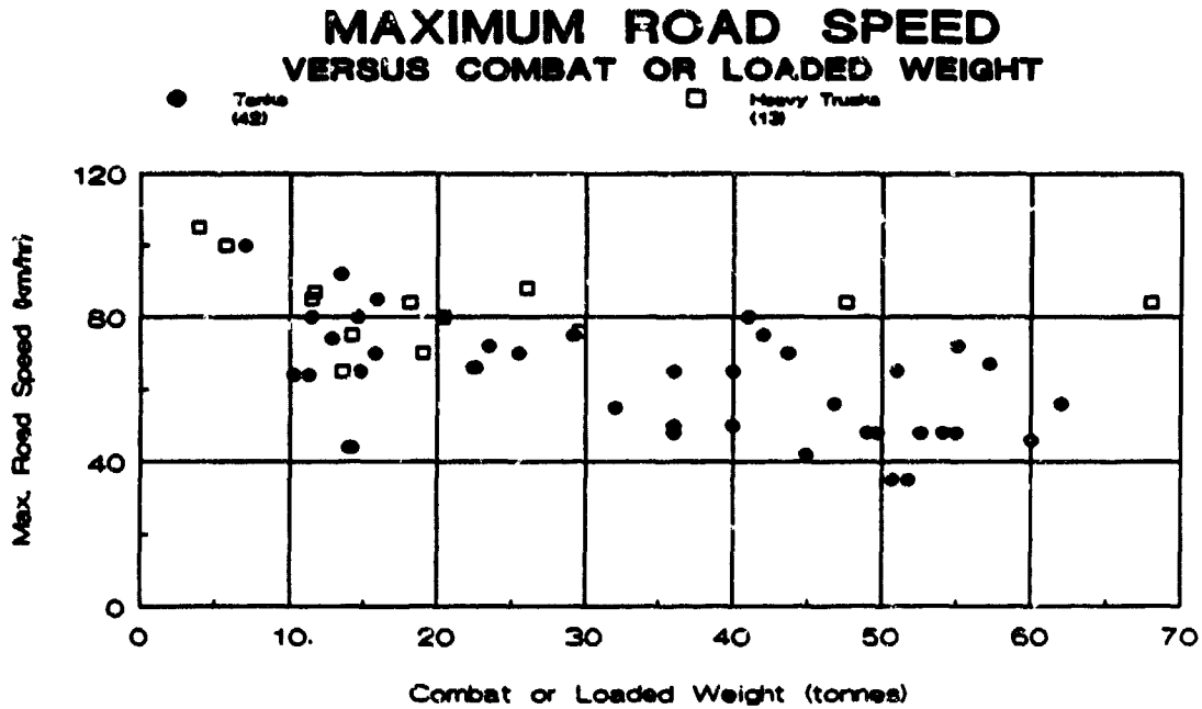
Figure 4-1. Maximum Rated Road Speeds of Tanks and Heavy Trucks
