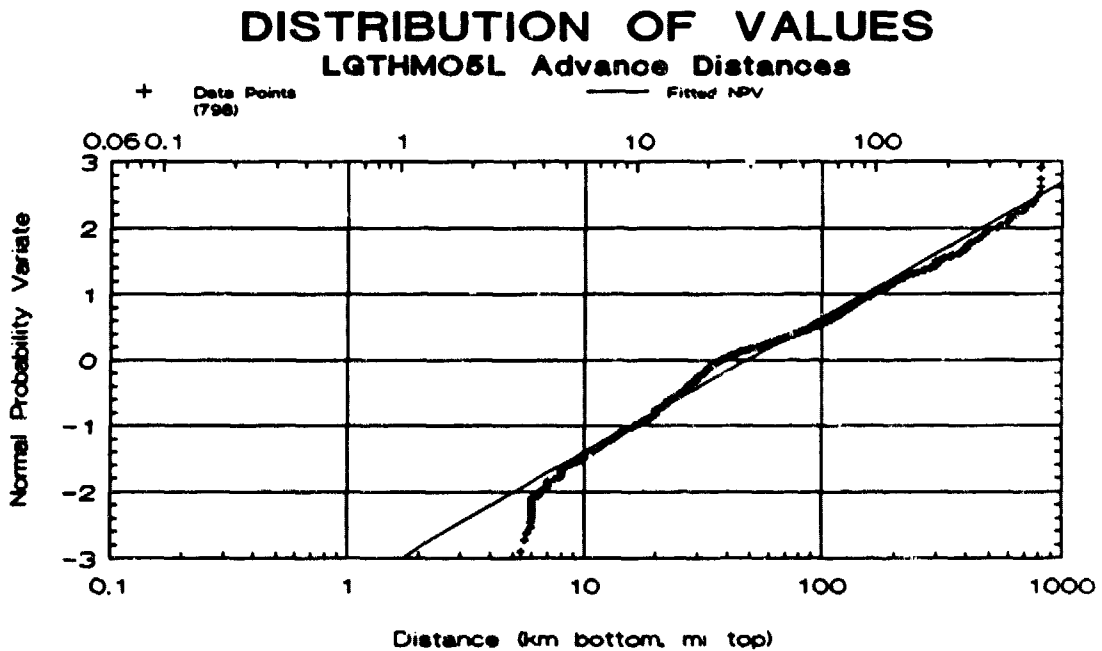
Figure 4-29d. Distribution of Total Advance Distance for LGTH05L Data
