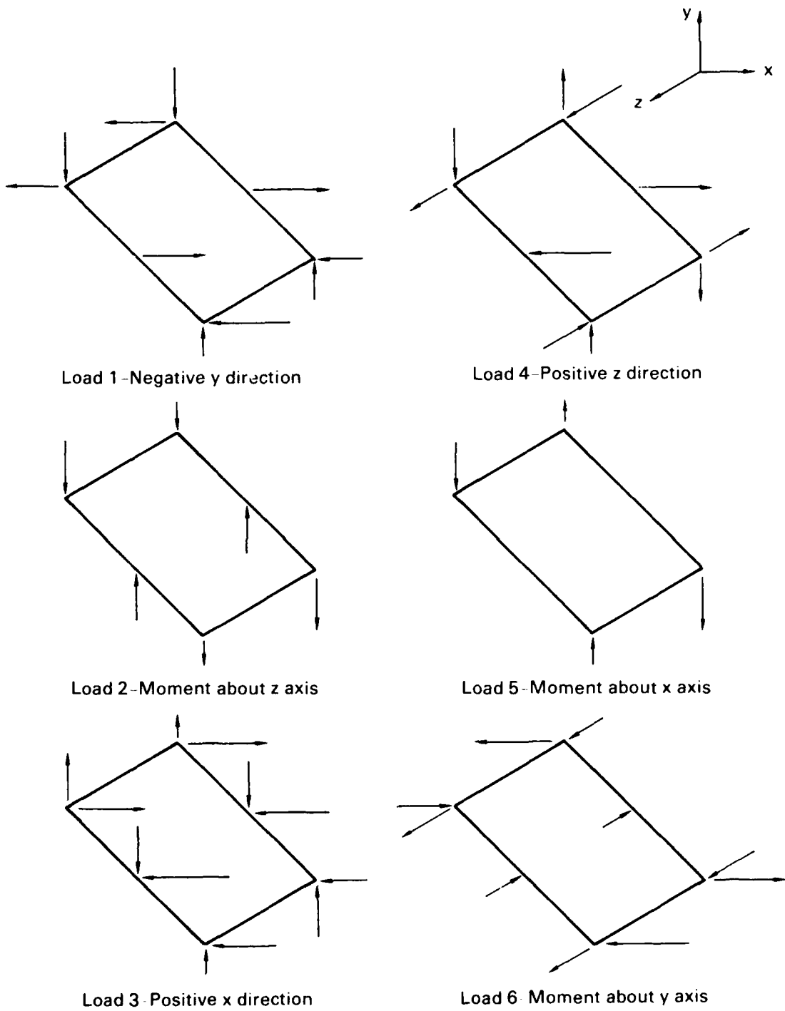
Figure 31. Summary of reaction forces.
