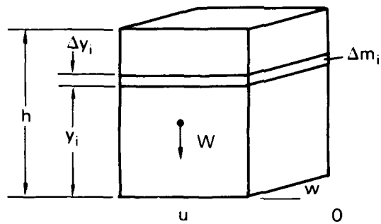
Figure 19. Uniform mass.
