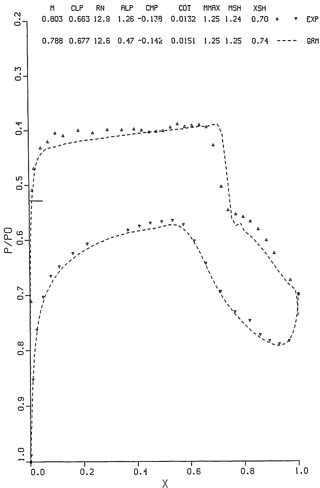
FIG. 63c: COMPARISON OF GRUMFOIL AND EXPERIMENT, TRANSITION FIXED. 10% AIRFOIL. C_L \approx 0.663
