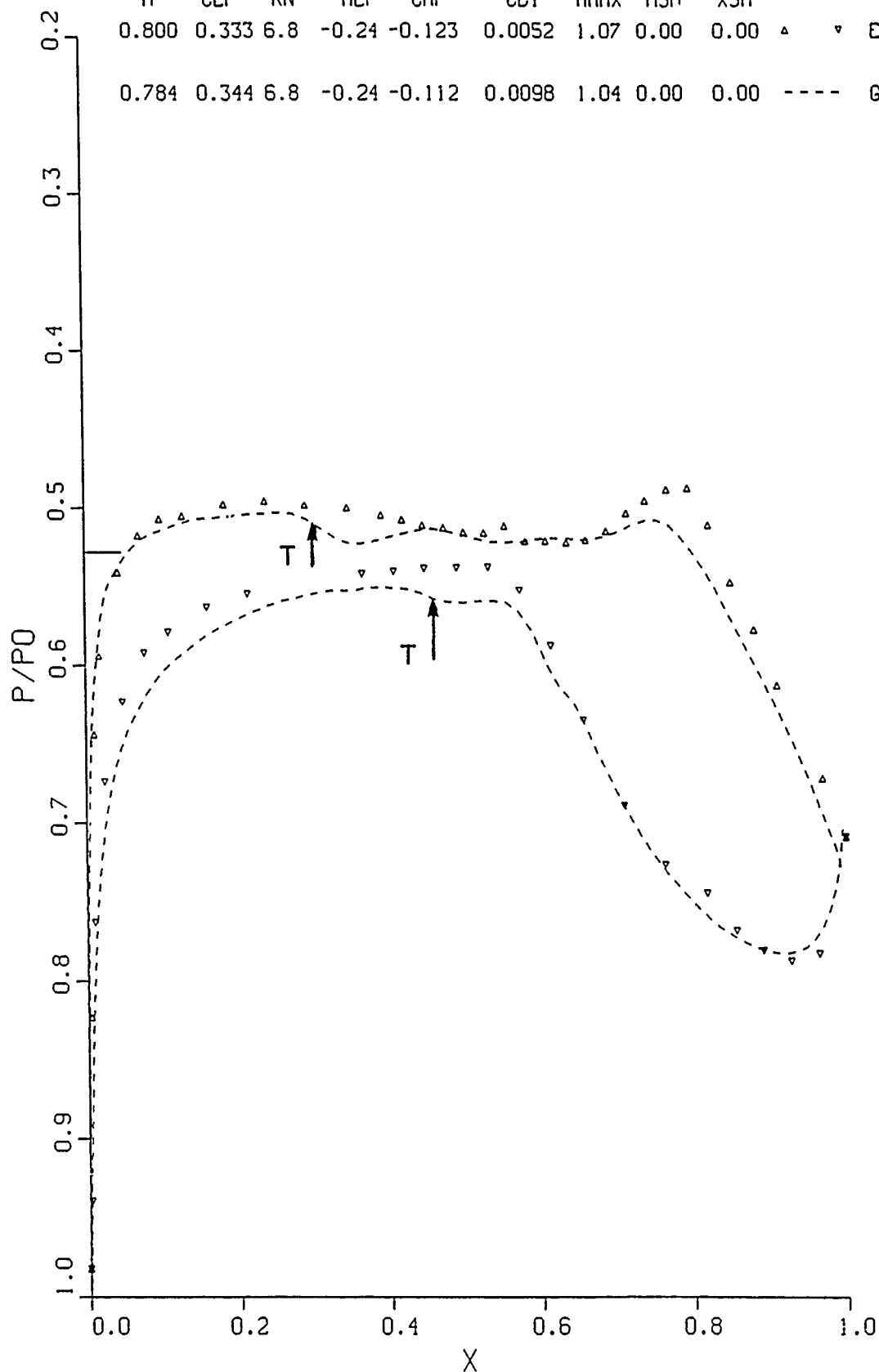
FIG. 64a: COMPARISON OF GRUMFOIL AND EXPERIMENT, TRANSITION FREE. 10% AIRFOIL. C_L \approx 0.333
