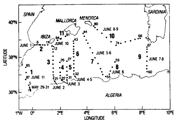
Fig. 1. Identification of CTD stations, section numbers, and dates.
