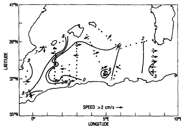
Fig. 8. Contours of minimum potential temperature above 350 m, indicating the concentration of W/W. In labeling the contours, the two leading digits, either 12 or 13, have been suppressed. Currents greater than 2 cm/s are indicated by arrows.
