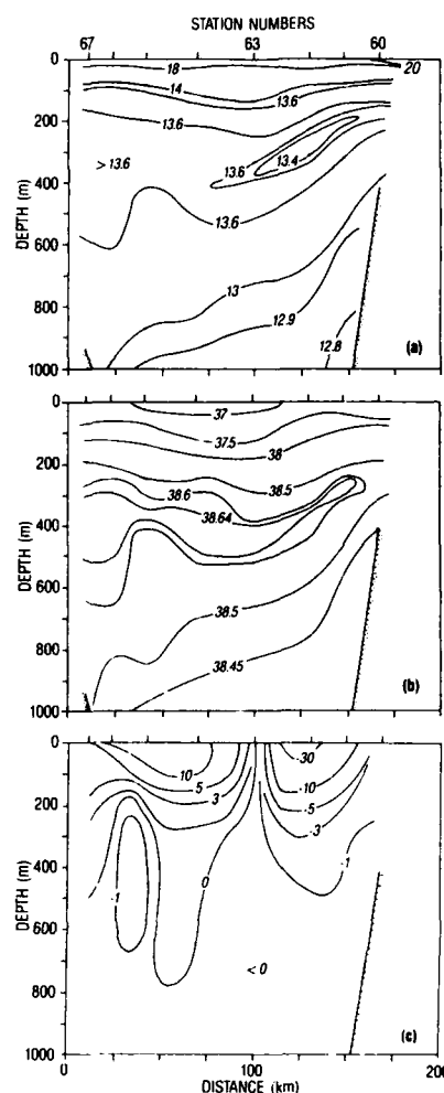
Fig. 4. Section 9, from the Algerian coast (station 60) across the Strait of Sardinia along longitude 8^{\circ}20'E . Otherwise as in Figure 3.
