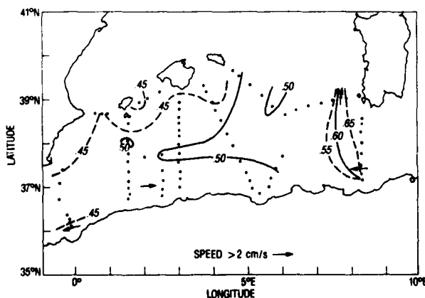
Fig. 7. Contours of maximum salinity, indicating the concentration of LIW. Contours are labeled with salinity in excess of 38 practical salinity units. Currents greater than 2 cm/s are indicated by arrows.
