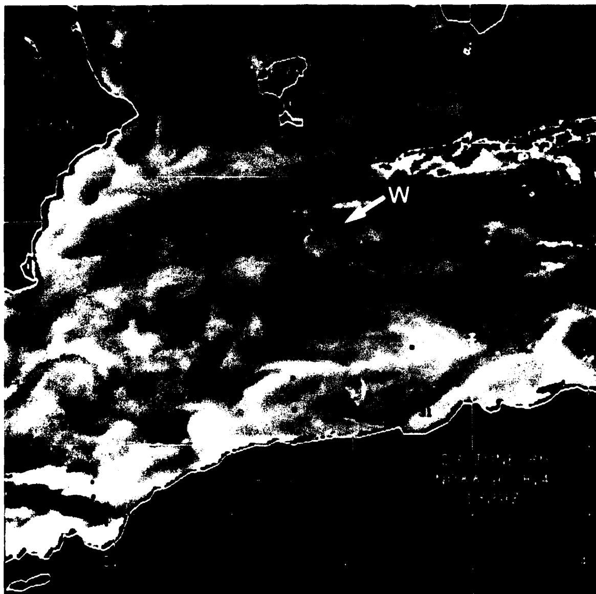
Fig. 9. Satellite IR image of June 3, 1329 UT, coincident with station 26. The eddy just north of station 26 is eddy W, a long-lived feature.
