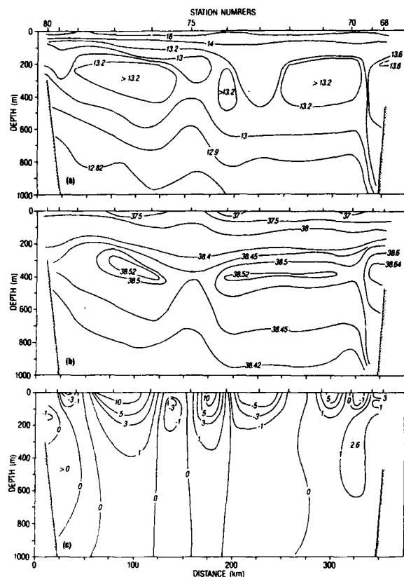
Fig. 6. Section 10. Sardinia (station 68) to Menorca. (a) Potential temperature, in degrees Celsius, (b) salinity, and (c) geostrophic current, cm/s, positive northward.
