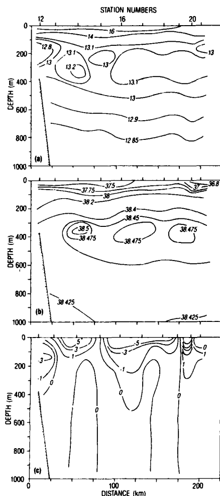
Fig. 3. CTD data along section 3 from Ibiza (station 12) southward to the Algerian coast along longitude 1^{\circ}30'E . (a) Potential temperature, in degrees Celsius. (b) salinity, and (c) geostrophic current, cm/s, positive eastward. The isotachs near station 20, too crowded to be labeled, show the AC confined to a jet with surface speeds of over 100 cm/s.
