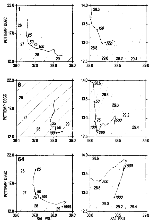
Fig. 2. TS plots for three stations showing characteristics of representative water masses. For each station, a full-depth plot is on the left, and an expanded plot of the deeper layers is on the right. Contours of sigma-theta are superimposed, and depths in meters are given at several points along each trace. Station 1 indicates MAW ( S < 37.5 ) in the upper 100 m near the Algerian coast. Station 8 has a layer of WIW ( T < 13.0 ) between 75 and 400 m. Station 64 illustrates the salinity maximum typical of LIW.
