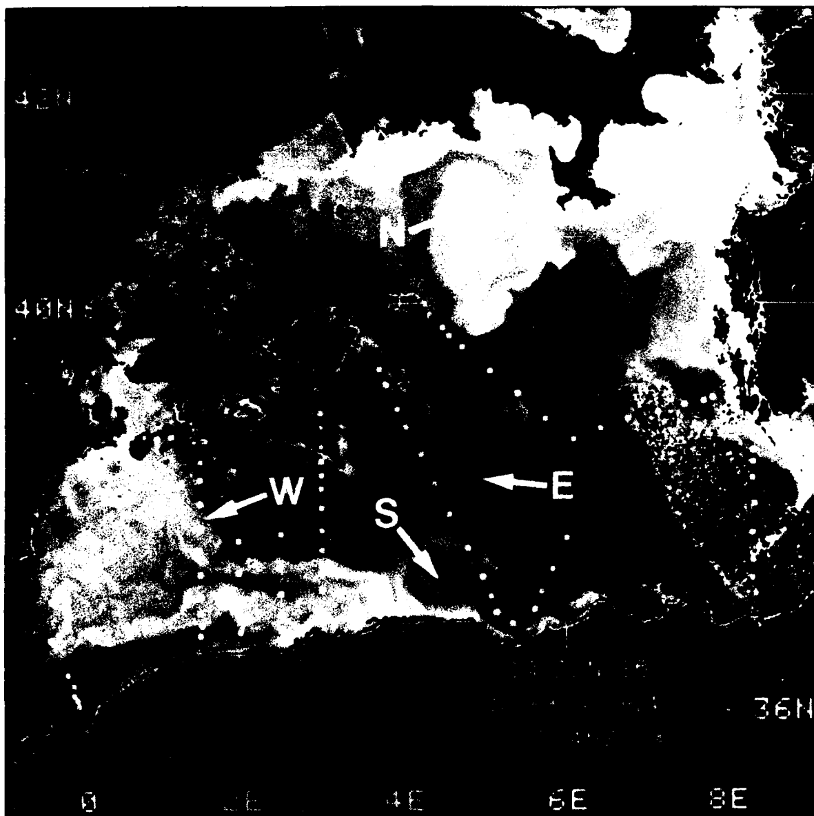
Fig. 5. Satellite IR image of June 9, 0248 UT. The picture was taken about one day after the end of section 9 and is nearly coincident with station 74. The arc of cool (light colored) water in the Strait of Sardinia is partly obscured by clouds, which appear as dark speckles.
