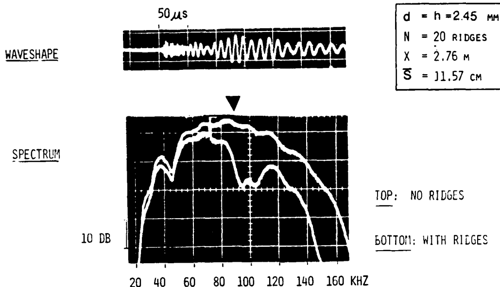
FIG . 8.7. Attenuation of transmitted underwater acoustic waves by ridge width resonances.
