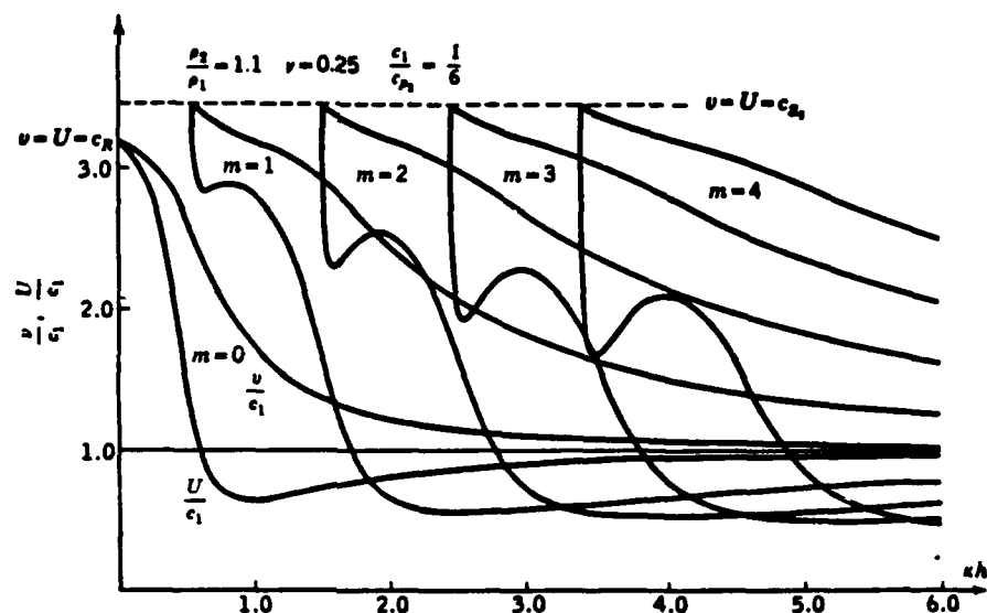
Fig. 4.33 Dispersion curves for a fluid layer overlying a semi-infinite elastic solid, for the first five modes.
