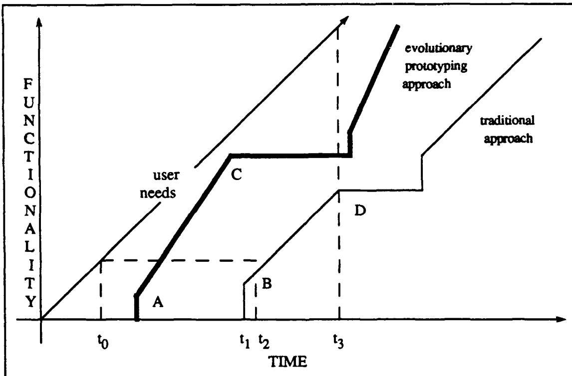
Figure 37. Evolutionary Prototype vs. Traditional Approach
