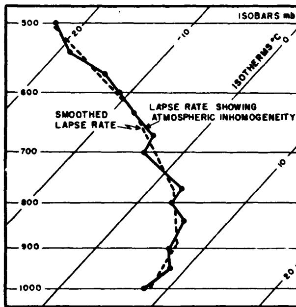
Figure 47. Effect of Atmospheric Inhomogeneity on an Otherwise Smooth Lapse Rate [ 55 ].
