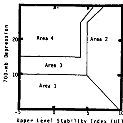
Figure 38a. Convective Gust Potential Graph.
