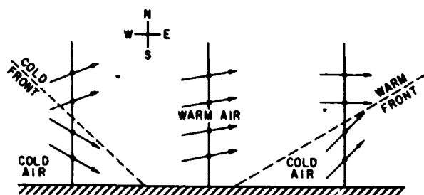
Figure 54. Vertical Distributions of Wind Direction in the Vicinity of Frontal Surfaces
