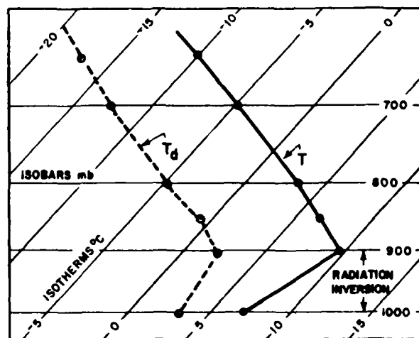
Figure 41. Nocturnal Radiation Inversion (1000 to 900 mb).
