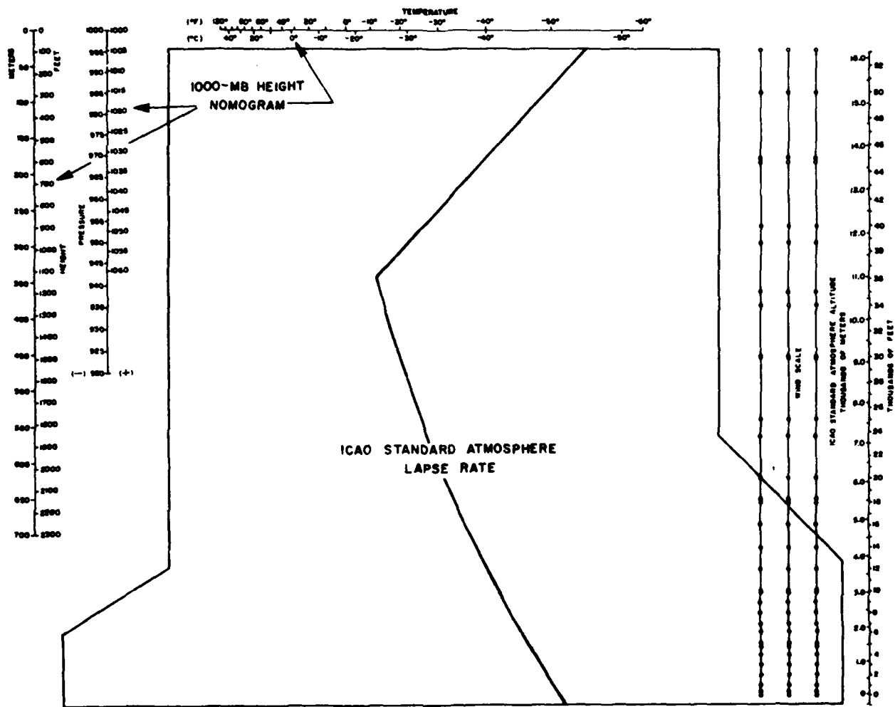
Figure 6. Auxiliary Scales on the Skew-T Chart.
