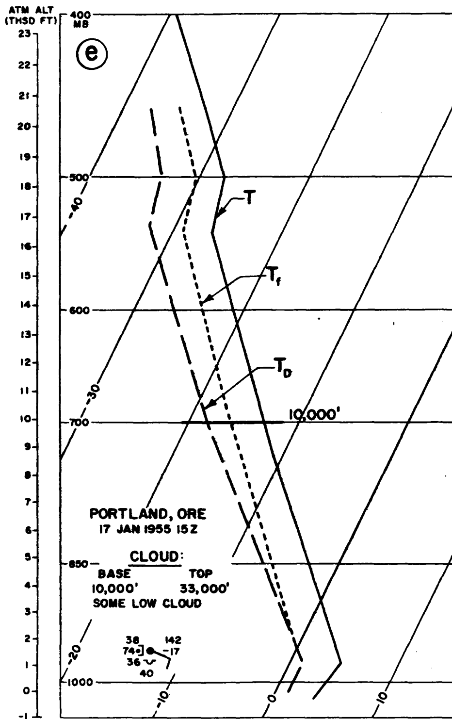
Figure 62s. Deep Layer of Cloud from Lower Levels to Tropopause with Some Clear Layers not Revealed by Sounding. There is cloud from 4000 feet to the tropopause, with the exception of an unspecified clear layer between the top of the low stratocumulus and the base of the middle cloud at 10,000 feet. From the sounding, there is little indication of any layering, and the dew-point depression is 4°C to 6°C throughout the sounding. This sounding is typical of solid or near-solid cloud from the surface to great heights in moderately cold atmosphere (500-mb temperature about -30°C).
