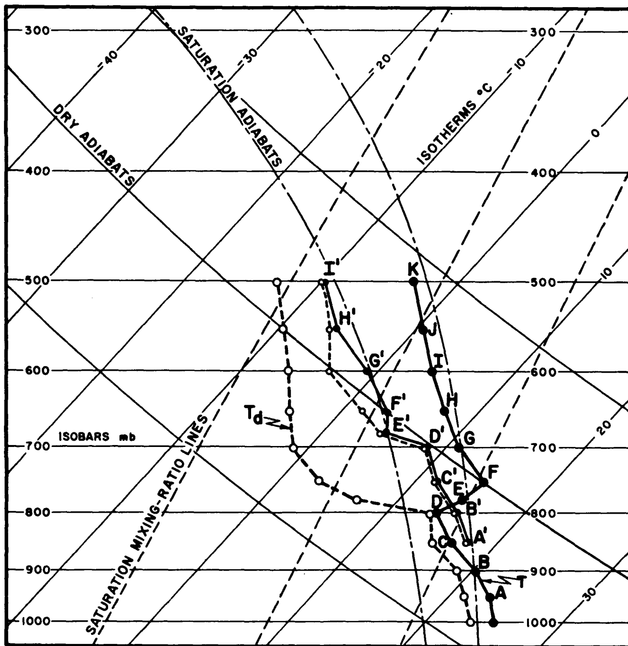
Figure 36. Superadiabatic Lapse Rate ( D'E' ) Resulting from Lifting an Air Mass 100 mb.
