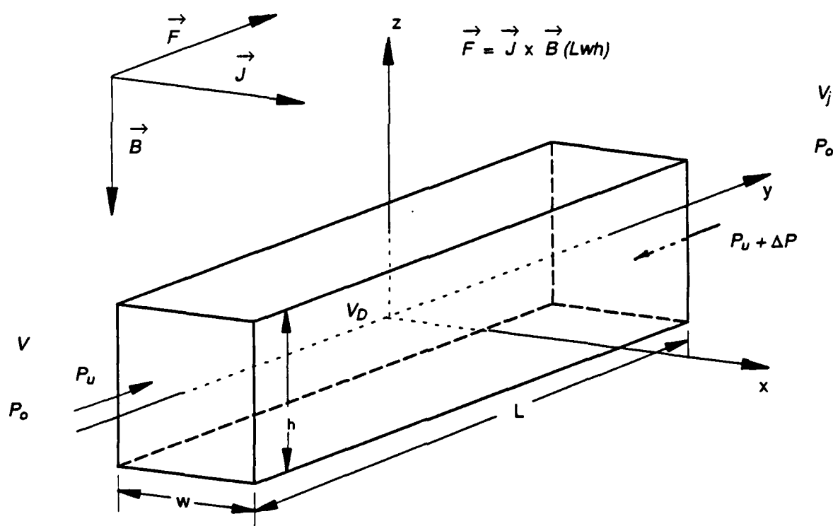
Fig. 6. Propulsive magnetohydrodynamic rectangular duct configuration.
