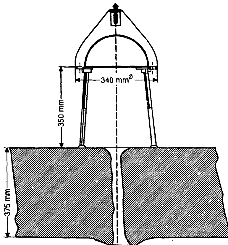
Blasting Charge for the Engineer Corps - HI 5 (15 KG Shaped Charge)
