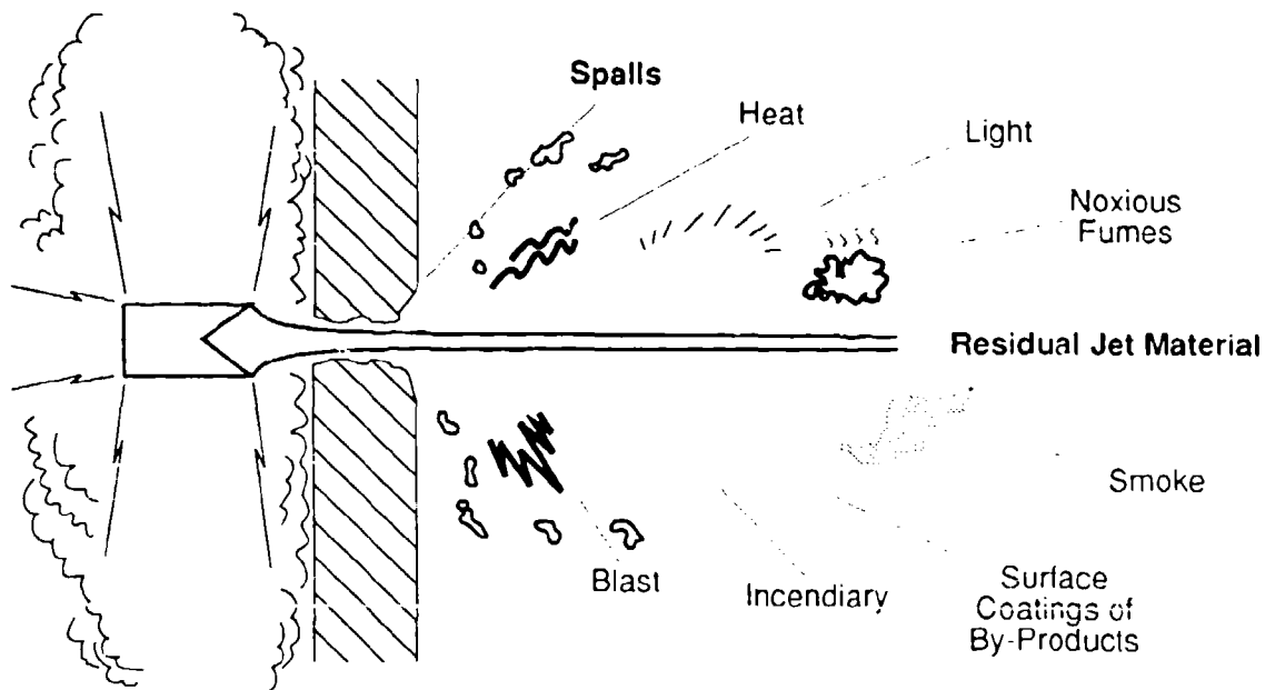
Fig. 45 Diagram of Behind Armor Effects
