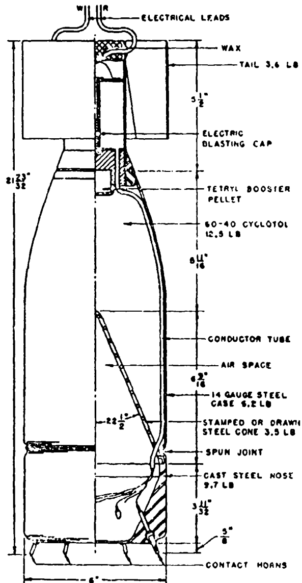
FIGURE 1. Antisubmarine shaped-charge bomb.
