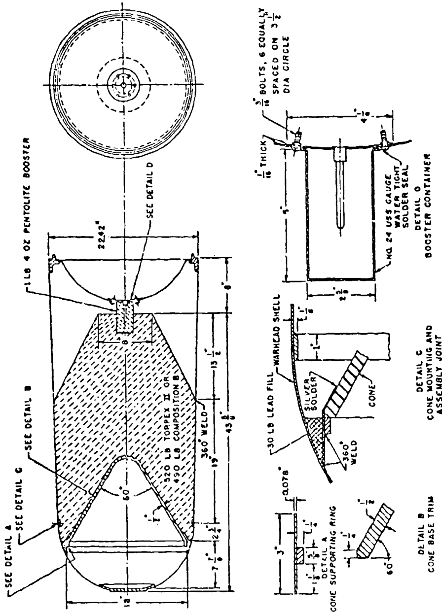
FIGURE 3. Shaped-charge torpedo warhead.
