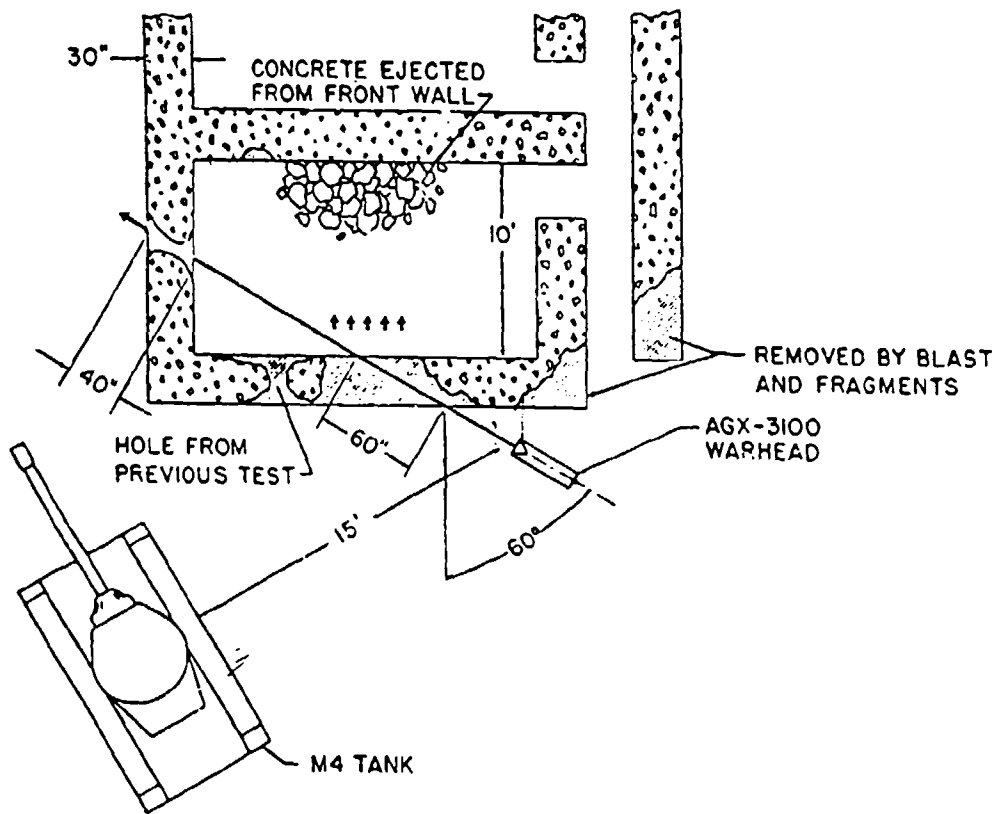
Test setup for AGX-3100 warhead Test No. 2. Jet penetrated more than 100 in. of concrete.
