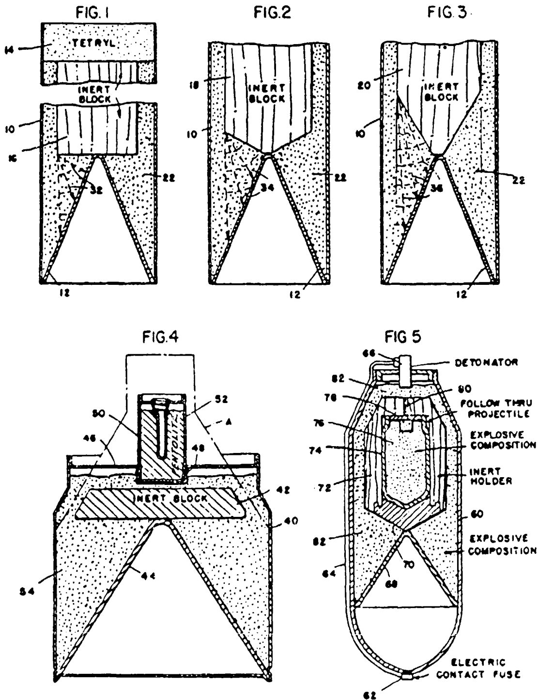
Fig. 38 Moses patent wave shapers, follow-through, U.S. 1949
