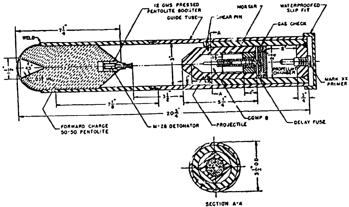
FIGURE 2. Antisubmarine shaped-charge follow-through bomb.
