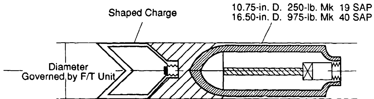
Concept: ACX-3300 Shaped Charge? SAP Follow-Through (F/T)
