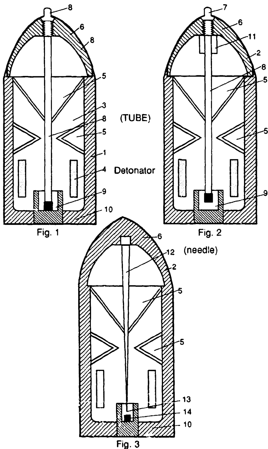
Fig. 16 Mohaupt, et al., first patent illustrations, 1939/1941
