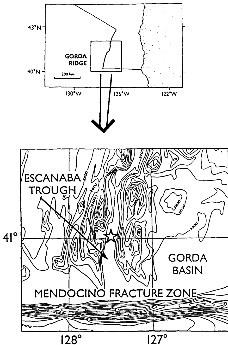
Fig. 5.1. Bathymetric chart showing location of northeast Pacific station in southern Escanaba Trough.
