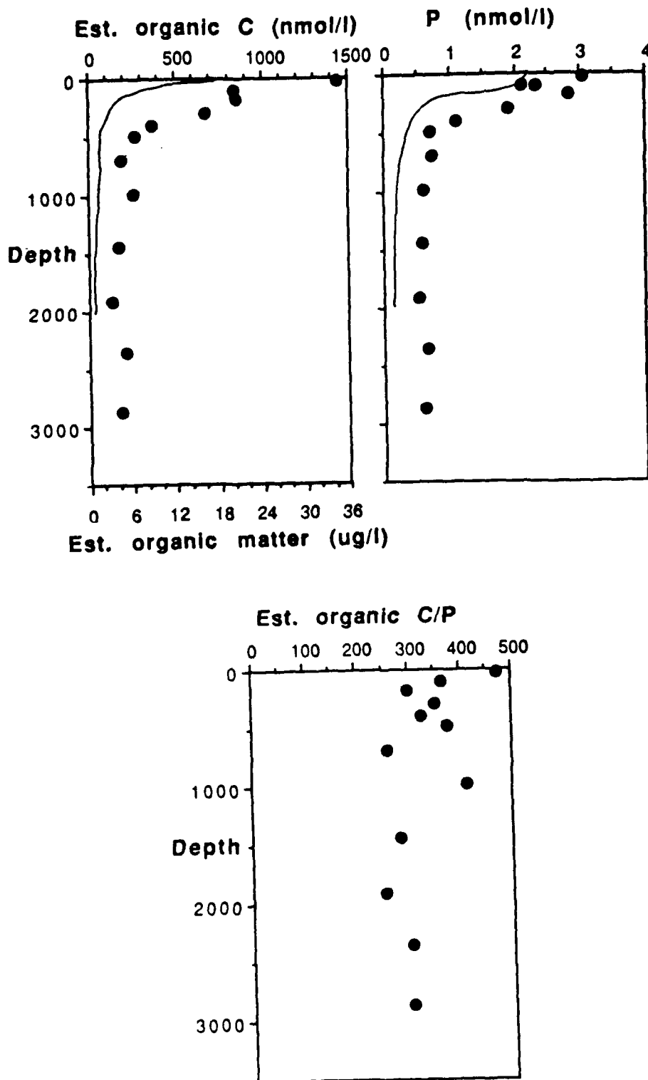
Fig. 5.4. Particulate organic carbon (estimated), phosphorus (measured), and organic C/P ratio (upper limit estimate).
