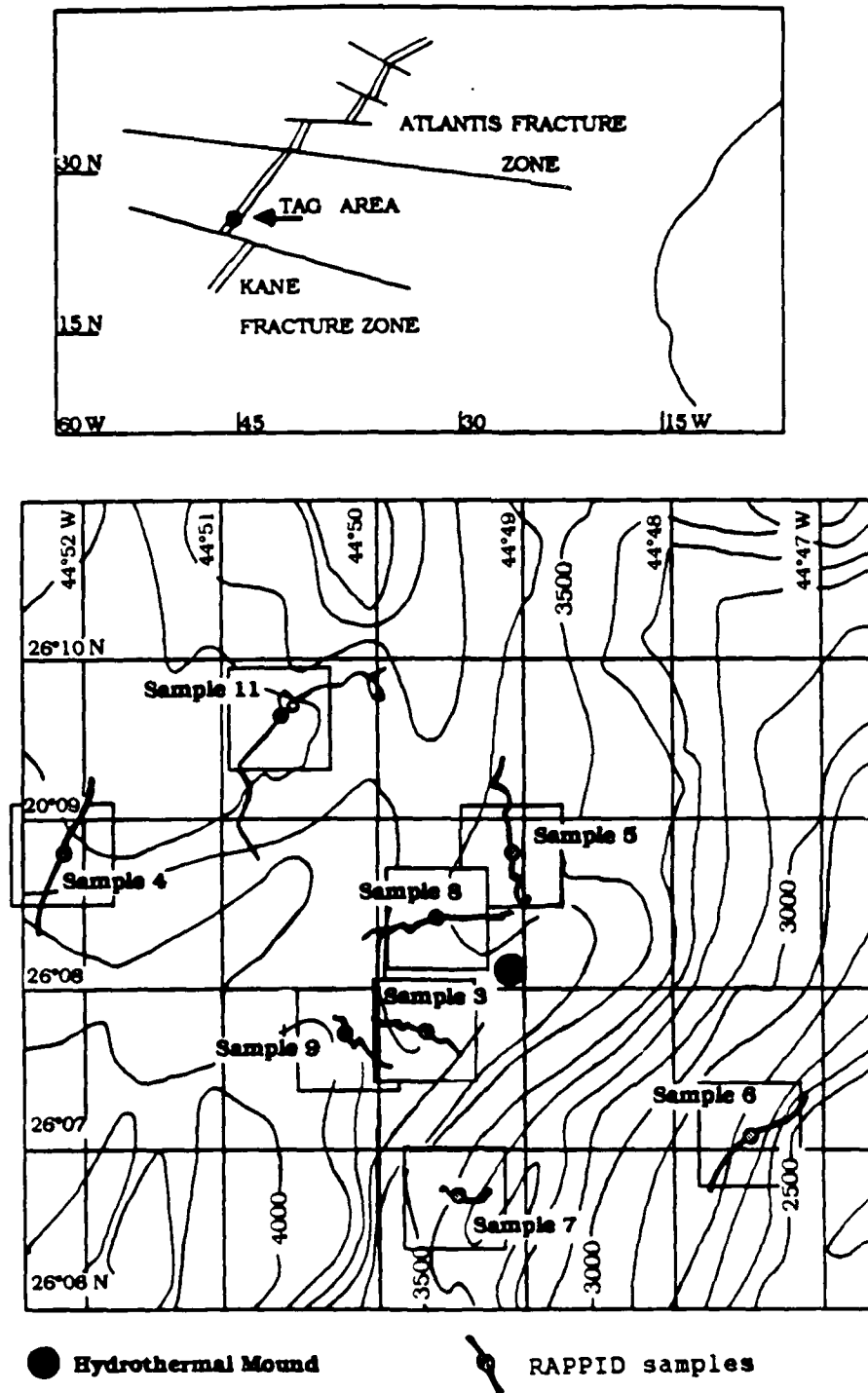
Fig. 6.5 TAG hydrothermal area and detail of approximate RAPPID pump sample locations (lines through points indicate approximate ship drift during pumping). Navigation was generally by satellite fixes and dead reckoning. Other sampling stations (FIDO pump, CTD) shown as well.
