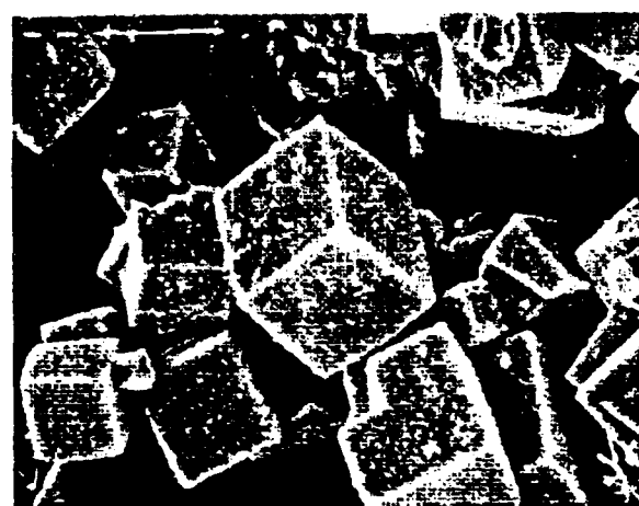
Figure 7. Cu powder reduced from DMFA with EG and PVP present, top. Cu powder reduced from DMFA with no surface additive, bottom.
