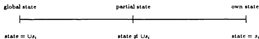
Figure 2.4: Spectrum of Local States
