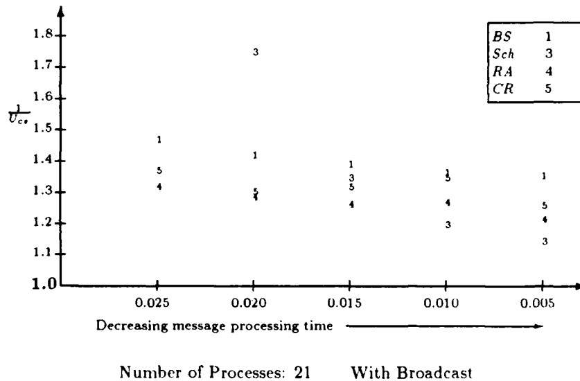
Figure 5.7: Algorithms in Fail-prone Environment
