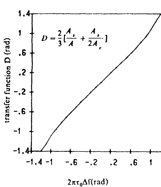
Figure 4. Transfer Function of Frequency Discriminator
