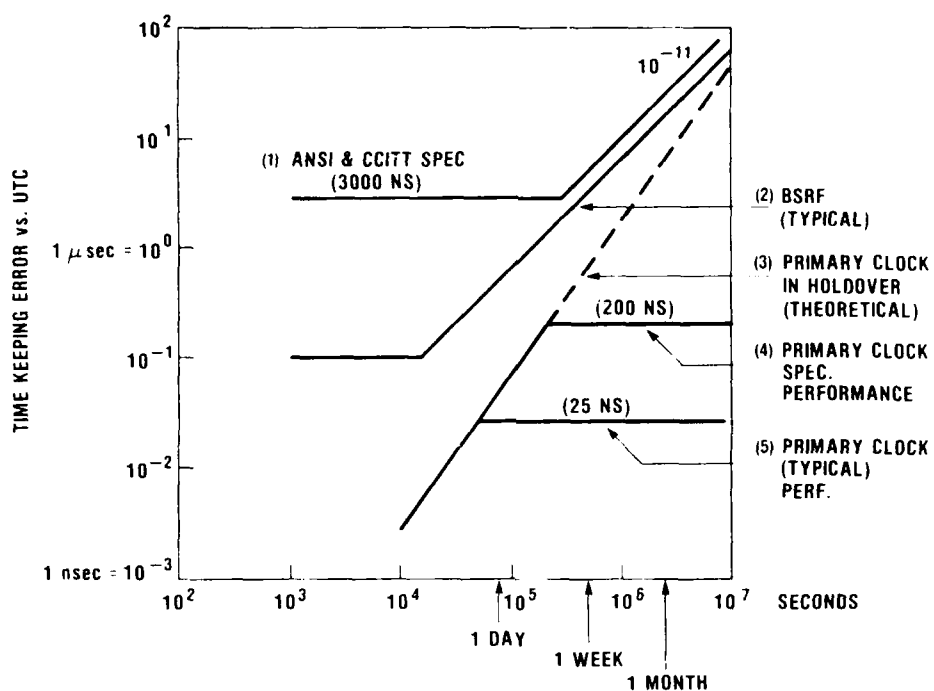
FIG. 7 PERFORMANCE COMPARISONS
