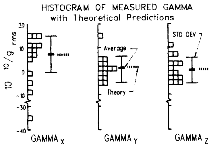
FIGURE 7. Histogram of gamma measured on each axis of 15 resonators (10 MHz, 3rd, SC-cut, 2-point mount.) Average and standard deviation of measured values are compared to analytically predicted values.
