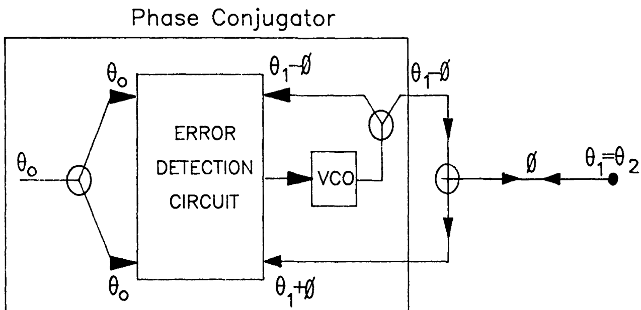
FIGURE 2. PHASE CONJUGATOR
