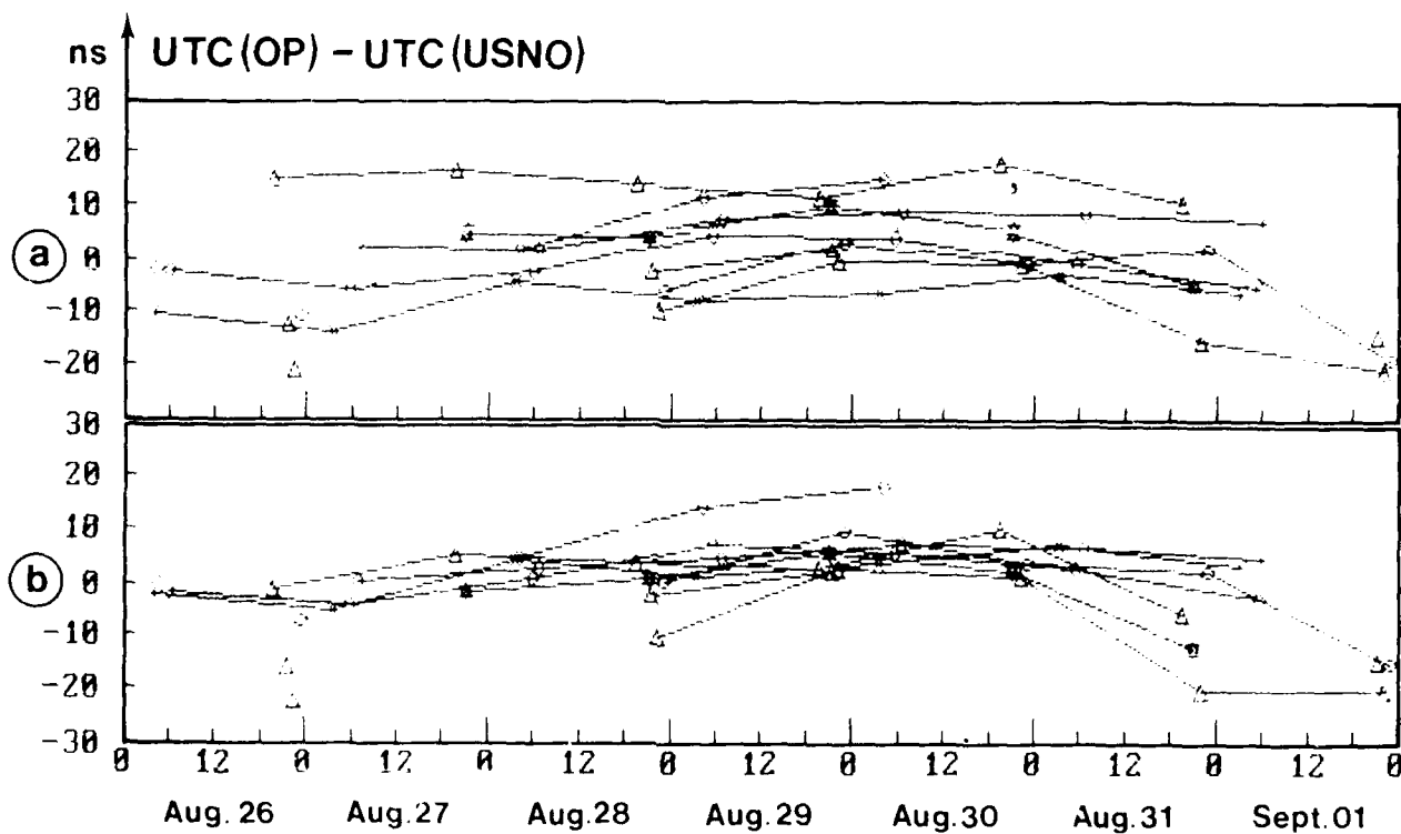
figure 5. Example of time comparison between OP and USNO
