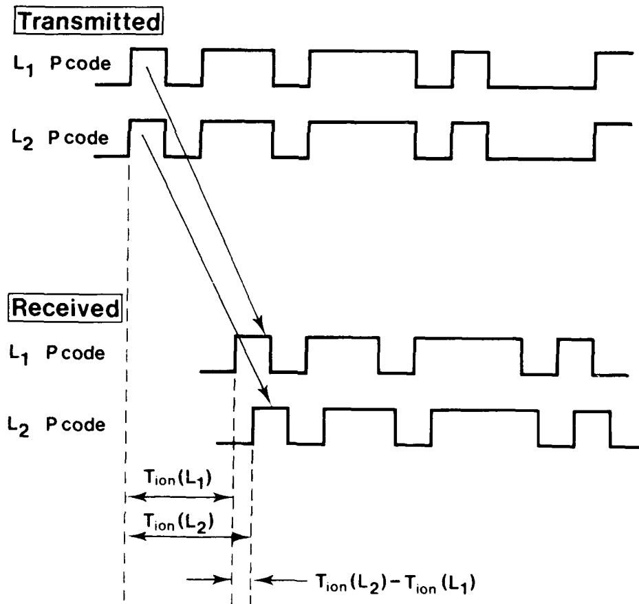
figure 1. Transmitted and received L_1 and L_2 P-codes.
