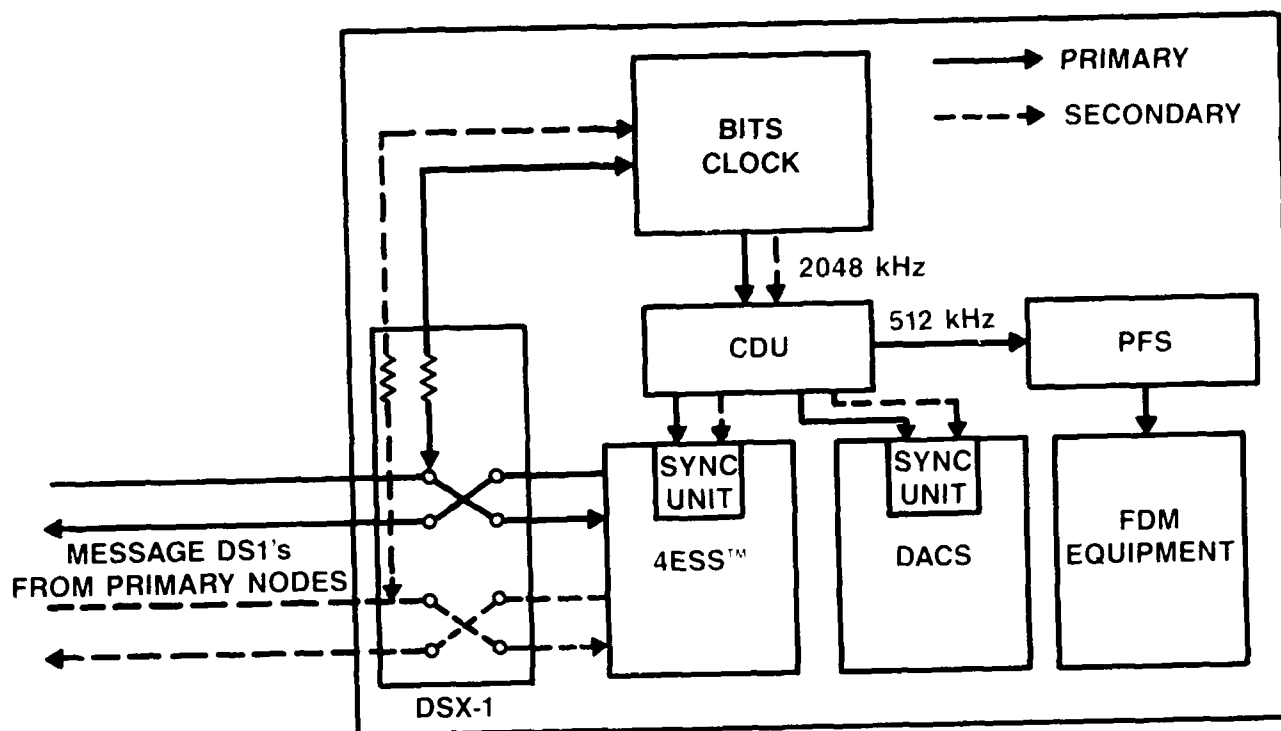
FIG. 5 SECONDARY NODE TIMING DISTRIBUTION
