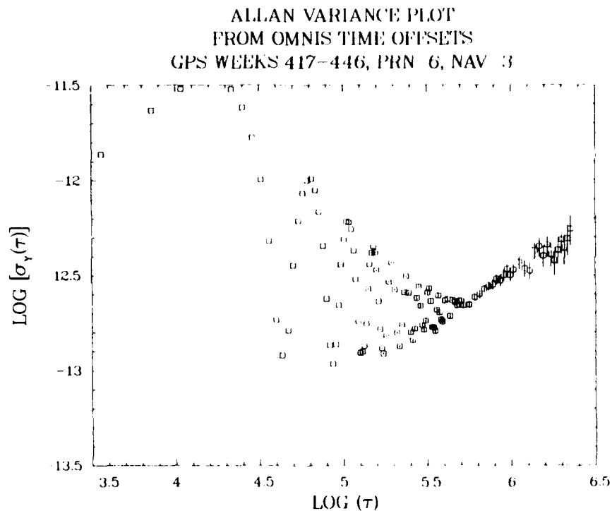
FIGURE 9. ALLAN VARIANCE FOR PRN6/NAV3 FOR WEEKS 417-446, 1988
