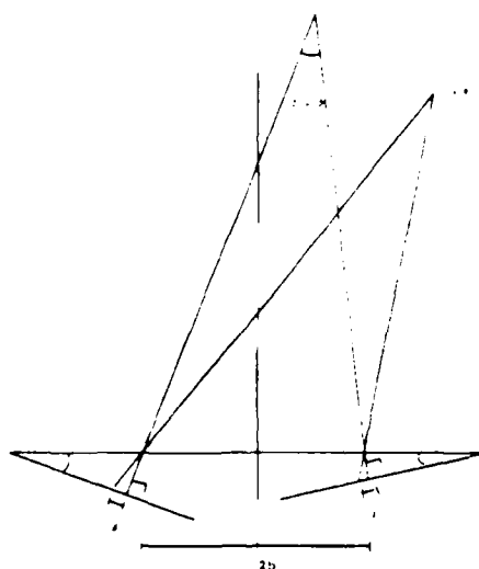
Figure 2.6: Configuration of two cameras whose optical axes intersect at a point.
