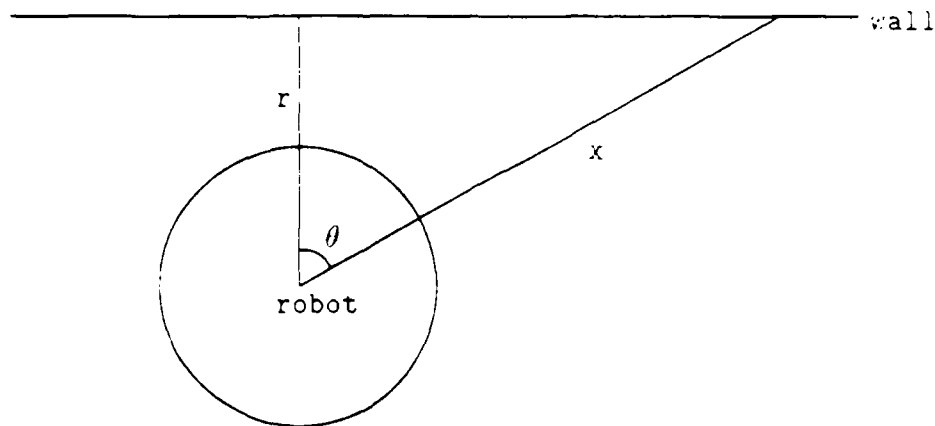
Figure 2.2: Same scene, top view.
