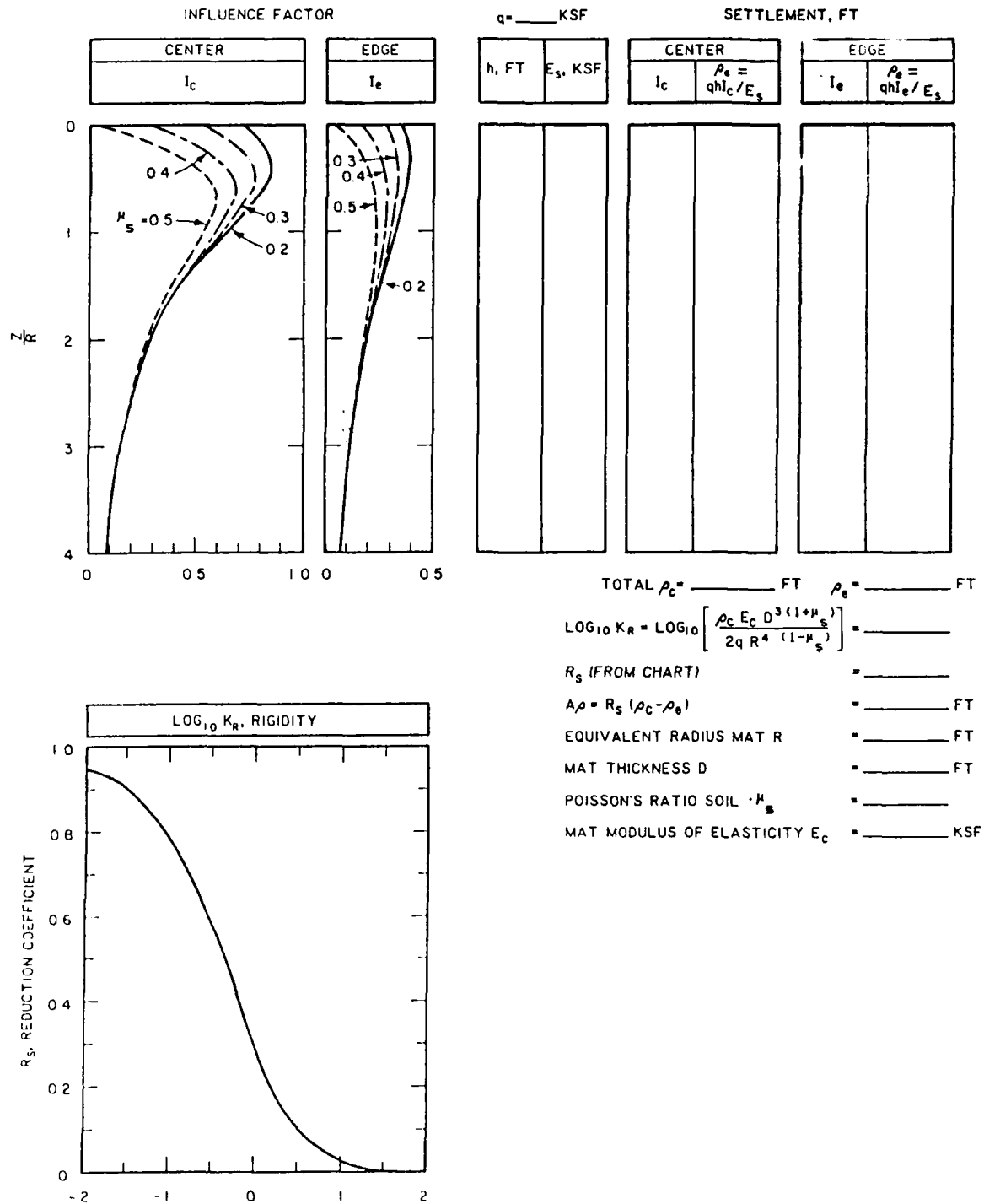
Figure 8. Settlement computation (after Kay and Cavagnaro 1983)
