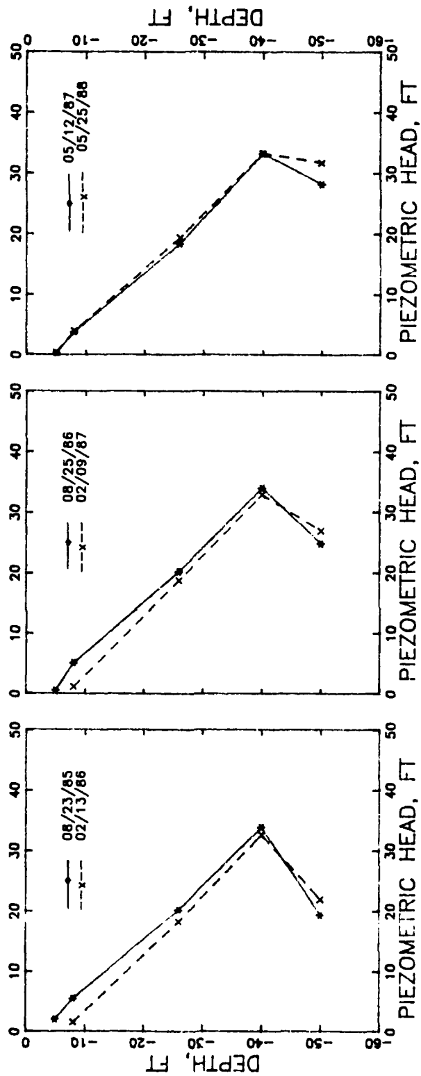
Figure 58. Piezometric heads
