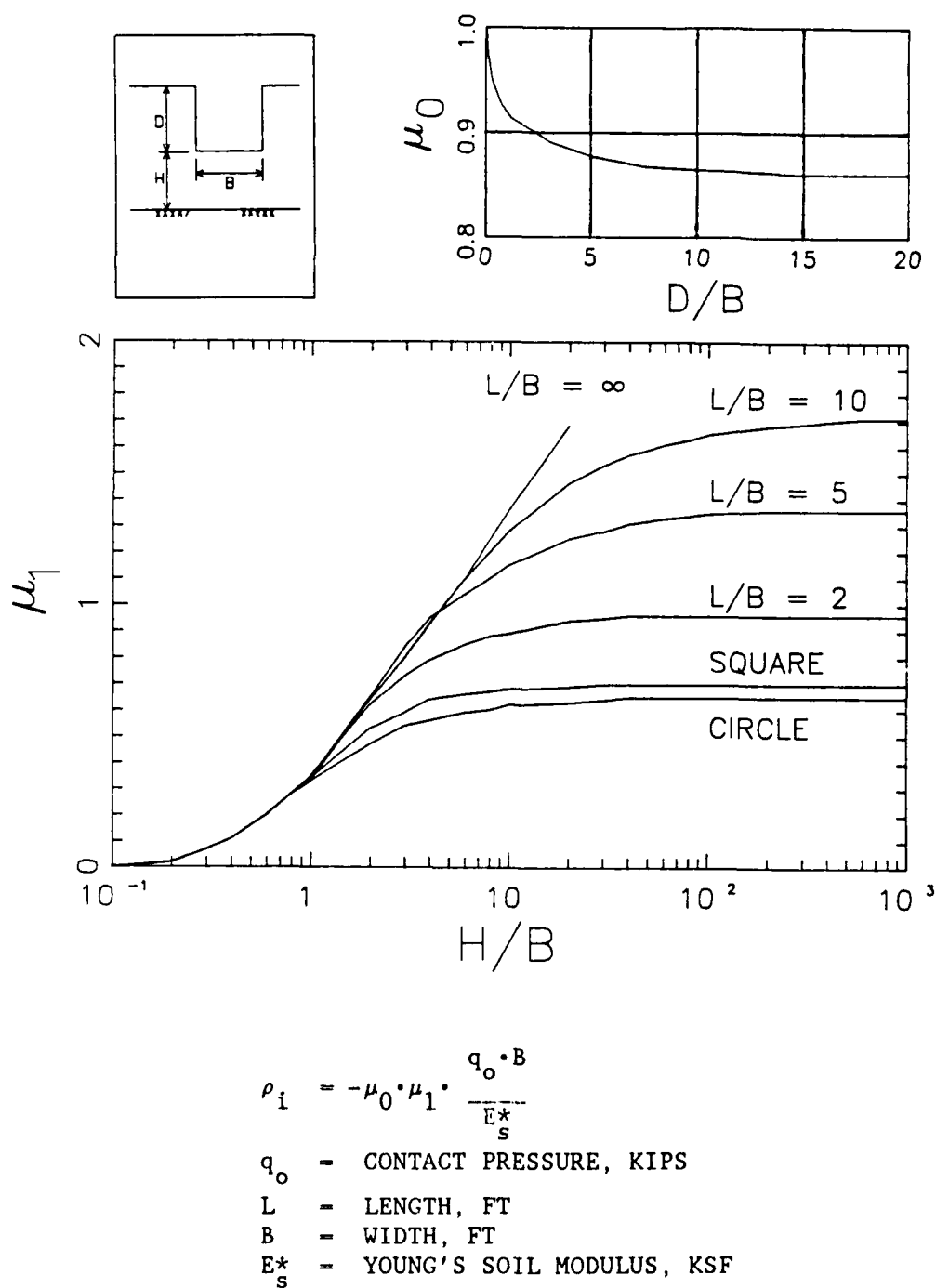
Figure 4. Chart for estimating immediate settlement in cohesive soil. Reprinted by permission of the National Research Council of Canada from the Canadian Geotechnical Journal , Vol 15, 1978, "Janbu, Bjerrum, and Kjaernsli's Chart Reinterpreted", by J. T. Christian and W. D. Carrier III, p 127
