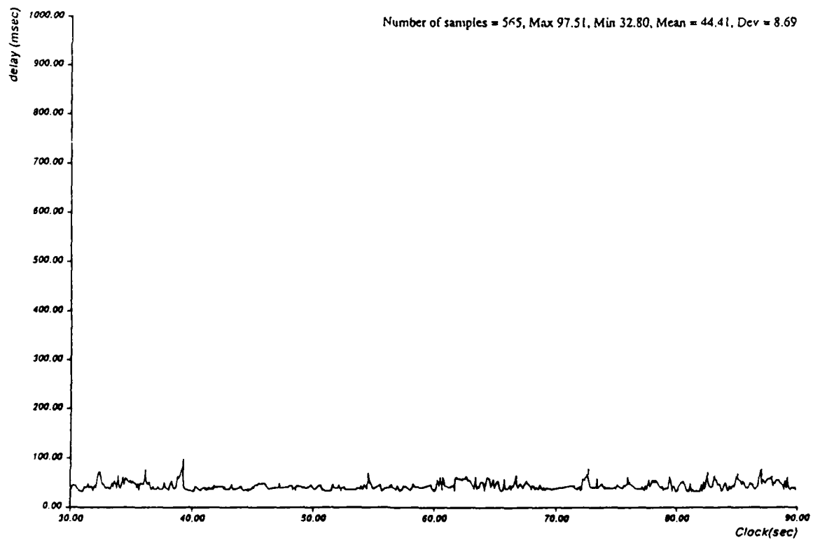
Figure 4-16: End-to-end packet queueing delay of 3-hop flows.
