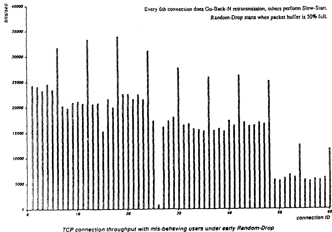
Figure 4-13: TCP-SS connection throughput with random drop (with misbehaving users).
