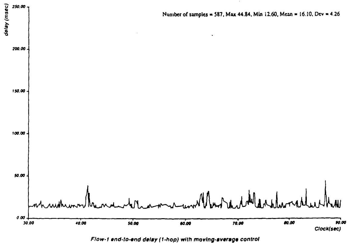
Figure 4-15: End-to-end packet queueing delay of 1-hop flows.
