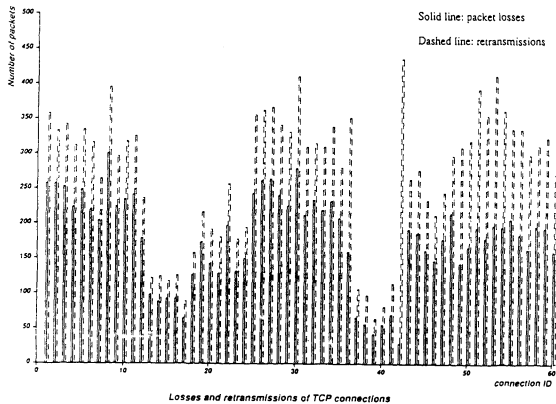
Figure 4-7: The average throughput, packet losses and retransmission of TCP-SS connections.
