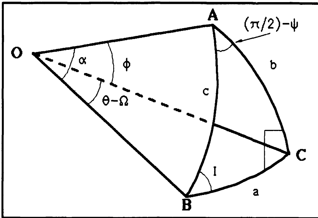
Figure A2. Spherical Triangle Relating Planetocentric Angles to Orbital Elements
