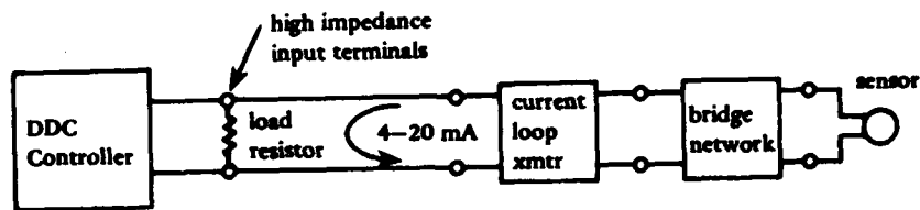
Figure 19. Current loop transmitter.
