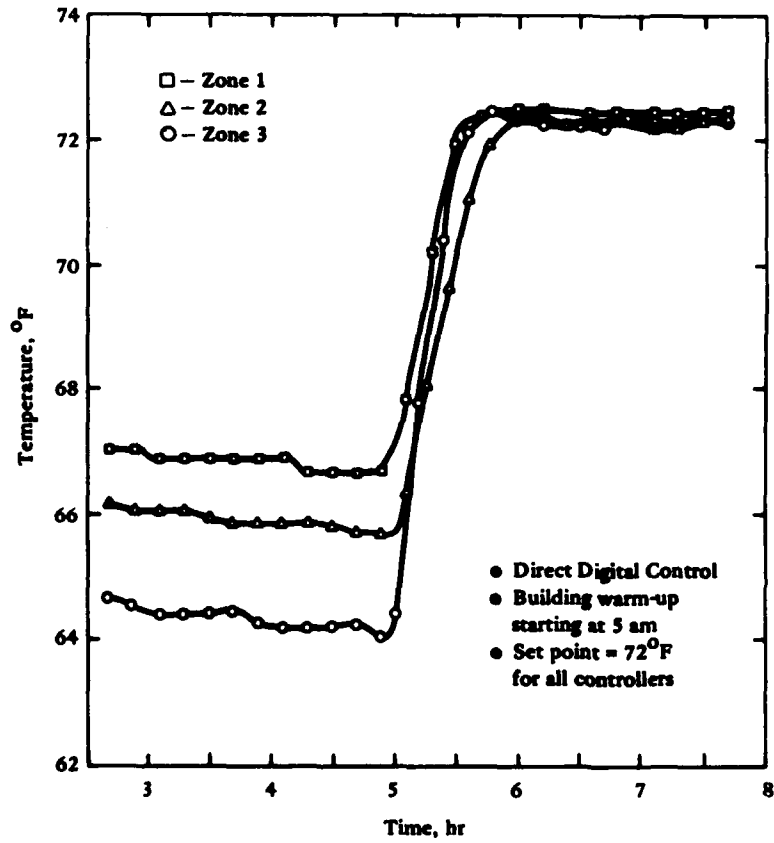
Figure 12. Measured system performance with Direct Digital Control. (Ref 1)
