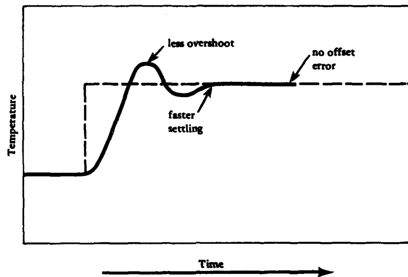
Figure 10. Proportional/integral/derivative control.
