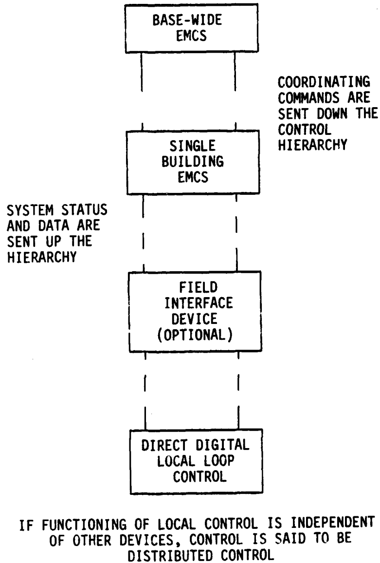
Figure 3. Relationship between DDC and EMCS.
