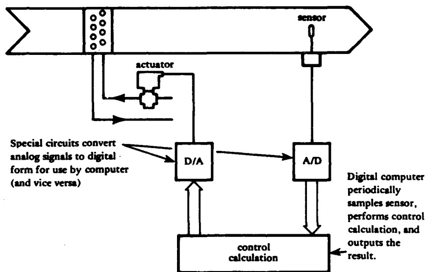
Figure 1. A digital control system.
