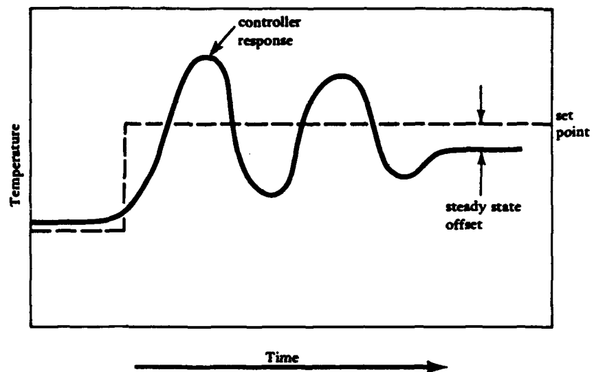
Figure 9. Proportional control.
