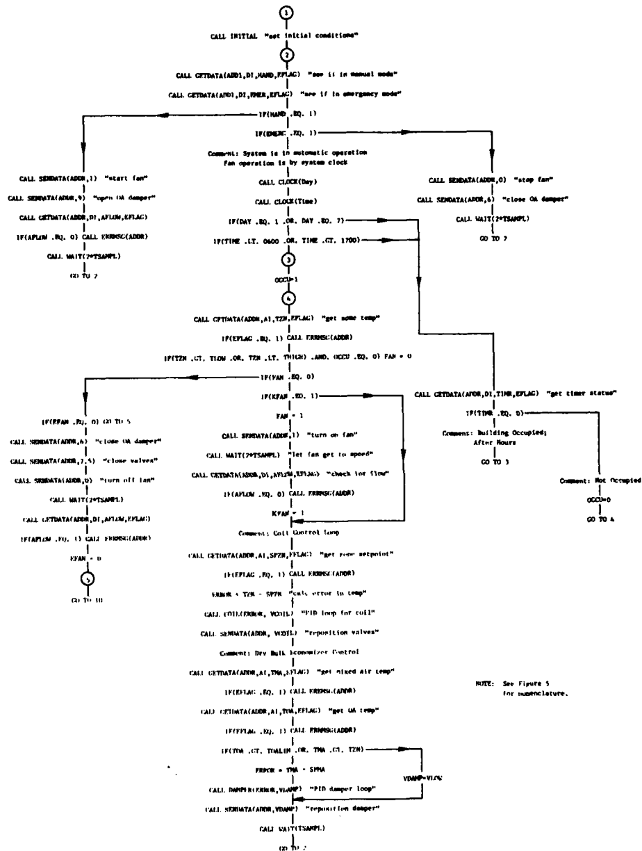
Figure 7. Control program flowchart for DDC System.
