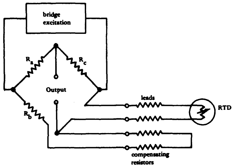
Figure 18. Four wire RTD sensor and bridge circuit.
