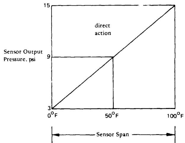
Figure 4. Illustration of sensor nomenclature.
