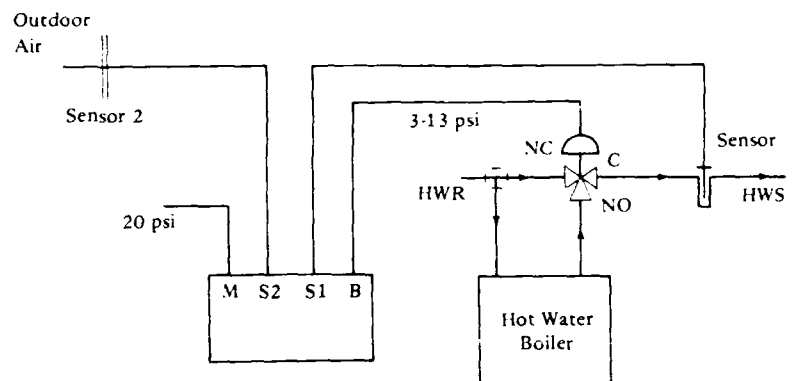
Figure 6. Application of Two-Input Controller.
