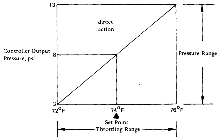
Figure 3. Illustration on controller nomenclature.
