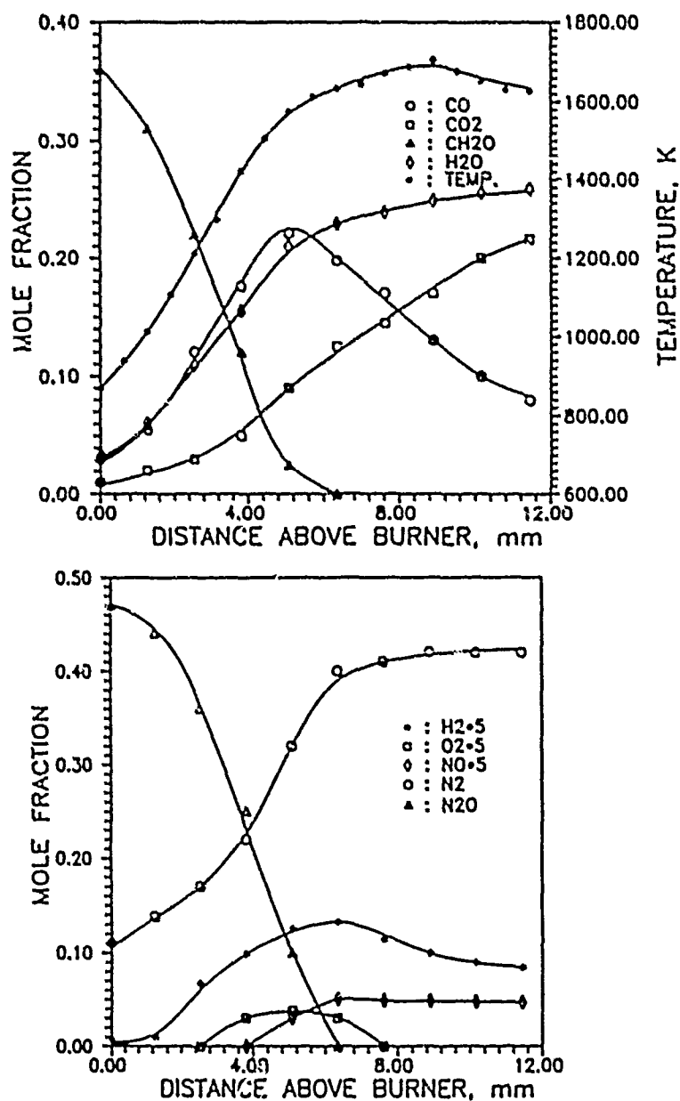
Figure 2. Measured concentration profiles in a \text{CH}_2\text{O}/\text{N}_2\text{O} laminar premixed flame at 50 torr. The reactant mole fractions are 0.43 \text{CH}_2\text{O} and 0.57 \text{N}_2\text{O} and the total flowrate is 2.21 standard liters per minute.
