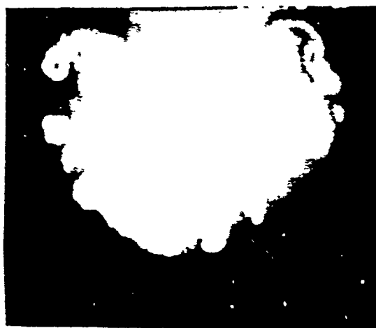
\alpha = 0.5
