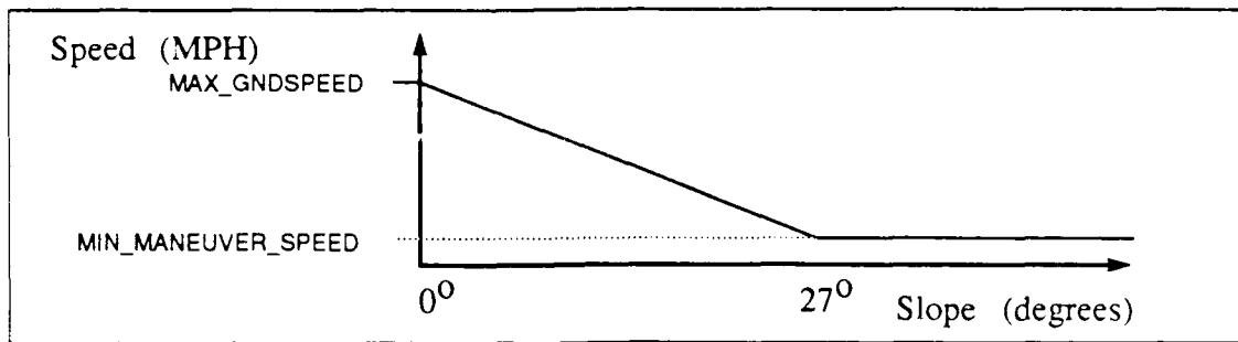
Figure 3-5 Slope Governor Function
