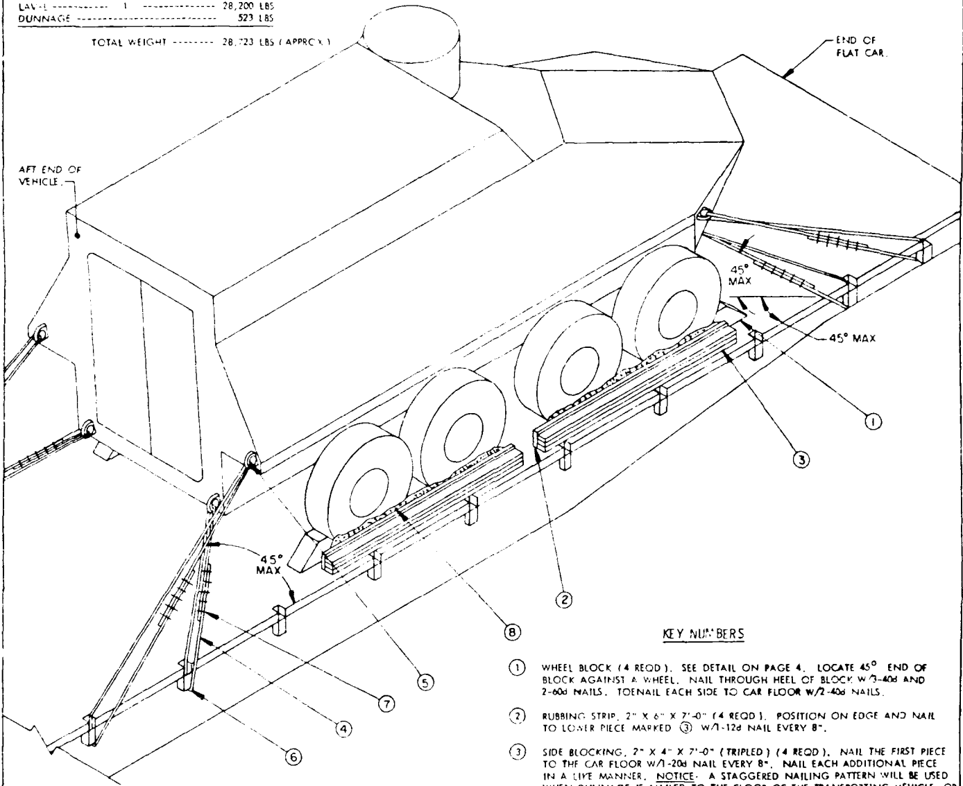
ISOMETRIC VIEW
