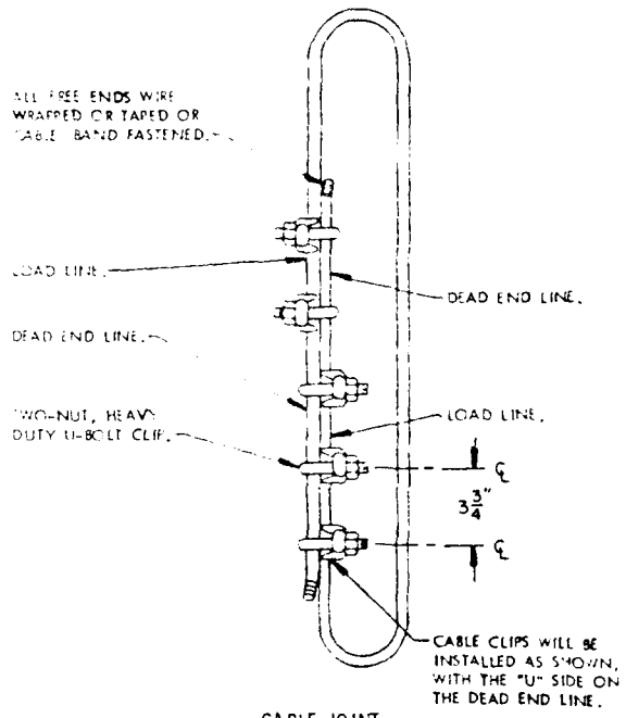
CABLE JOINT
