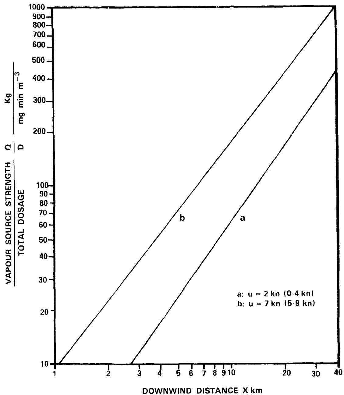
Figure 9 DISPERSION OVER LAND STABILITY CATEGORY S = 9
