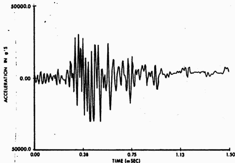
Figure 6. Typical Muzzle Acceleration During Firing
