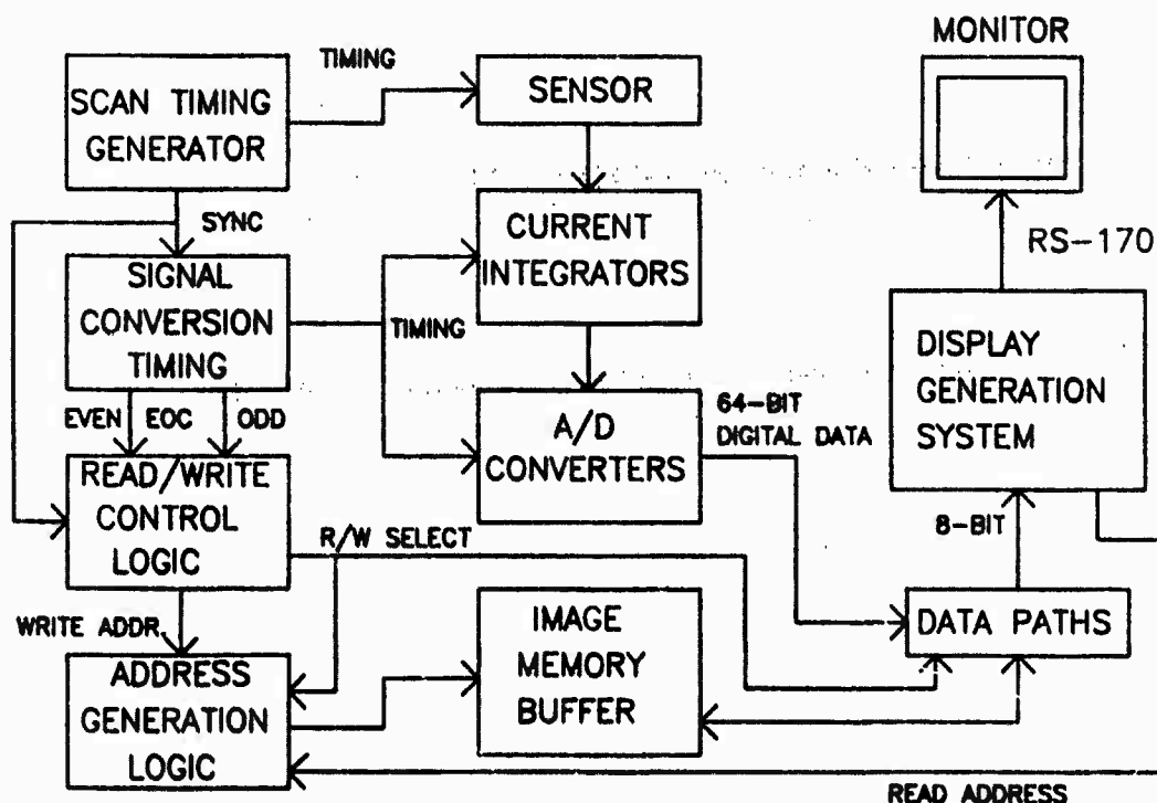
Figure 14. Camera System Block Diagram
