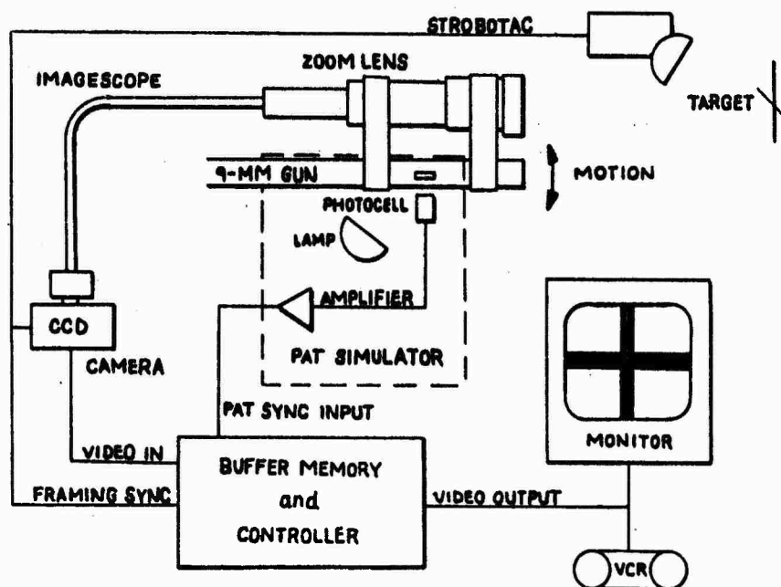
Figure 17. System Used to Physically Simulate PIMS Concept
