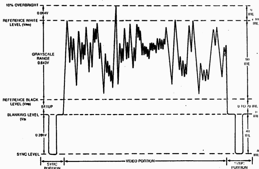
Figure 16. RS-170 Video Signals
