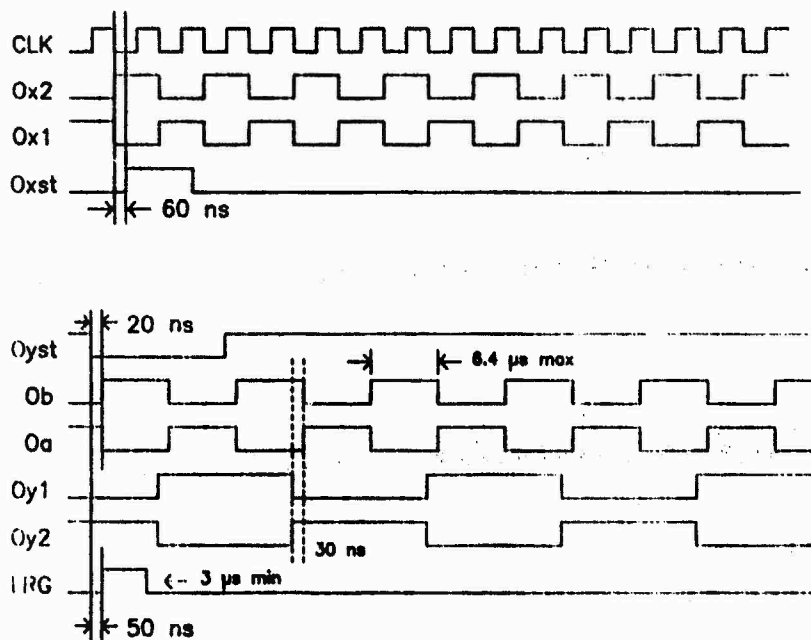
Figure 12. Sensor Clock Signal Timing
