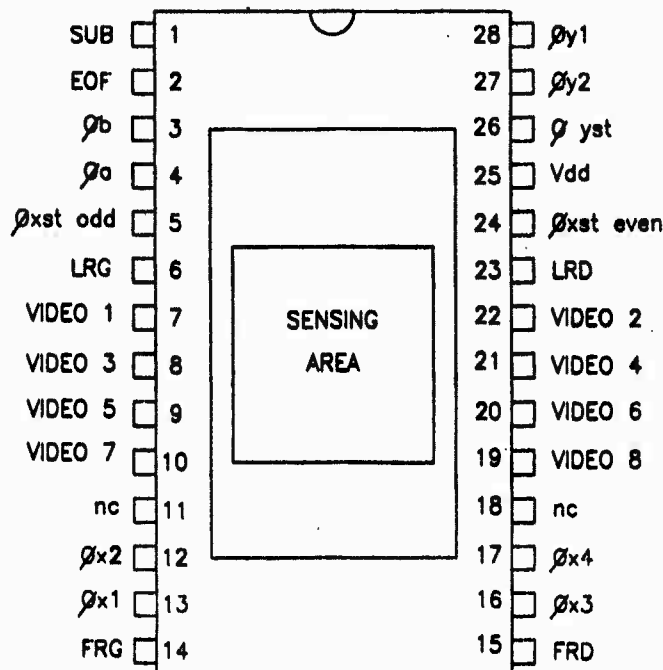
Figure 10. High Speed Sensor
