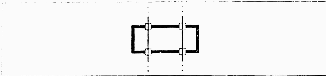
Figure 4.12. Trivial Cycle
