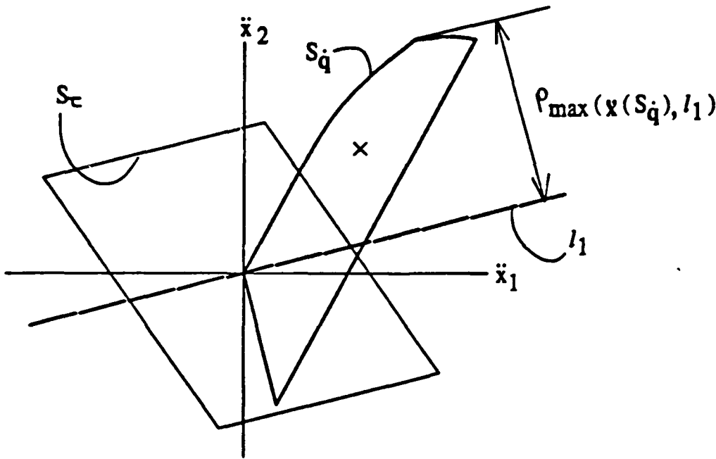
Figure 13: Maximum distance from reference line l_1 to a point on the set S_{\ddot{q}}
