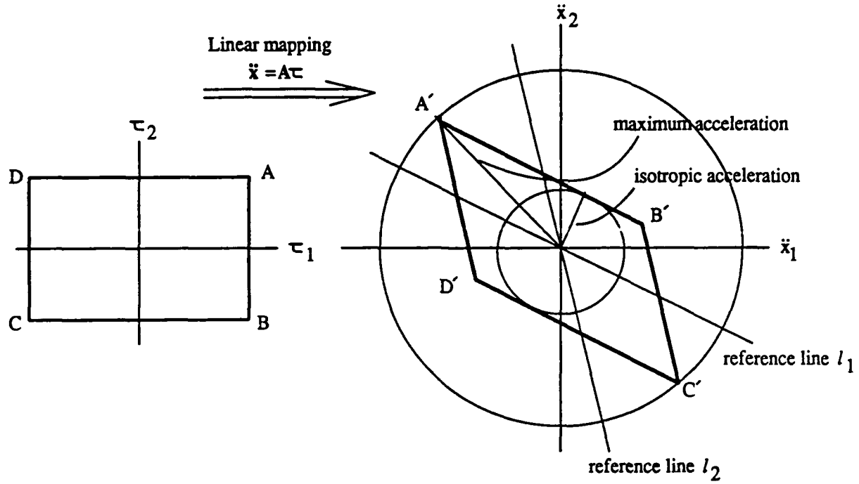
Figure 12: Characterization of the image set of the linear mapping for a two degree-of-freedom manipulator
