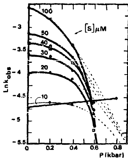
Fig.1 - Pressure dependence of the observed rate of carbamylation at 35^\circ\text{C} , \text{pH} = 7.4 ; v = 6.25 \text{ IU.}\mu\text{l}^{-1} ( 1 \text{ IU} = \mu\text{mol BuSCh hydrolysed.min}^{-1} at V_{\text{max}} in 0.1\text{M} phosphate \text{pH} 7 , 25^\circ\text{C} ).
