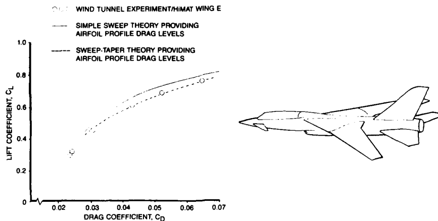
Figure 7 HIMAT Maneuver Polar Comparison
