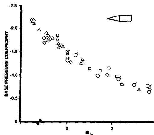
Figure 28 Base Pressure Test Data Scatter
