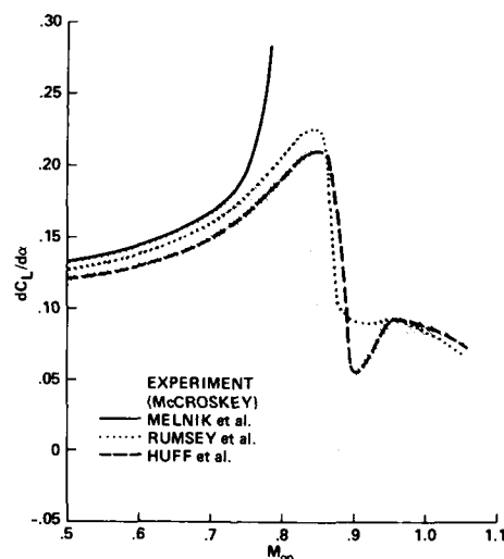
Fig. 7.- Comparison of computed and measured results for the lift-curve slope as a function of the freestream Mach number, \alpha = 1.49^\circ , C_A airfoil.
