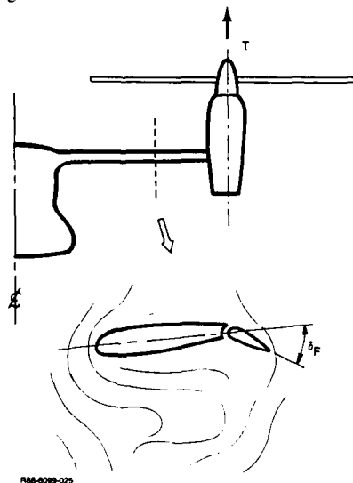
Figure 24 Rotor Downwash - Airfoil Interaction Schematic
