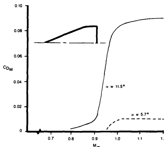
Figure 23 Wing Planform Wave Drag Due-to-Lift Prediction (Ref. 18)
