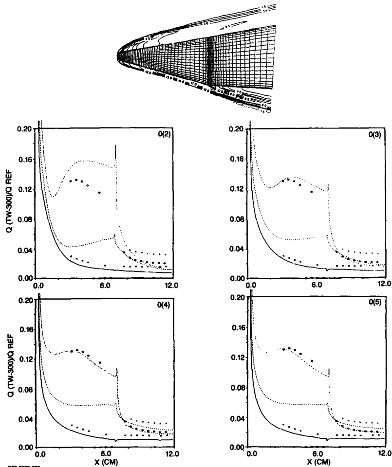
FIG-6080-022 Figure 22 Effect of Convergence Level on Hypersonic Heat Transfer M = 10
