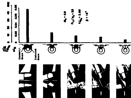
Fig. 40: Afterbody Drag Increment for Fighter Aircraft
