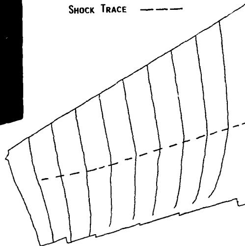
Fig. 19 - Experimental and Numerical Oil Flow. Attached Flow
