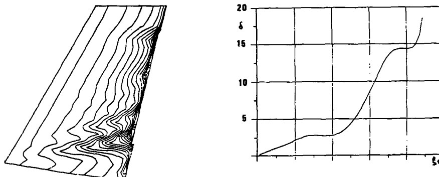
Fig. 8 - Delta Distribution Over Wing Upper Surface
