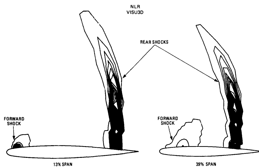
Fig. 11 Visualization of wave drag on two sections of the 'ONERA M6 wing' at M_{\infty} = .84 , \alpha = 6^\circ
