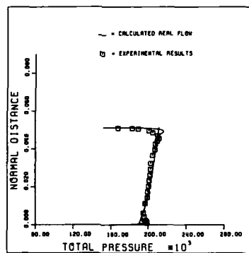
c) Rotor exit (Station 2)
