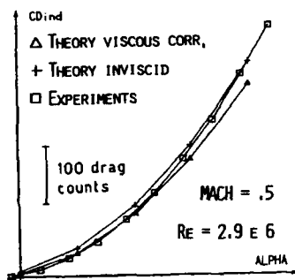
Fig. 12.b - Induced Drag Coefficient
