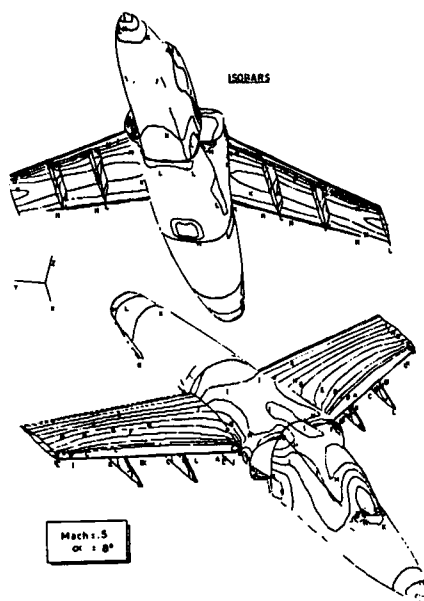
Fig. 6 - Theoretical Pressures
