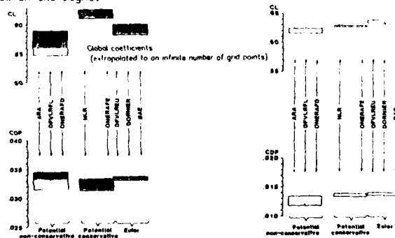
Fig. 13: Comparison of CFD Methods for Wing Analysis
