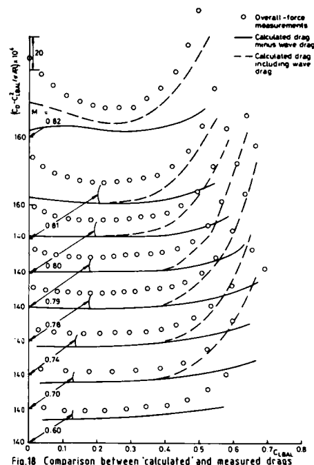
Fig.18 Comparison between 'calculated' and measured drags
