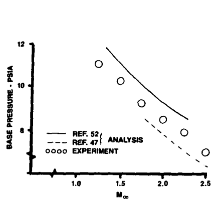
Figure 27 Effect of Mach Number on Base Pressure
