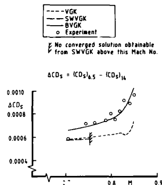
Fig.10 Differences between notional drag per surface at two unit Reynolds numbers, R = 6.5 \times 10^6 and R = 14 \times 10^6 , RAE 5238
