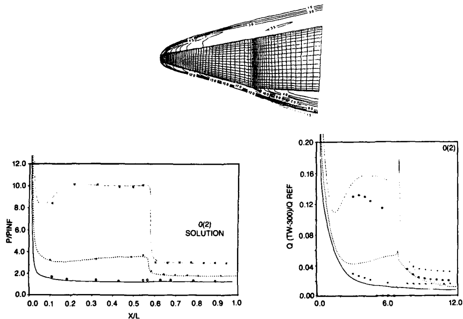
Figure 2 Pressure Field & Heat Transfer Computational (after 1/2 Hour on Cray X-MP)
