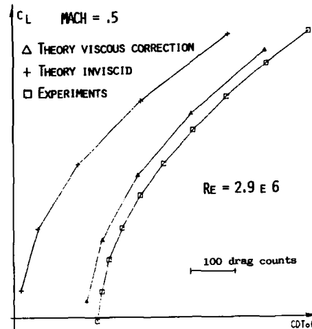
Fig. 13 - Total Drag Coefficient
