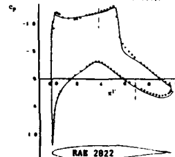
Fig. 10: 2D Zonal Navier-Stokes Solution
