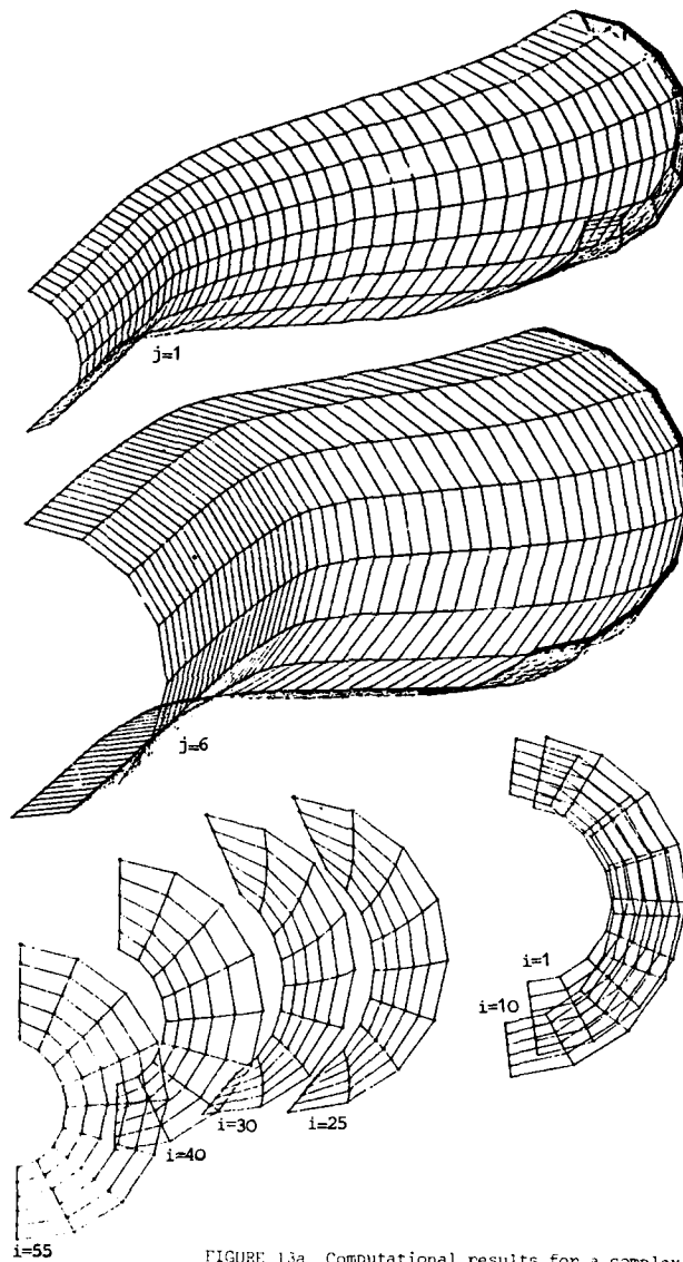
FIGURE 13a Computational results for a complex geometry duct. The computational grid.
