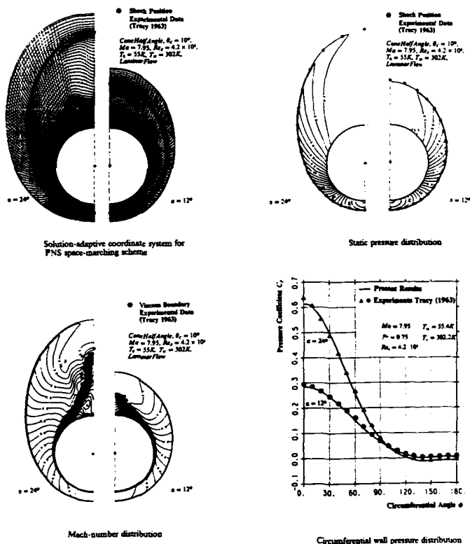
Fig. 49: PNS Selection for Cone at Incidence
