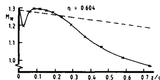
Fig.20 Calculation of Mach number normal to shock at two stations on wing
