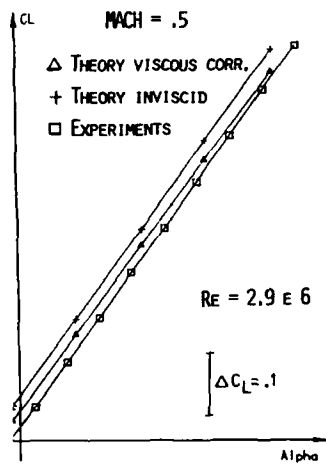
Fig. 12.a - Lift Coefficient
