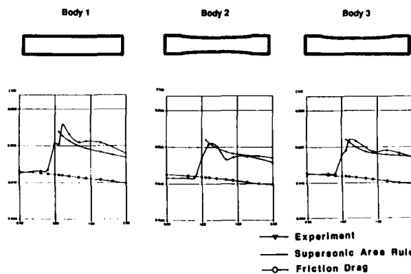
Fig. 28: Wave Drag Code Validation - Variation of Body Cross Section
