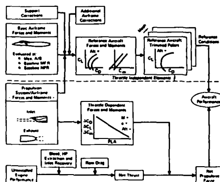
Fig. 45: Thrust/Drag Accounting System: Procedure, schematically
