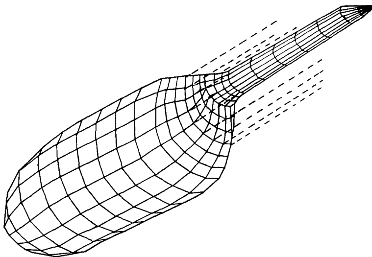
Figure 26 Helicopter Fuselage Panelization for Unsteady Flow Simulation
