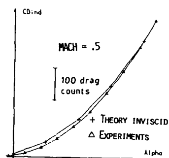
Fig. 3 - Induced Drag Coefficient
