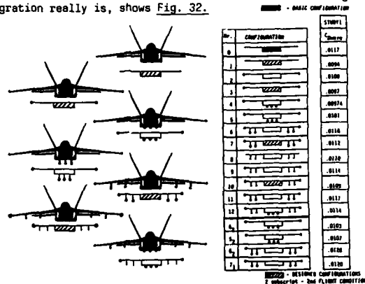
Fig. 32: Drag Optimization for Store Integration
