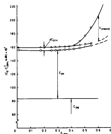
Fig.14 Analysis of drag, M = 0.78
