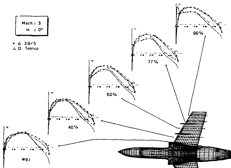
Fig. 4 - Theoretical - Experimental Pressure Distributions
