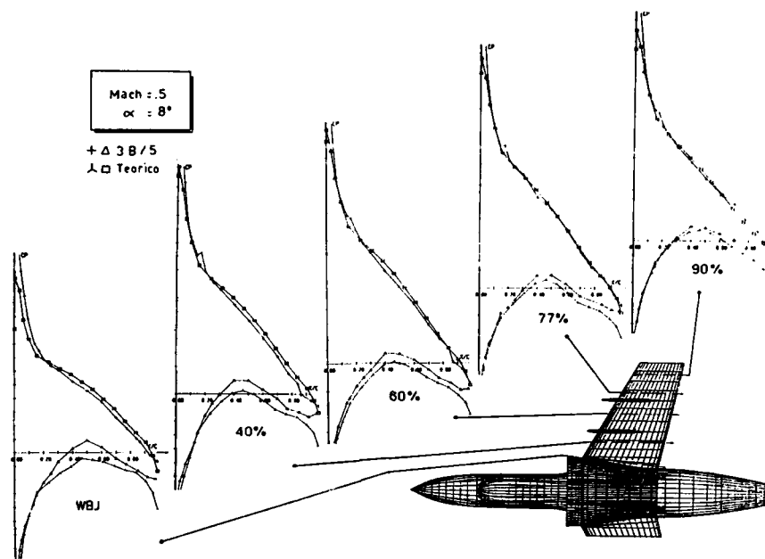
Fig. 5 - Theoretical-Experimental Pressure Distributions \alpha = 8^\circ
