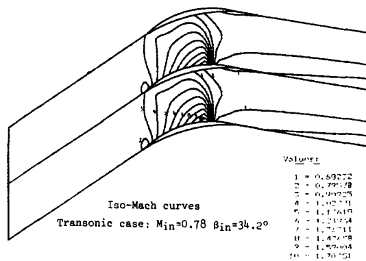
Figure 15a. Non-viscous calculation results DCA Cascade
