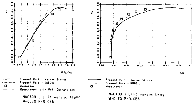
Fig. 8: Navier-Stokes Analysis for Airfoil Sections NACA 0012
