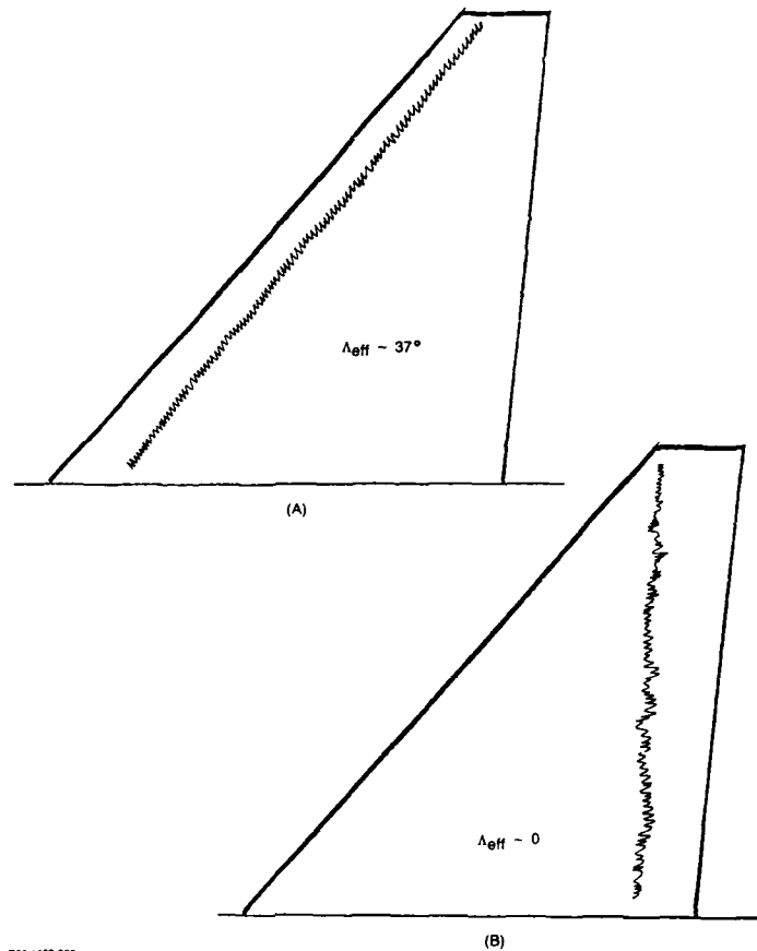
Figure 9 Fighter Planform Effective Sweep Variations
