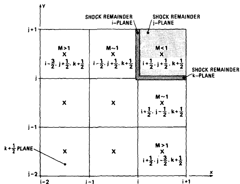
Fig. 6 Capture of shock remainders in MATRICES
