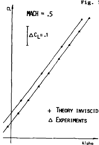
Fig. 2 - Lift Coefficient
