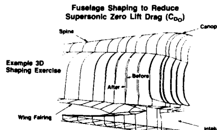
Fig 28 Full Shaping - Reduced C_{D0} by 5% Exercise Increased Volume by 400 Litres
