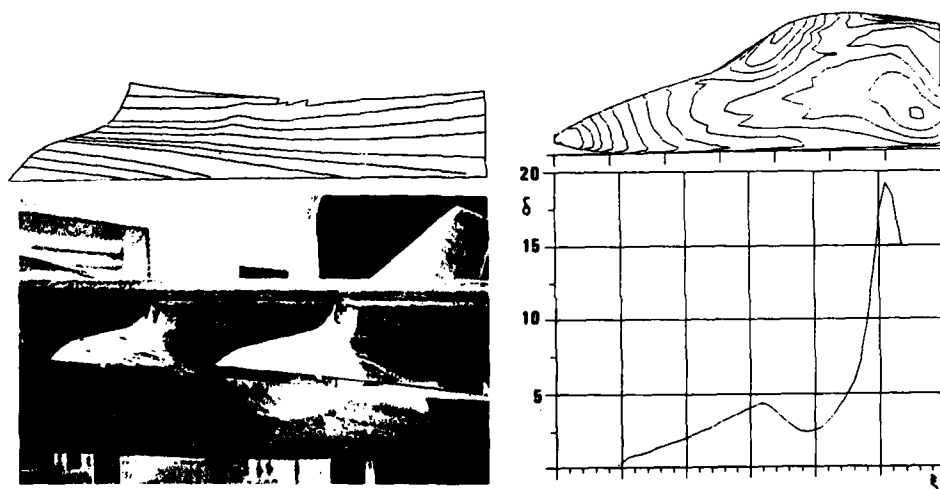
Fig. 10 - Experimental and Computed Wall Streamlines on Inboard Pylon
