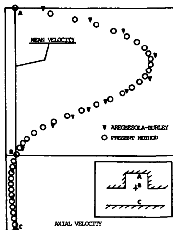
(a) velocity profile in the plane groove
