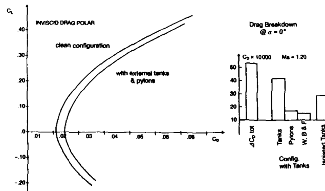
Fig. 37: Wave Drag Increment Analysis due to Store Installation
