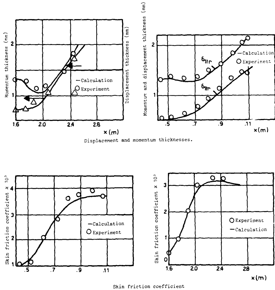
FIG. 5 Comparison between calculation and experimental results for two transitional boundary layers.
