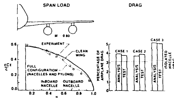
Fig. 14: Analysis of Wing Loading and Nacelle Drag
