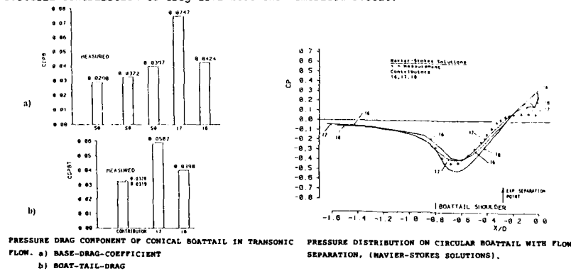
Fig. 42: AGARD WG 08: Integration of Boattail Drag
