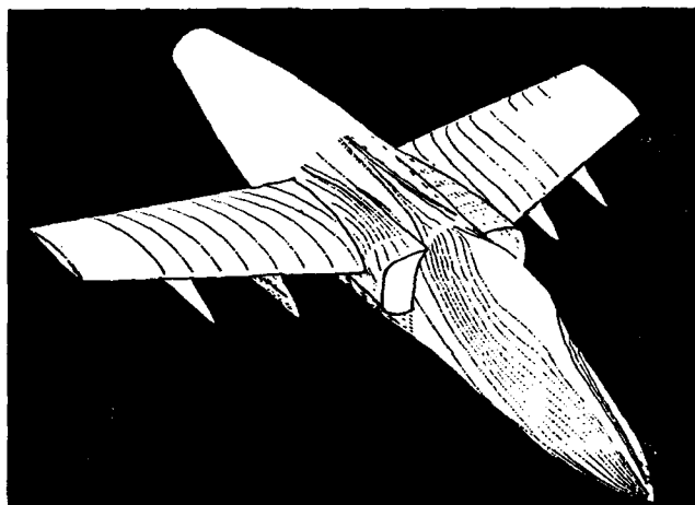
Fig. 9 - Computed Wall Streamlines
