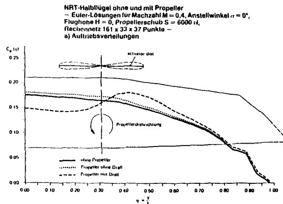
Fig. 15: Spanwise Load Distribution for Wing with Propeller
