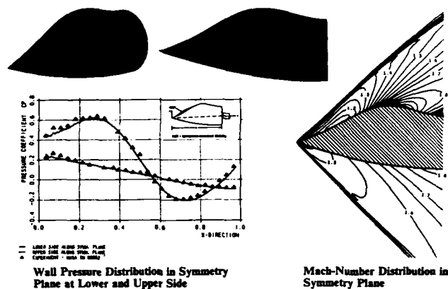
Fig. 48: Euler Space Marching for Results for NASA-Forebody 4
