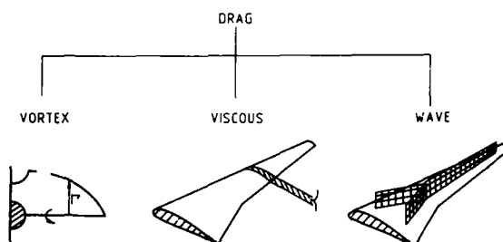
Fig.2 Far field analysis of drag of wings at subsonic speeds
