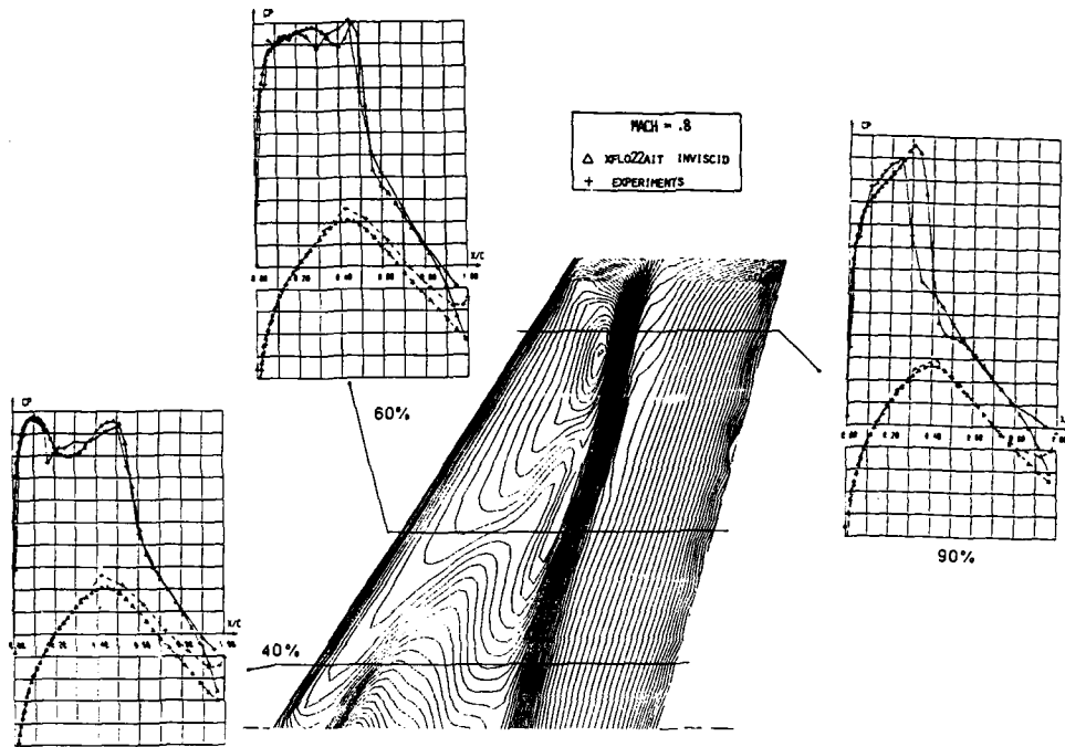
Fig. 15 - Comparison Between Transonic Wind Tunnel and Numerical Pressure Distributions. Isobars From XFL022AIT - Case \alpha=5^\circ
