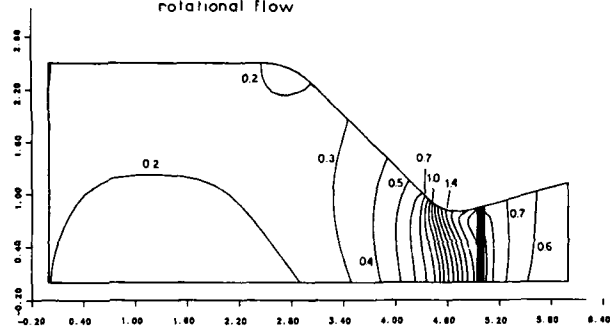
ISOMACH CONTOURS rotational flow
