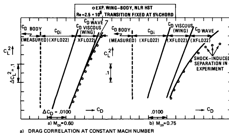
a) DRAG CORRELATION AT CONSTANT MACH NUMBER
