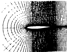
Fig. 9: 2D Navier-Stokes Solution for VA7-00-0 Airfoil
