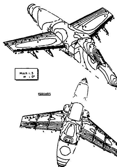
Fig. 7 - Computed Pressures
