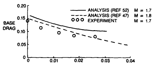
Figure 29 Effect of Mass Injection on Base Drag
