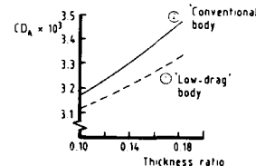
Fig 21 Pressure distributions and drag versus thickness ratio for axisymmetric bodies calculated by Myrings method
