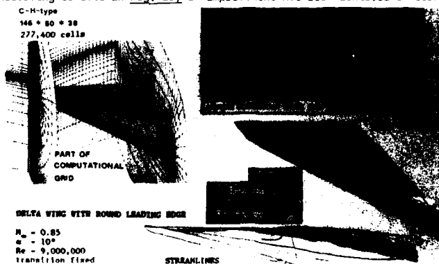
Fig. 23: Flow Field Analysis using EULER Flow Code including Leading Edge Flow Separation
