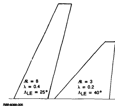
Figure 5 Transport & Fighter Wing Planforms
