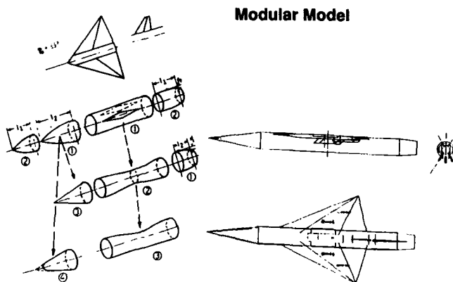
Fig. 25: Wave Drag Code Validation - Modular Model
