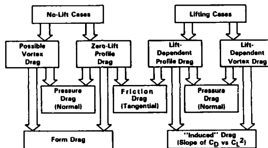
Fig. 1: Sources and Terminology of Drag Contribution
