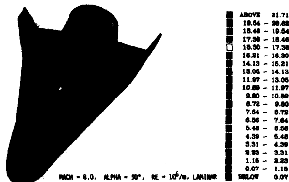
Fig. 52: HERMES Isobars as Navier-Stokes Solution
