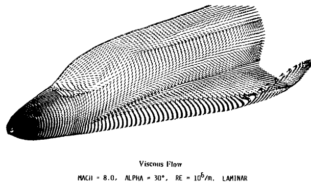
Fig. 51: Direction of Wall Stress Vector for HERMES
