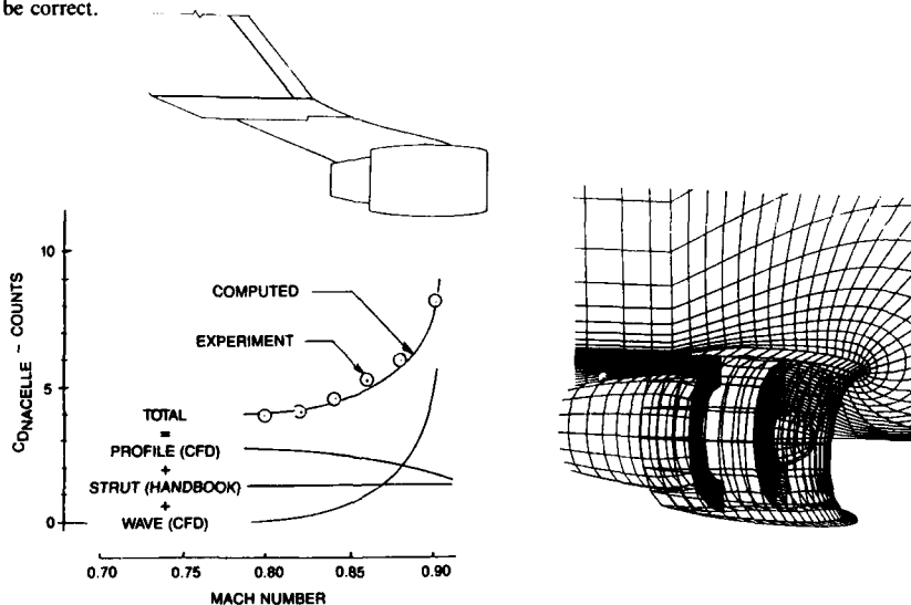
Figure 18 Nacelle Drag Correlation (Boeing-Tinoco)
