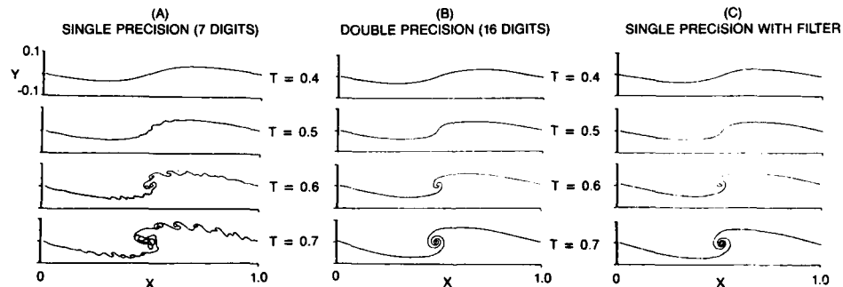
Figure 17 Vortex Sheet Stability (Krasny (33))
