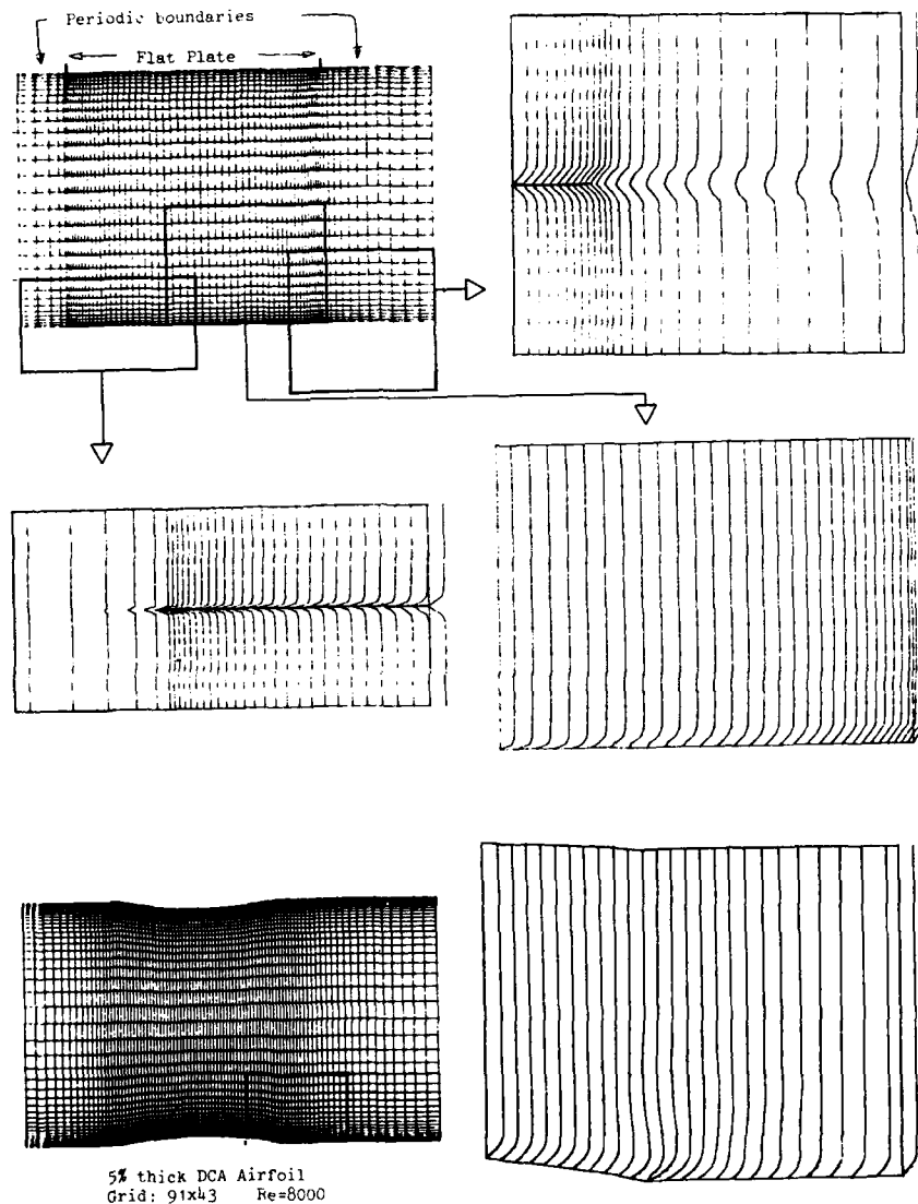
Figure 5b. Viscous laminar flow calculation results Velocity profiles
