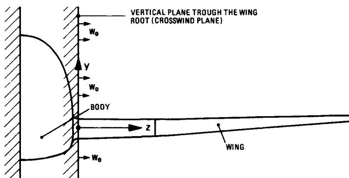
Fig. 1 The 'X-wind' concept in XFLO22
