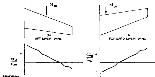
Figure 14 Forward/Aft Sweep Wing Drag Loading
