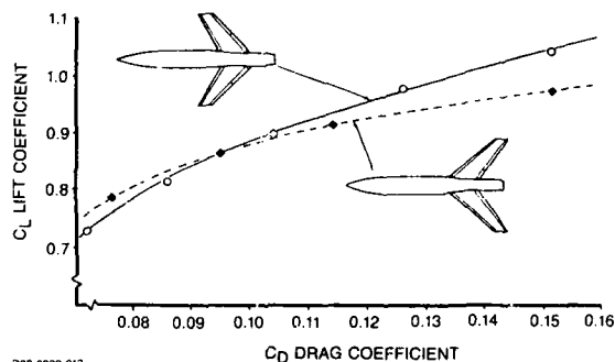
Figure 12 Forward/Aft Swept Wing Drag Comparison, AFFDL Wind Tunnel Test M_\infty = 0.9
