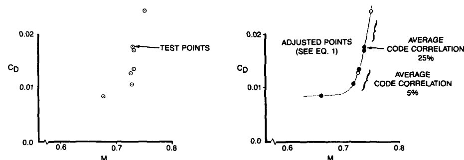
Figure 4 RAE-2822 Airfoil Drag Divergence Curve Data & Adjusted ( C_l \approx 0.74 )
