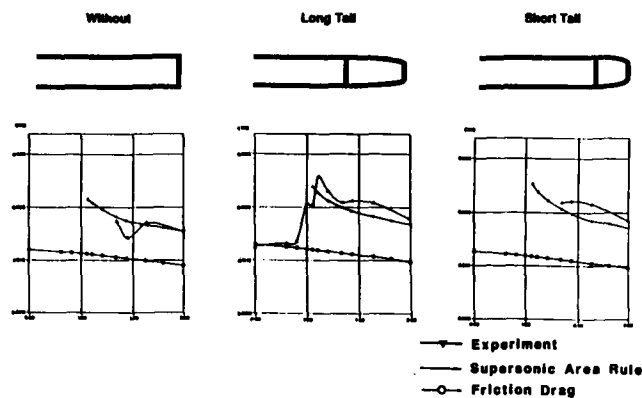
Fig. 29: Wave Drag Code Validation - Variation of Boat-Tail
