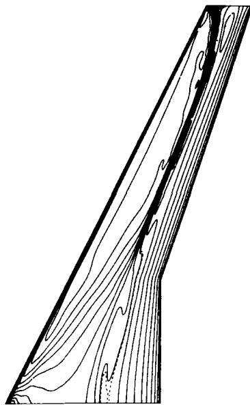
Fig. 9 Planform of the 'DFVLR-F4-wing', and upper surface isobars for the transonic condition M_\infty = .75 , \alpha = .84^\circ
