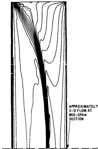
Fig. 7 Simple non-swept constant chord wing with M6 section profile (M6 test wing), showing the upper surface isobars at M_\infty = .77 , \alpha = 6^\circ
