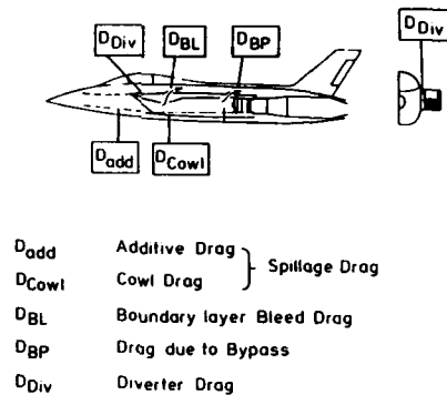
Fig. 46: Thrust/Drag Accounting System: Inlet Drag Components
