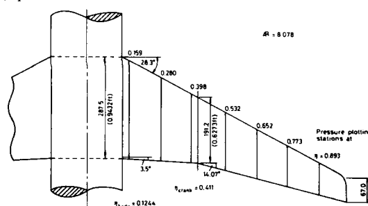
Fig.13 Planform of wing W4 showing pressure-plotting stations
