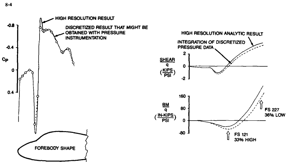
Figure 1 Effect of Pressure Distribution Discretization on Fuselage Shear & Bending Moment M = 0.7 ; \alpha = 4^\circ
