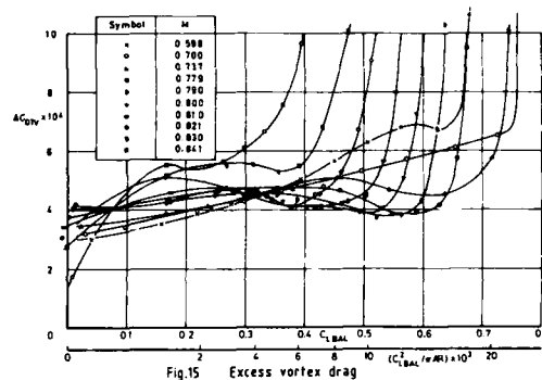
Fig.15 Excess vortex drag
