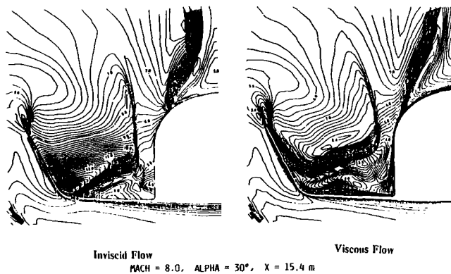
Fig. 50: Comparison of Euler/Navier-Stokes for HERMES
