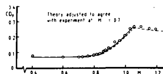
Fig 22 Pressure distributions and drag for a conical forebody with a spherical nose blunting ratio r/R = 0.3
