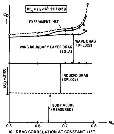
Fig. 2 NLR XFLO22 drag analyses for narrow-body transport configuration
