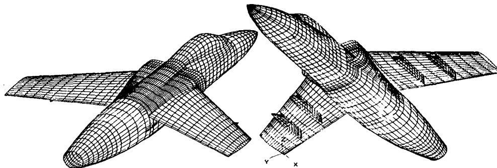
Fig. 1 - Panel Layout
