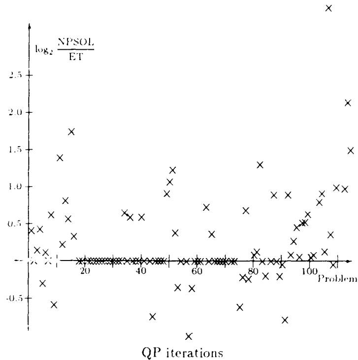
Figure 2. QP iterations: NPSOL vs. Early termination
