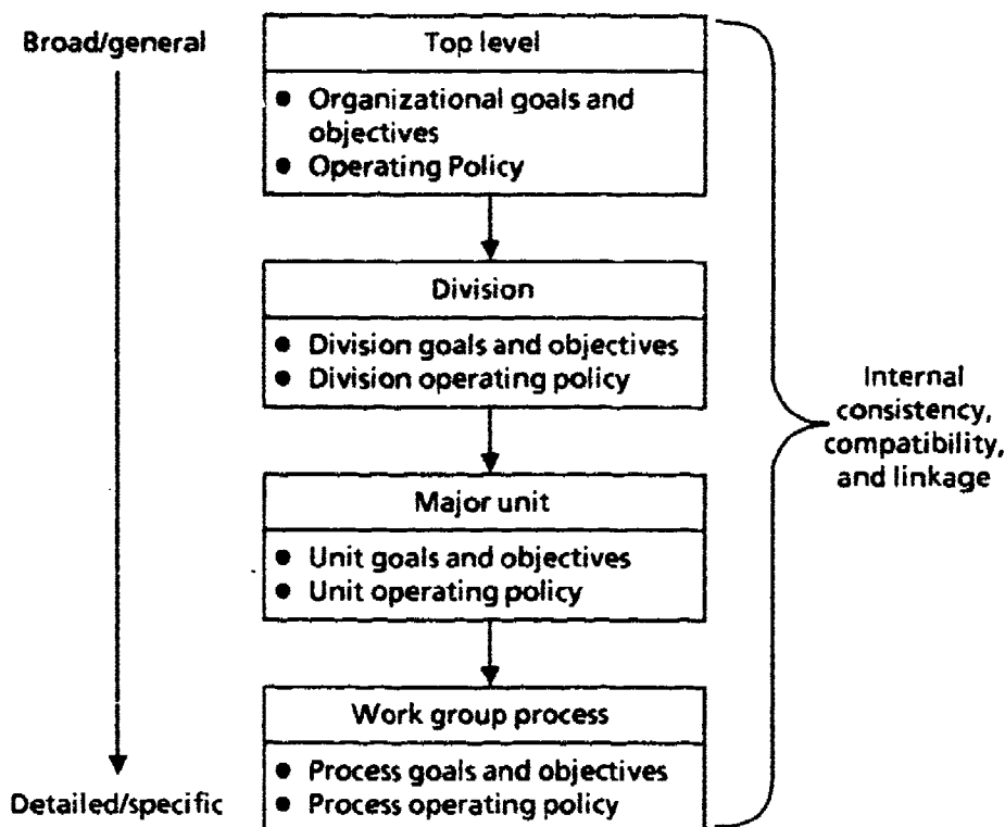
FIG. 4-1. POLICY DEPLOYMENT
