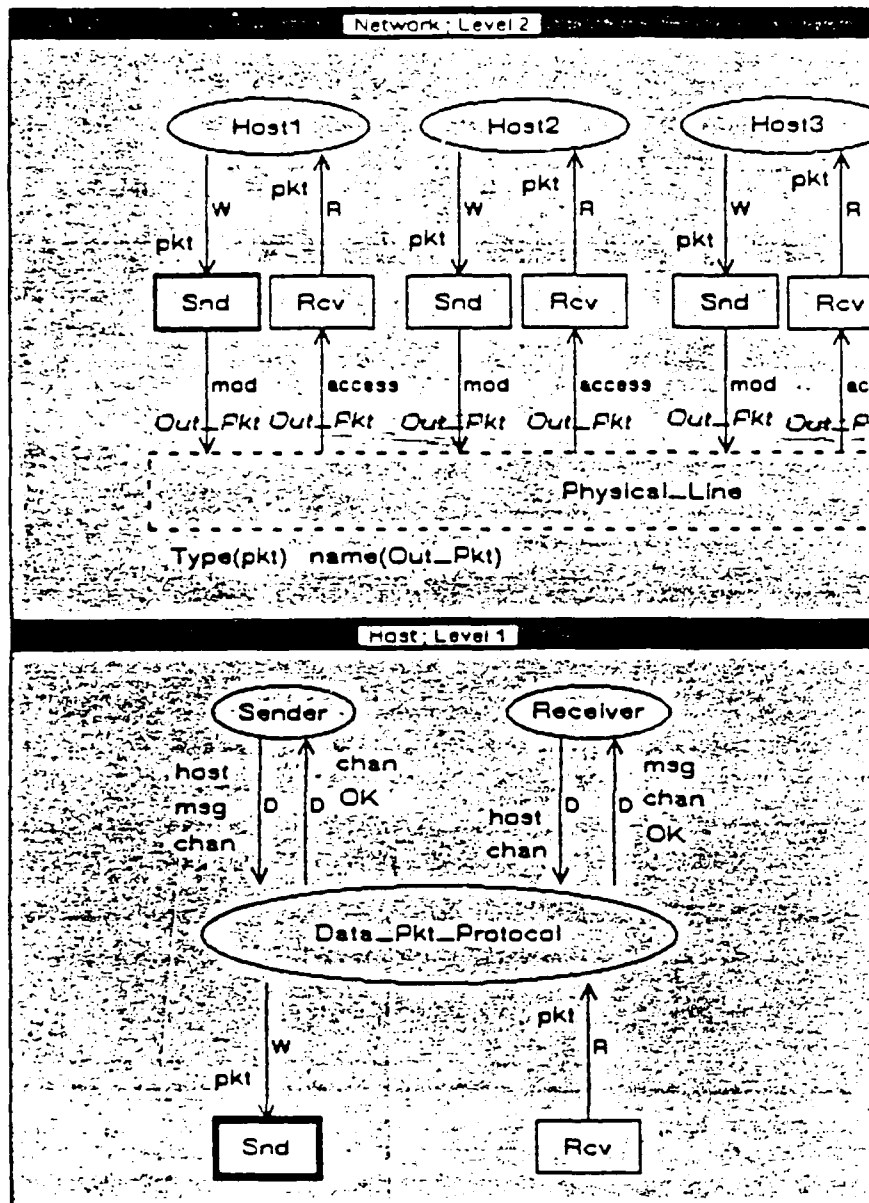
Figure 14. A design is shared through its interface entities, which are connected to another design by pointing.
