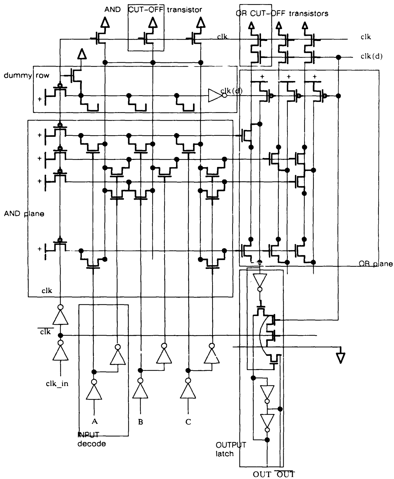
Figure 1. General schematic of the single-phase NOR/NOR PSA
