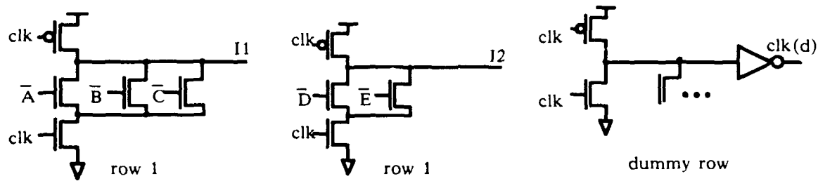
(b) AND plane
