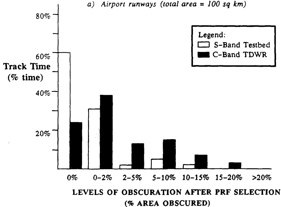
Figure A-3. Time distribution over total track time of obscuration conditions within gust front surveillance region. These represent conditions following adaptive PRF selection for runways and 360-deg circle.
