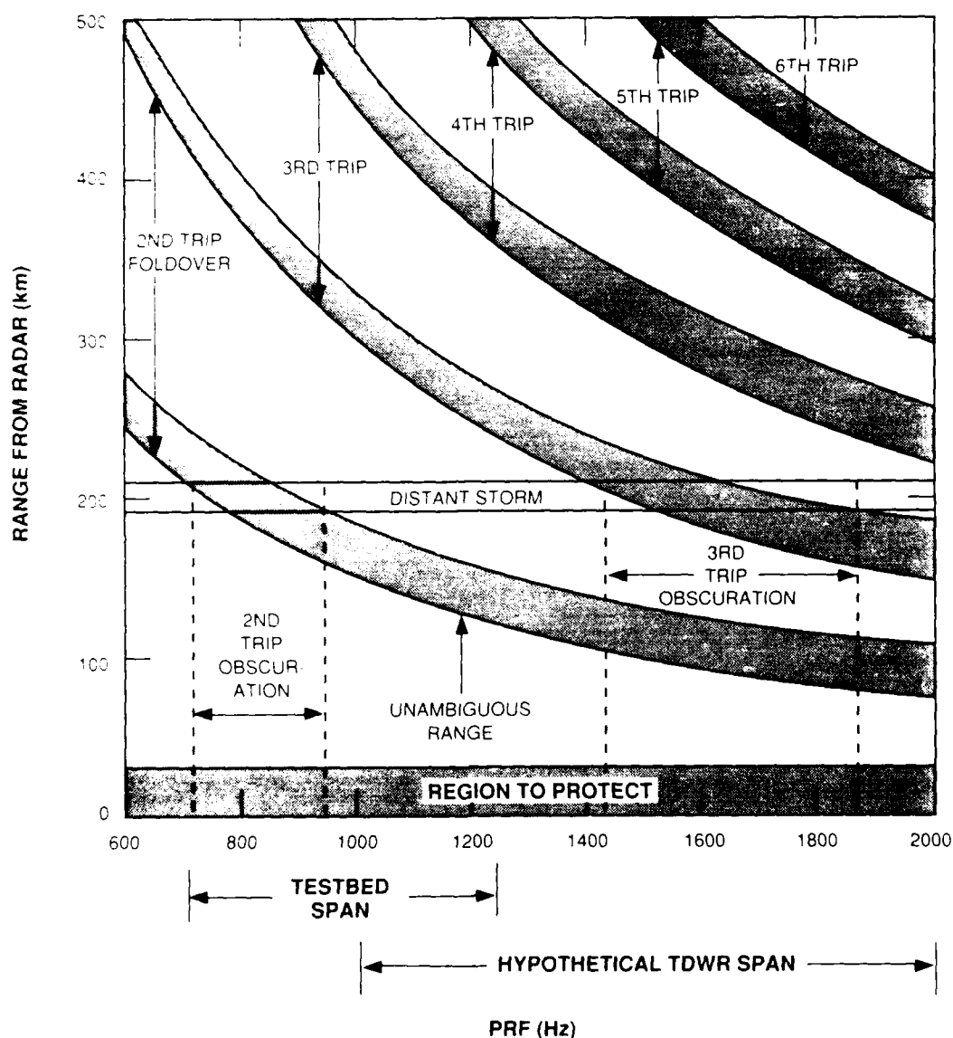
Figure 2-1. Adaptive PRF selection. The intersection of lines containing distant weather with curves defining n th trip foldover boundaries indicates which PRF values will result in range contamination to the high priority region.
