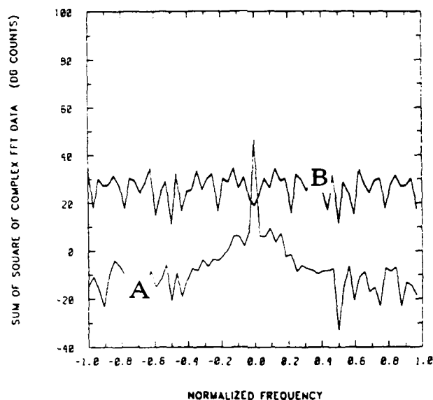
Figure 5-3. Frequency spectra of Cheyenne Ridge before and after pseudo-random phase modulation. Curve A illustrates signature of ridge before modulation; curve B illustrates signature after modulation.
