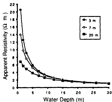
Figure 12. Model resistivity data (50-m spacing) for various water depths in cases where ice-bonded permafrost is 3-, 7- and 20-m depths beneath the seabed.
