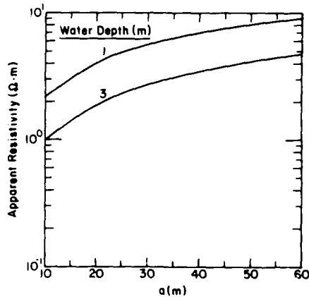
Figure 3. Model illustrating the influence of water depth on observations with a floating Wenner array for the Kittery, Maine, site. The resistivity values used were 0.25 \Omega \cdot m for seawater, 2.0 \Omega \cdot m for sand and 20.0 \Omega \cdot m for the rock. The thickness of the sand layer was 2.0 m.
