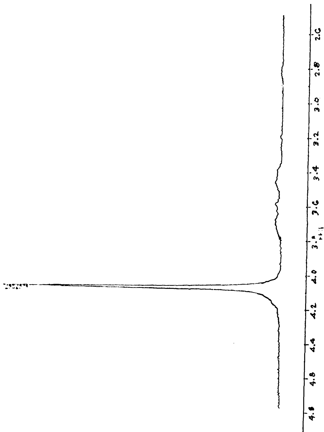
FIGURE 27. ^1\text{H} NMR OF HOMOACID AND CUBANE DIACID IN \text{D}_2\text{O} AFTER 20 H AT 60^\circ\text{C} AND 4 H AT 110^\circ\text{C}
