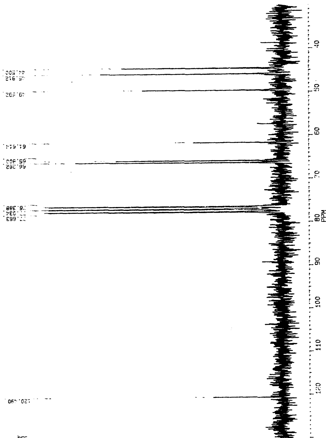
FIGURE 17. ^{13}\text{C} NMR OF CAGE BISKETAL
