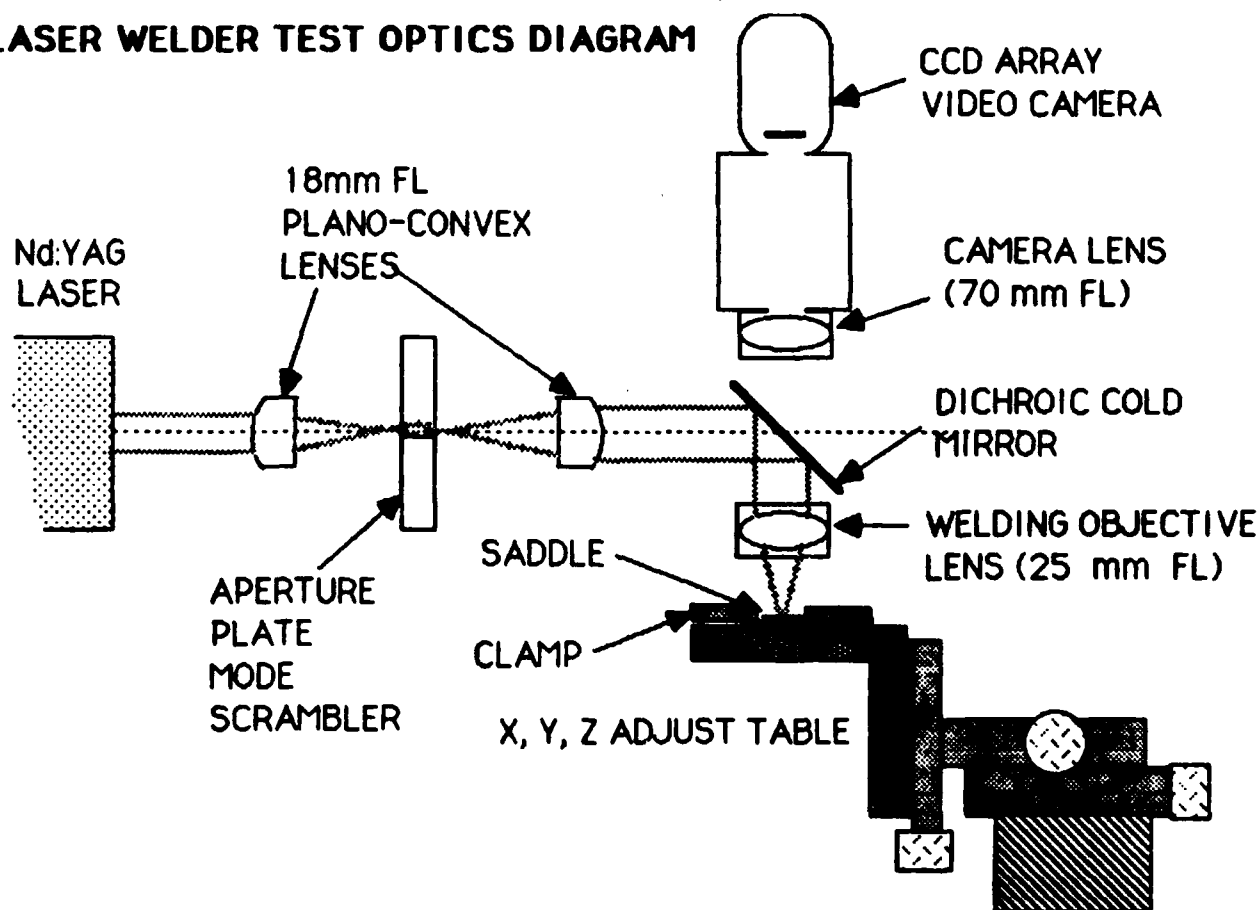
Figure 2.4.1 Experimental Imaging Optics for Welding Experiments. Light illumination to pass through to the video camera, which is used to locate the workpiece in the desired position before initiating the weld pulse. The 18 mm focal length lenses produce a small enough image of the laser mode pattern to fall within the 330 micron diameter hole in the plate, thus losing very little
