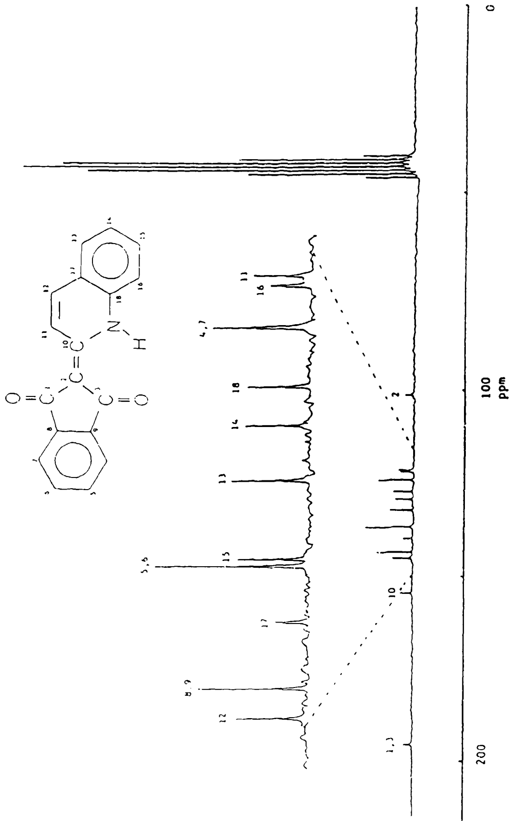
Figure 10. Carbon-13 NMR Spectrum of Dye Standard Solvent Yellow 33 (QID) in d 6 -DMSO at 80°C (See Table 1g for chemical shift assignments.)
