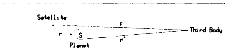
Figure 1. Geometry for Third-Body Perturbations
