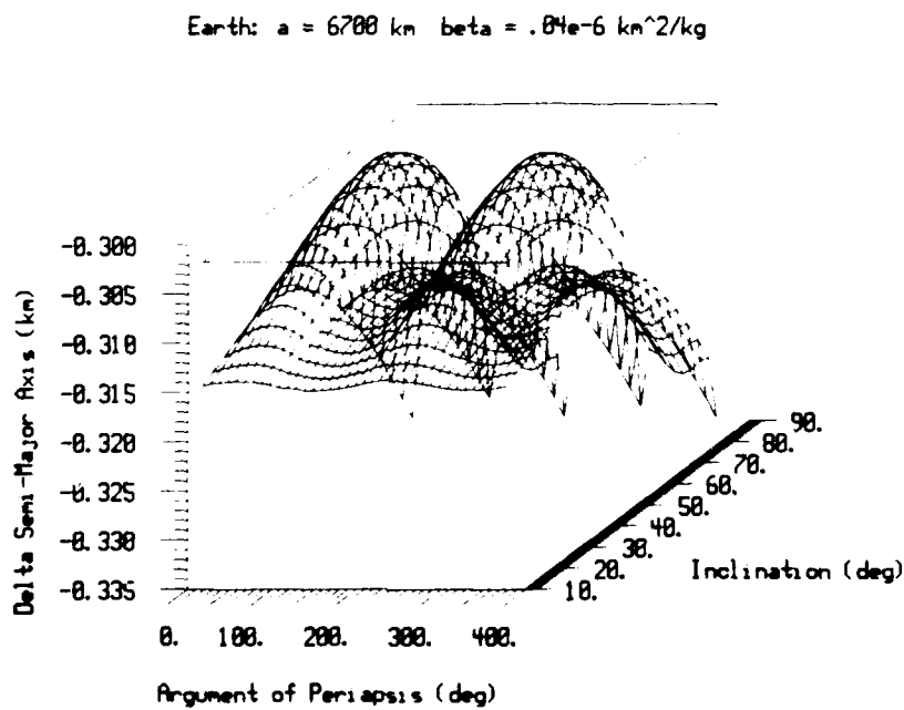
Figure D-2. Earth( a=6700\text{km} , \beta=.04\text{e-6 km}^2/\text{kg} ): Semi-major Axis Change
