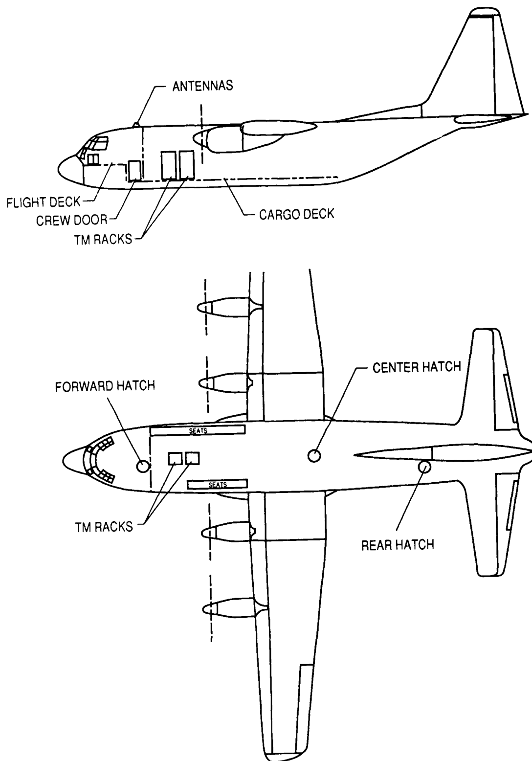
Figure 3. Aircraft Layout
