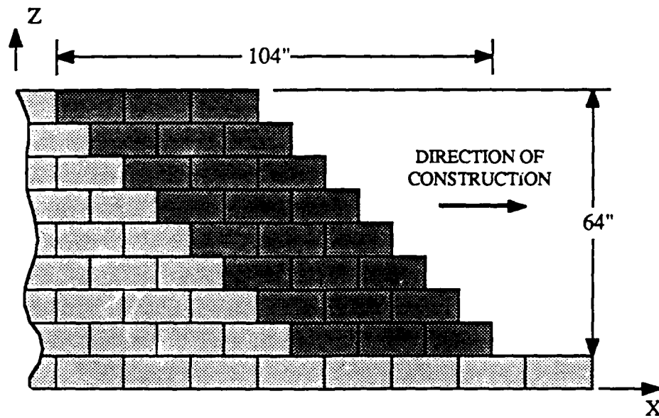
Figure 3.1.2 Staircase wall construction method
