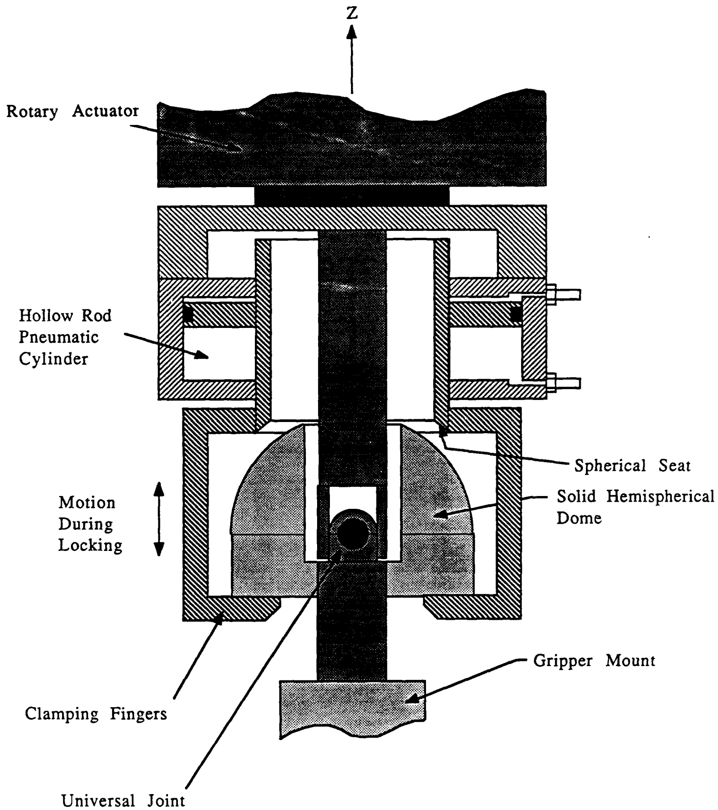
Figure 3.3.12 Lockable Universal Joint
