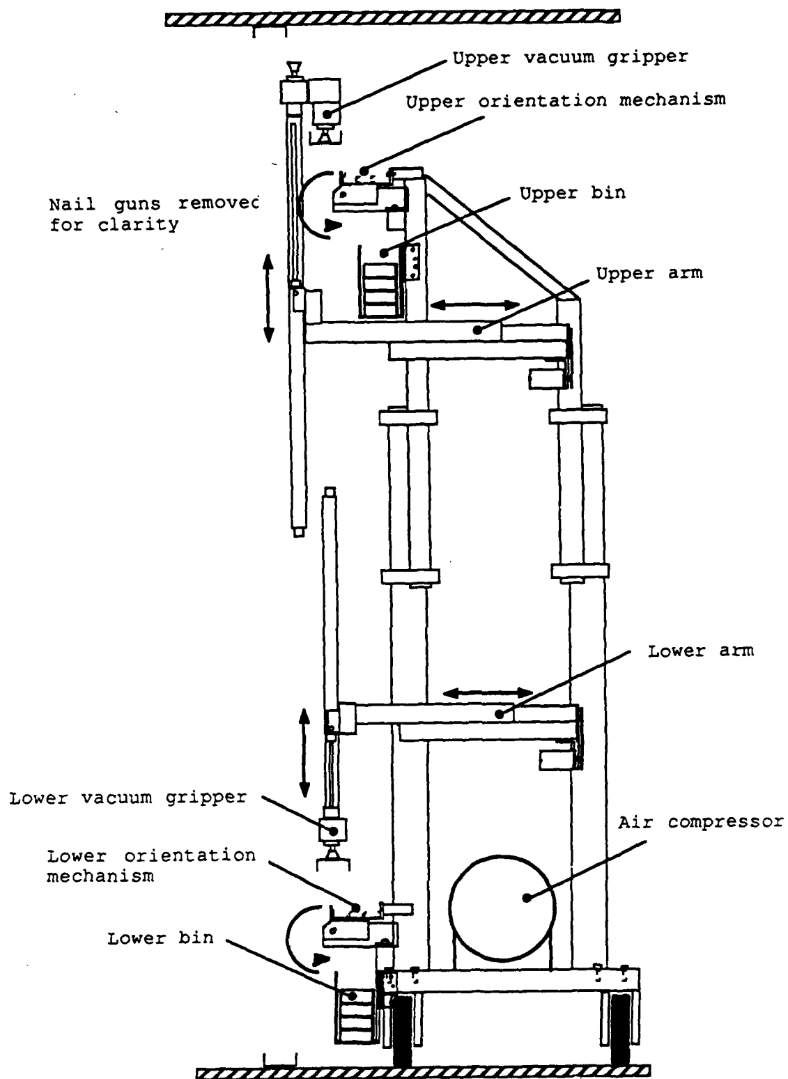
Figure 2.3.1 Trackbot schematic rear view
