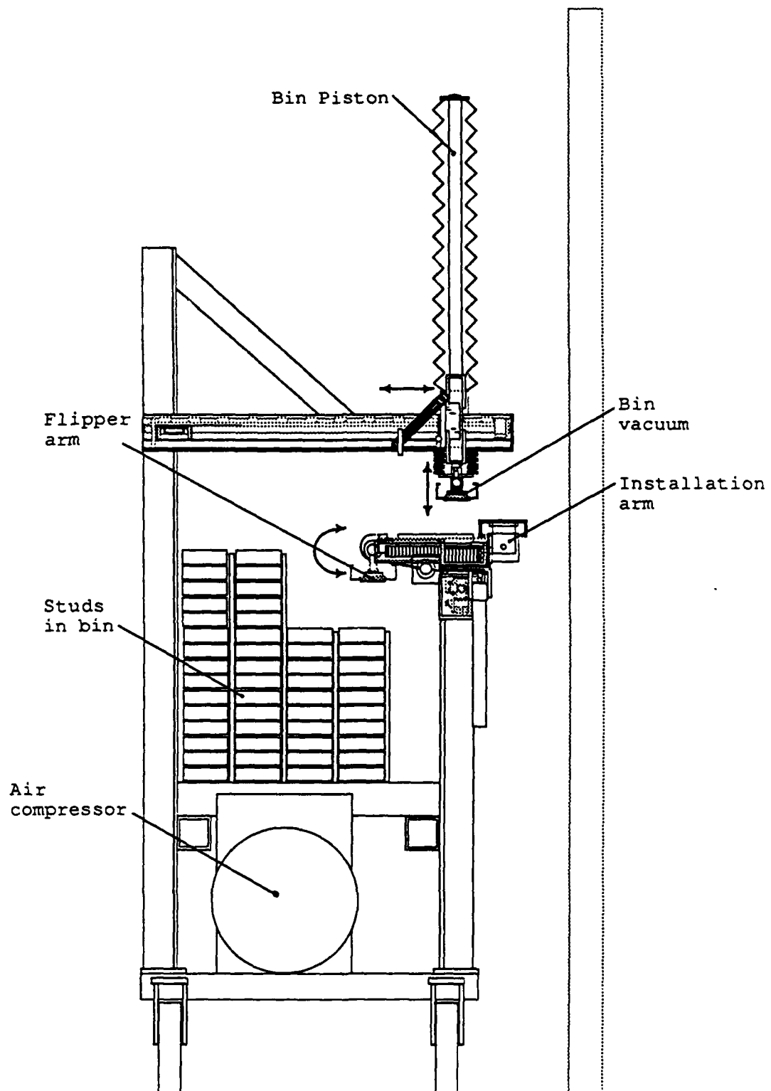
Figure 2.3.4. Studbot schematic rear view.
