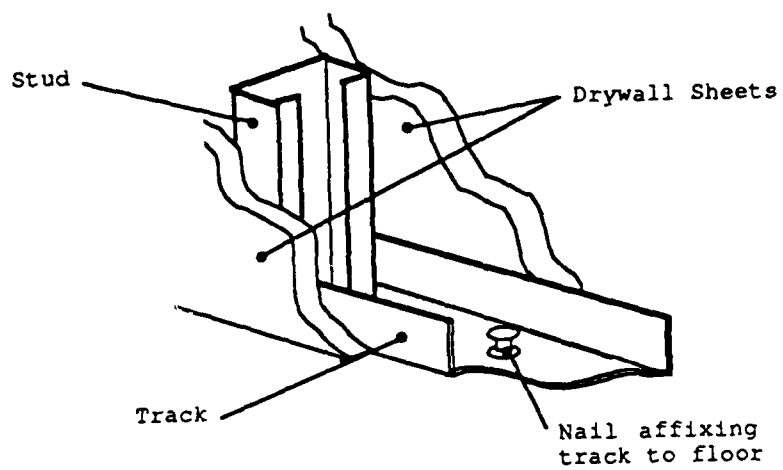
Figure 2.1.1 Cut-away view of wall.
