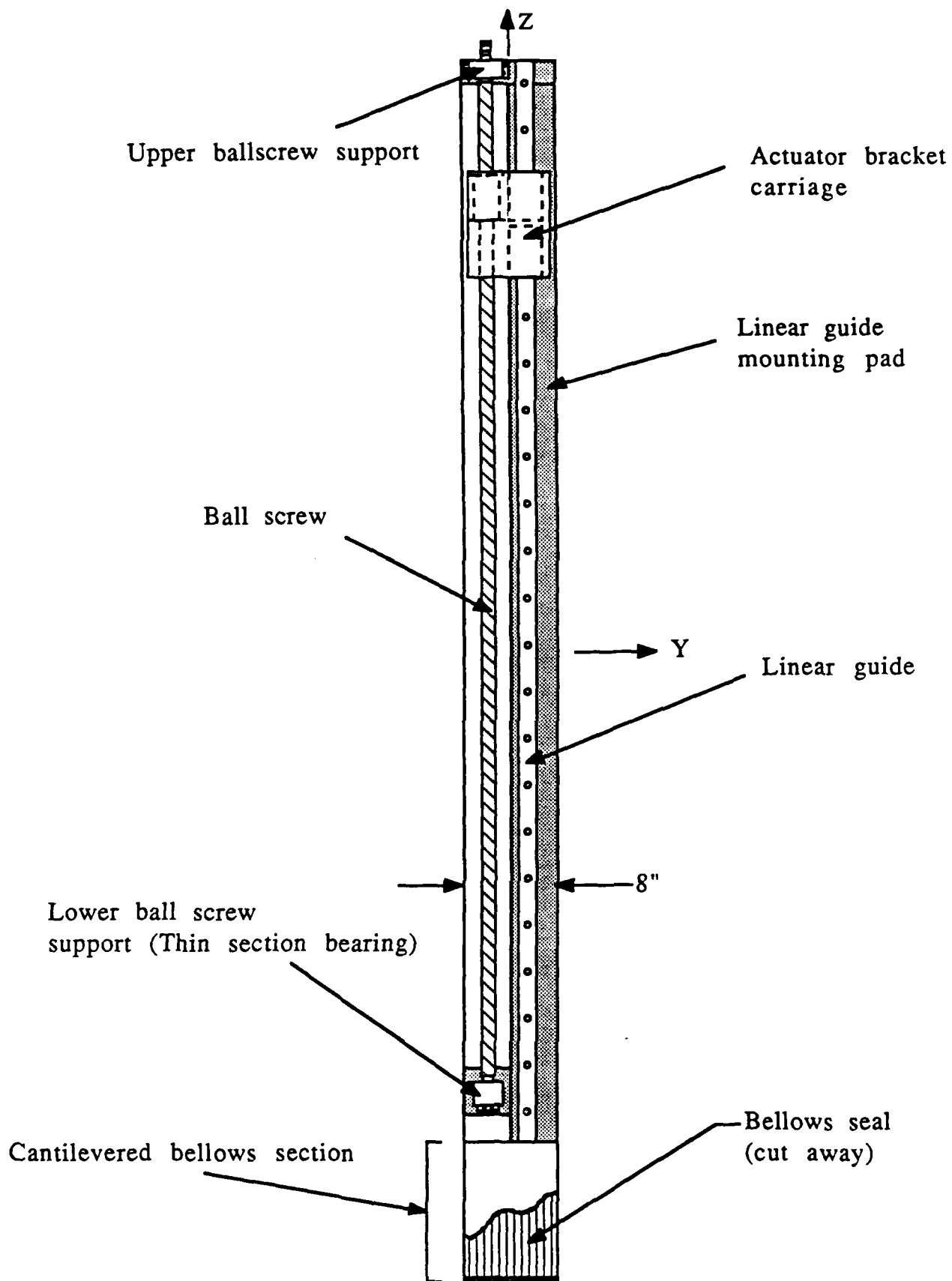
Figure 3.4.4 Front view of Z-axis assembly
