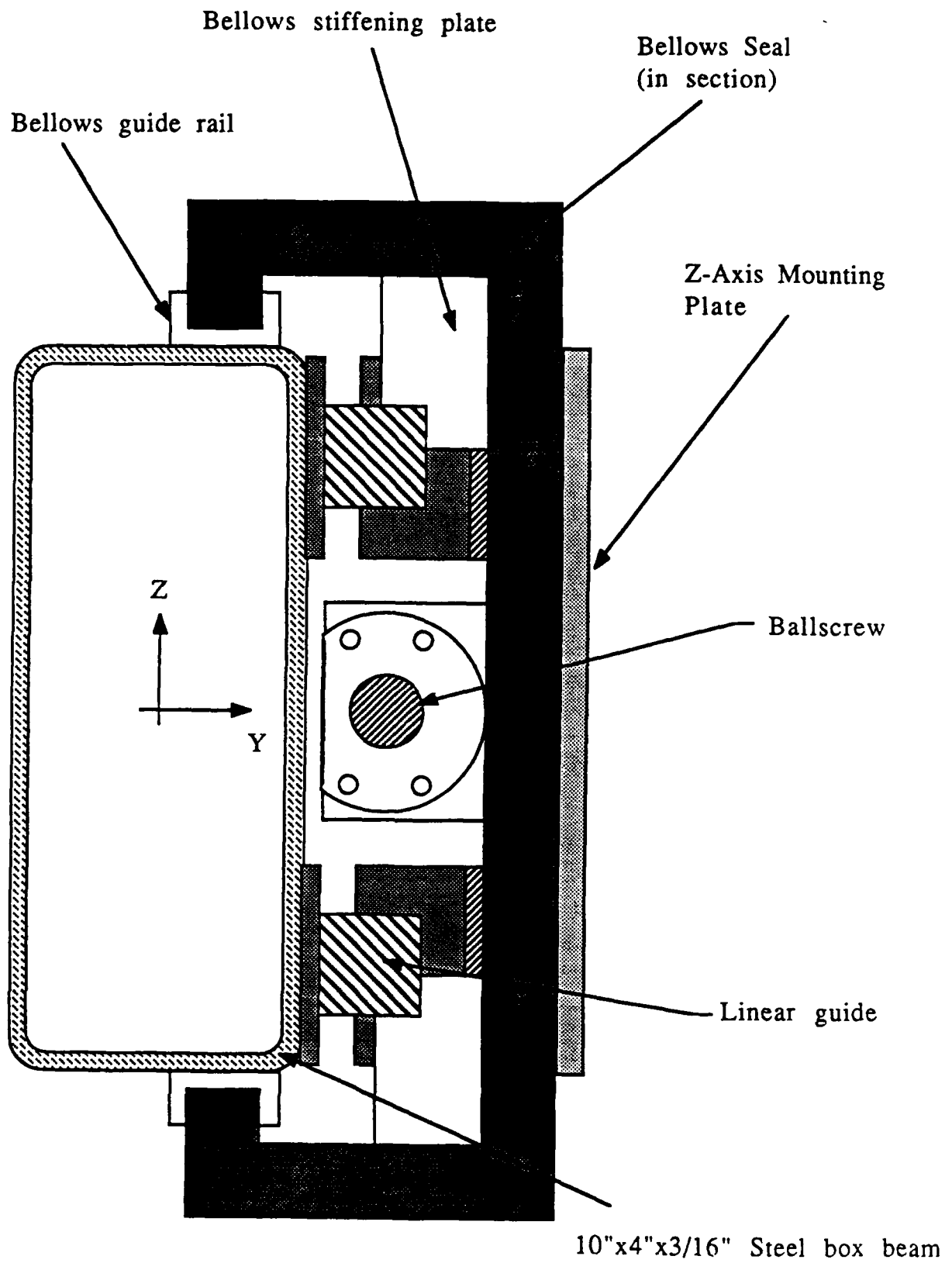
Figure 3.4.5 X-axis cross-section
