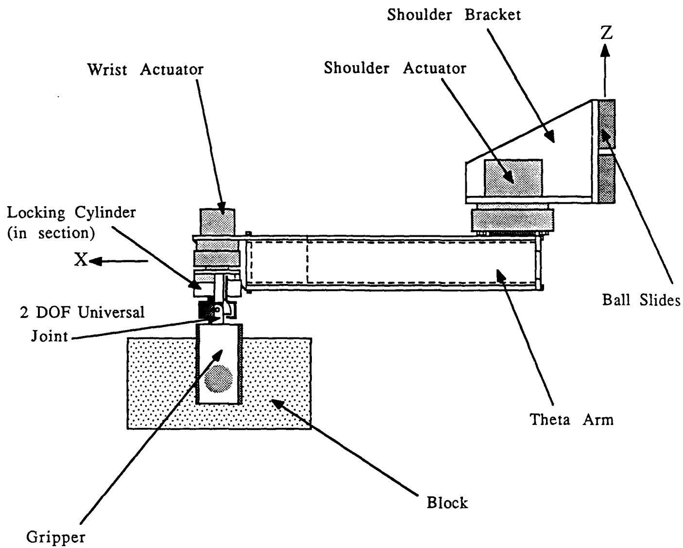
Figure 3.4.1: Theta Arm Configuration
