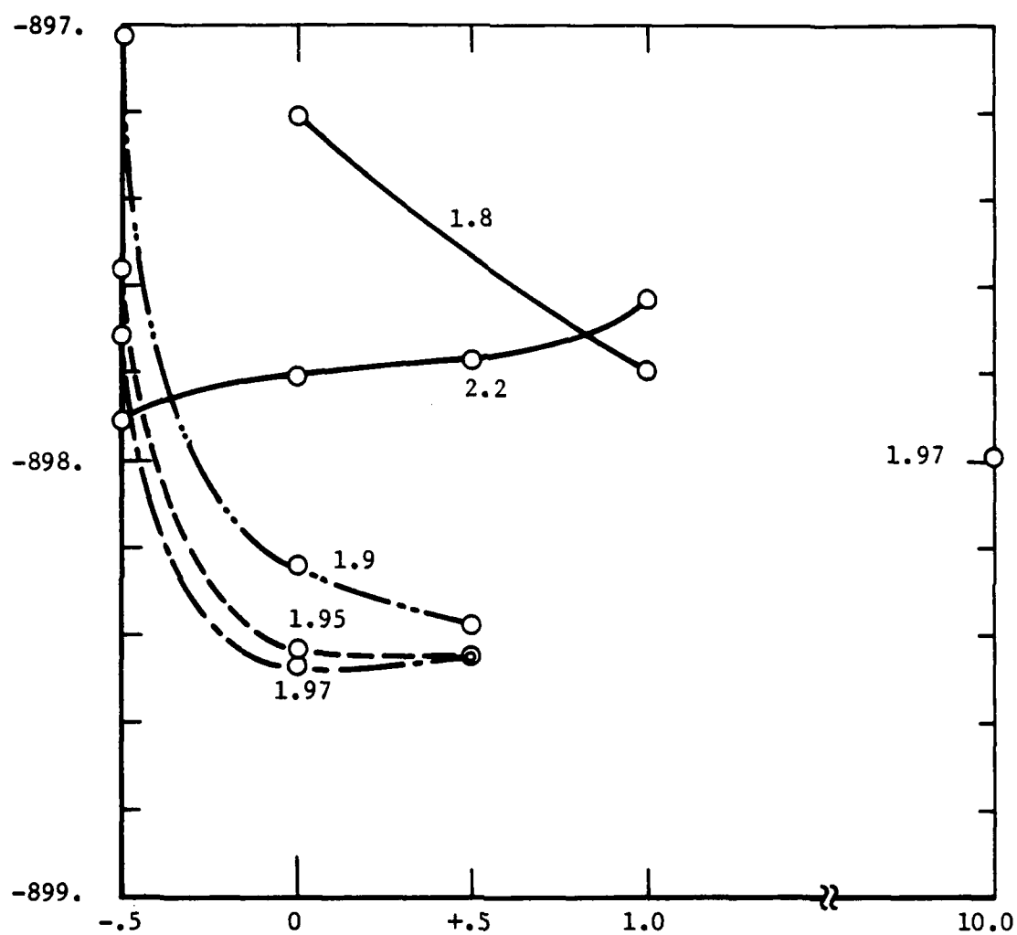
Figure 1. Surface Atom Equilibrium Position as a Function of the Nickel s-Orbital Exponent.
