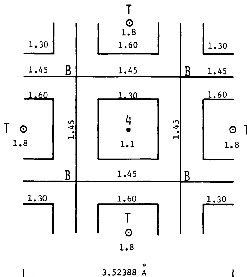
Figure 5. z-Coordinate Values for C Atom as a Function of x- and y-Coordinates Relative to Surface Nickel Sites.
