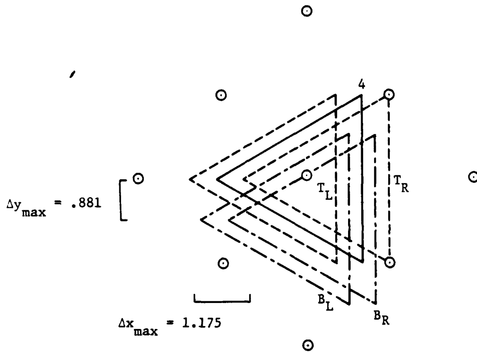
Figure 4. x- and y-Coordinates of High (60%) Coverage Model Calculations.
