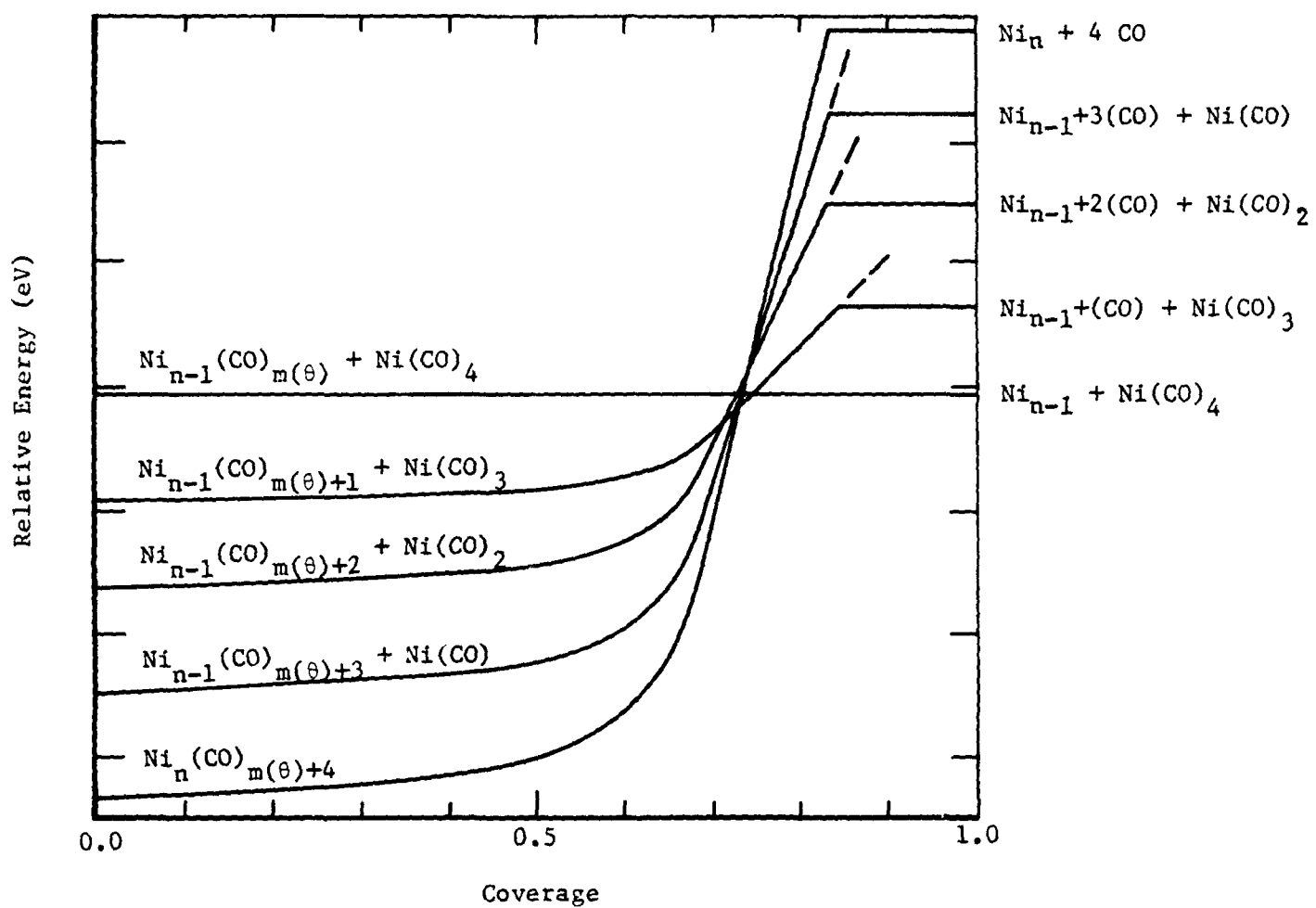
Figure 6. Relative Energetics of Competing Processes as a Function of Coverage.
