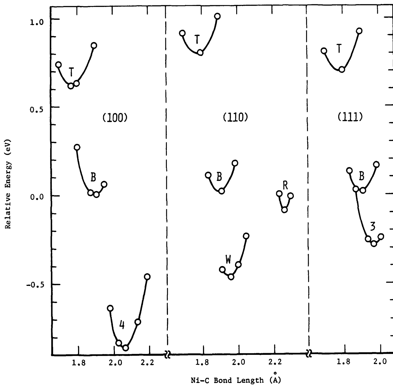
Figure 2. CO Adsorption Equilibria at Low Coverage.
