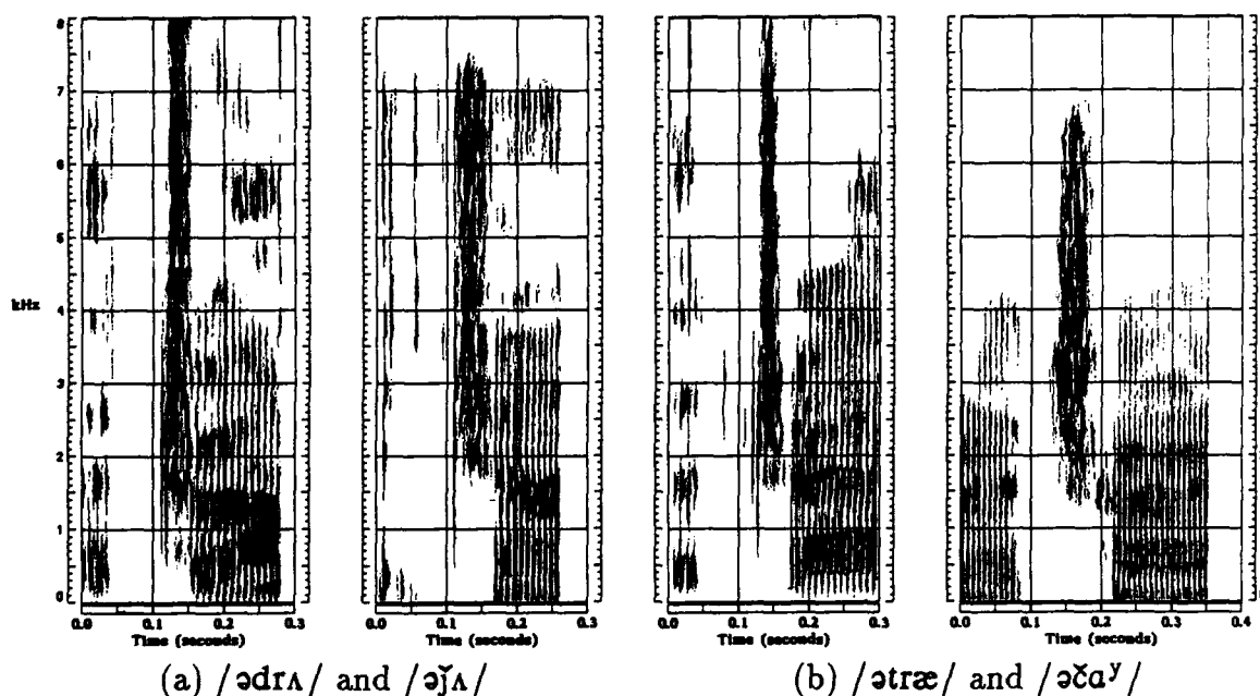
Figure 3.9: Spectrograms of (a) /ədɾʌ/ and /əjʌ/ and (b) /ətræ/ and /əɟaʏ/.
