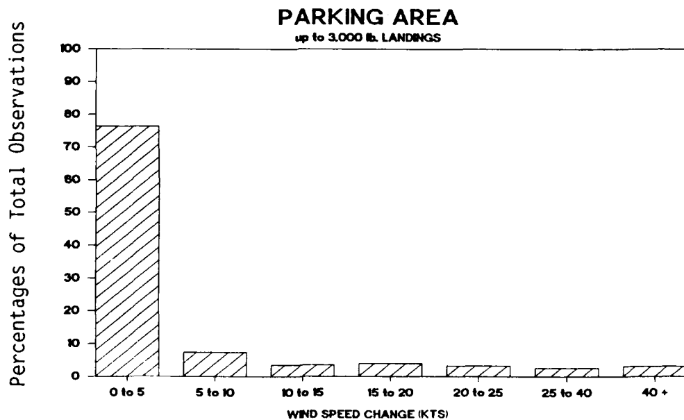
FIGURE 12. HISTOGRAMS OF WIND VELOCITY CHANGES FOR THE INDIANAPOLIS DOWNTOWN HELIPORT APPROACHES (SHEET 1 OF 3)
