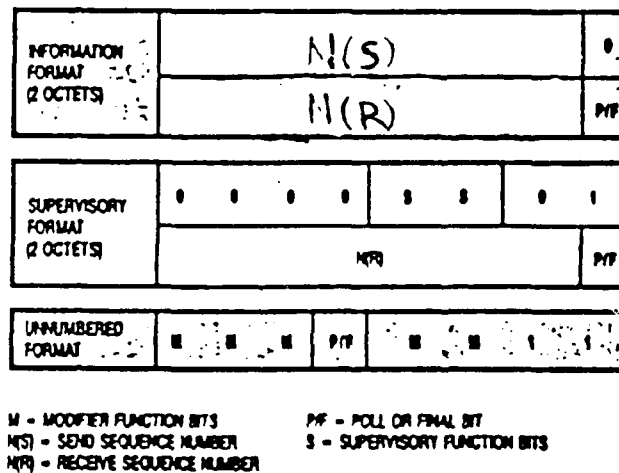
Fig. 5.14. The Control Field of ISDN LAPD
