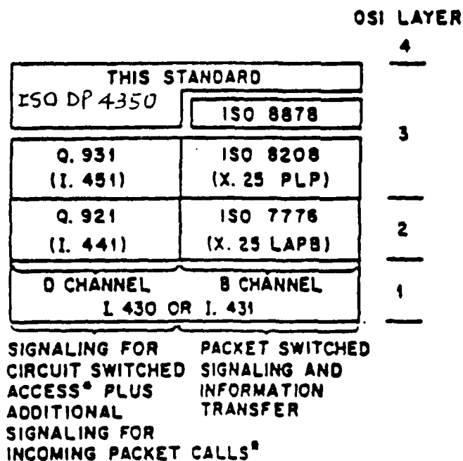
Fig. 5.21. The Protocol Layers at S and T Reference Points When B Channel Is Used in ISDN
