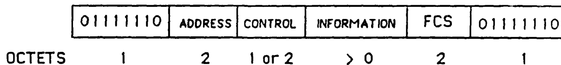
Fig. 6.11 Frame structure of the LAP-D protocol.
