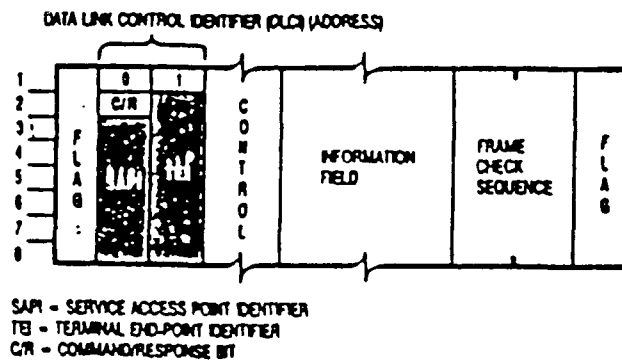
Fig. 5.13. Several Components of ISDN LAPD Frame
