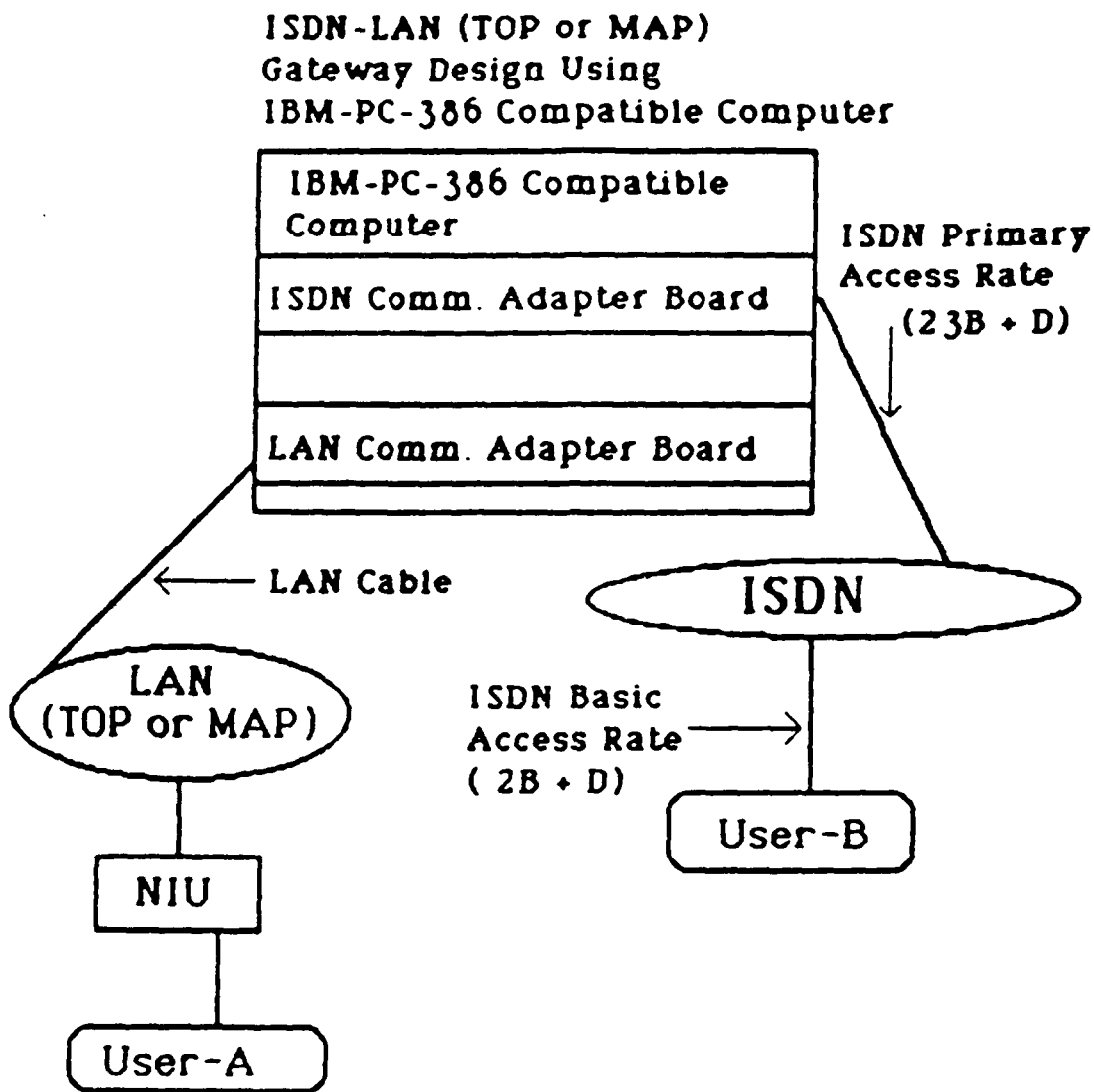
Fig. 5.37. The Scenario of ISDN-LAN (TOP or MAP) Gateway Design Using IBM-PC-386 Compatible Computer
