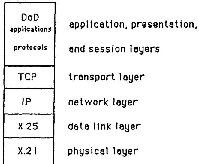
Fig. 6.3 DDN protocol structure implementing X.25
