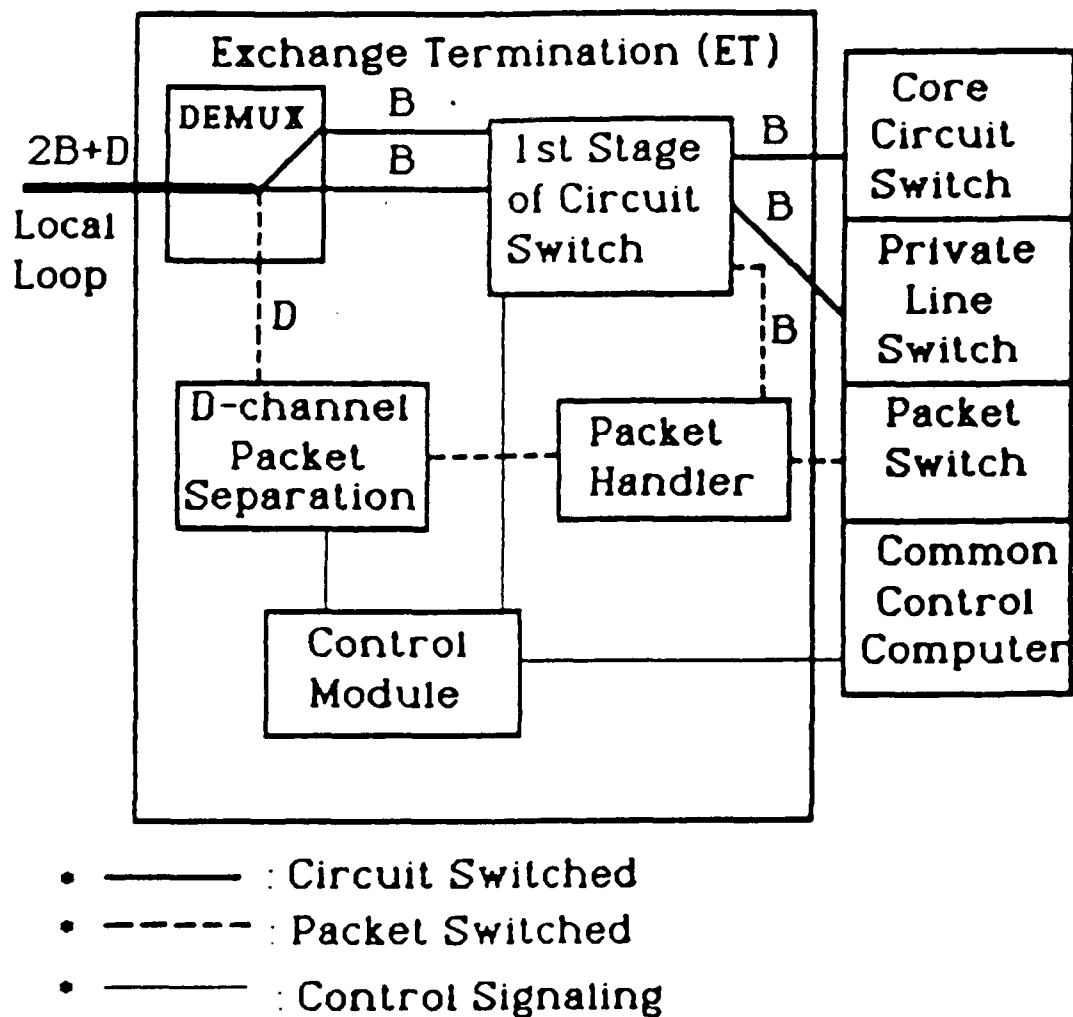
Fig. 5.8. The Exchange Termination (ET) Functional Elements of ISDN to Separate and Use B Channels and D Channel
